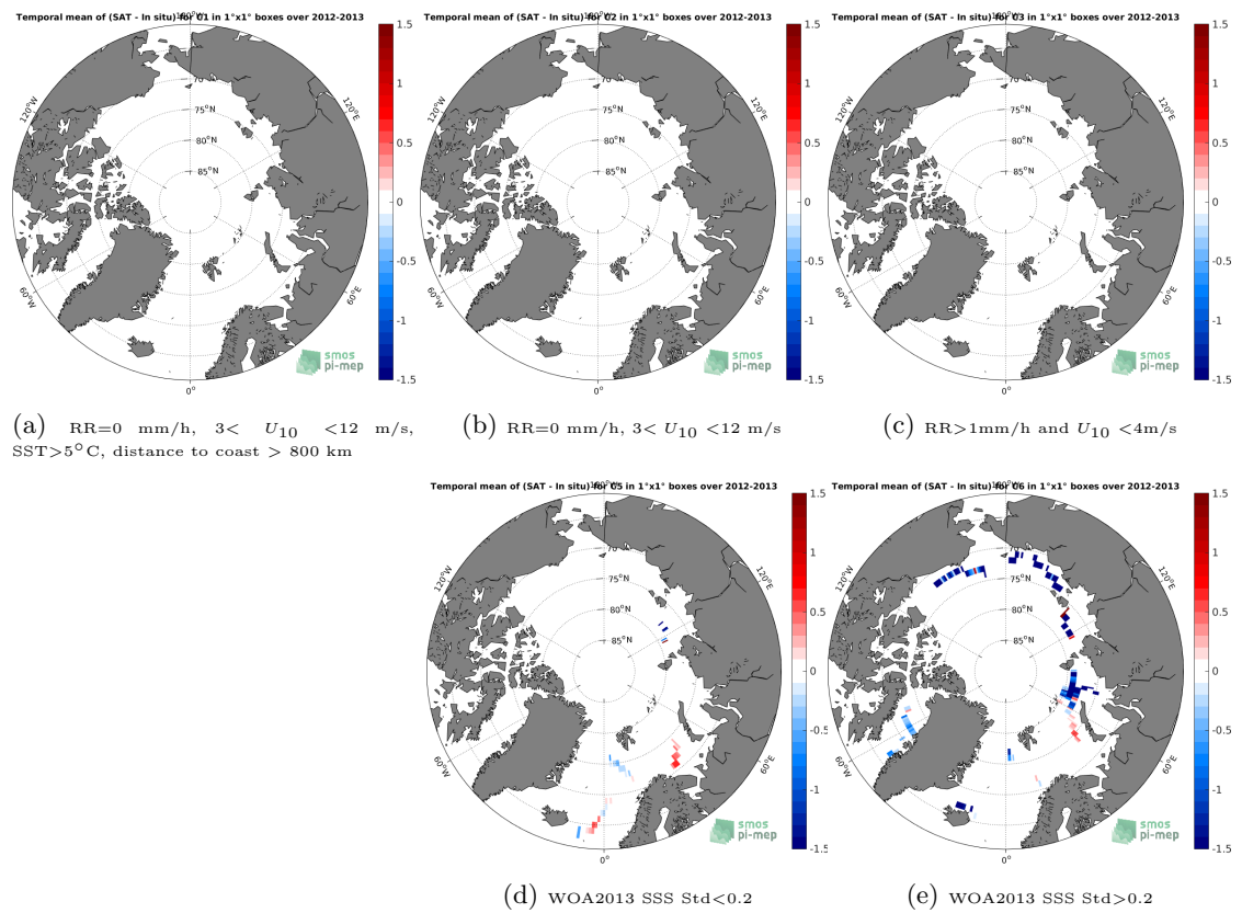
Figure 12: Temporal mean gridded over spatial boxes of size 1^\circ \times 1^\circ of \Delta SSS (Aquarius-L3-OR-V5-7DAY-RUNNING-1DEG - TSG-GOSUD-Sailing-ship) for 5 different subdatasets corresponding to:RR=0 mm/h, 3 < U_{10} < 12 m/s, SST > 5^\circ\text{C} , distance to coast > 800 km (a), RR=0 mm/h, 3 < U_{10} < 12 m/s (b), RR > 1 mm/h and U_{10} < 4 m/s (c), WOA2013 SSS Std < 0.2 (d), WOA2013 SSS Std > 0.2 (e).
