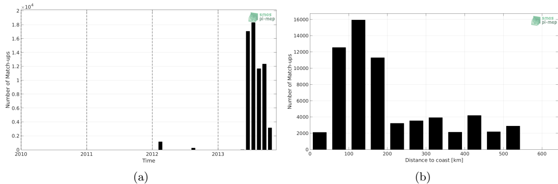
Figure 1: Number of match-ups between TSG-GOSUD-Sailing-ship and Aquarius-L3-OR-V5-7DAY-RUNNING-1DEG SSS as a function of time (a) and as function of the distance to coast (b) over the Arctic Ocean Pi-MEP region and for the full satellite product period.
