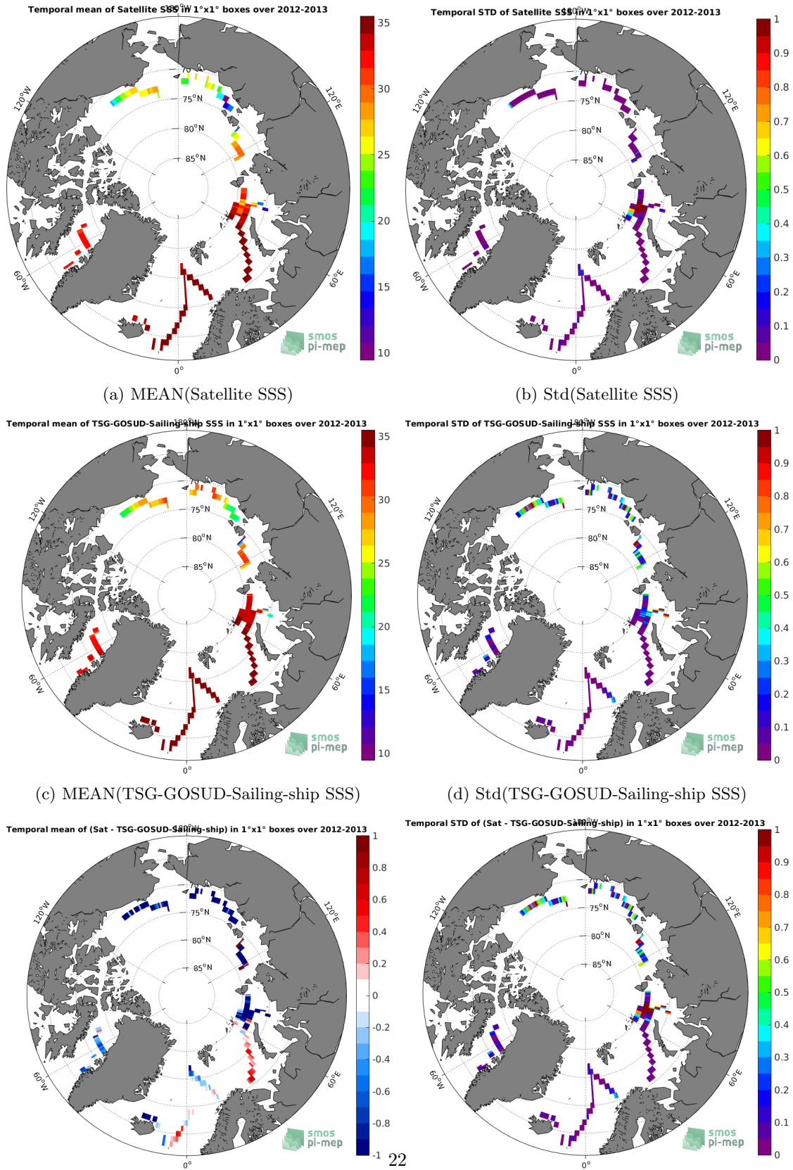
Figure 6: Temporal mean (left) and Std (right) of SSS from Aquarius-L3-OR-V5-7DAY-RUNNING-1DEG (top), TSG-GOSUD-Sailing-ship (middle), and of \Delta SSS (Satellite - TSG-GOSUD-Sailing-ship). Only match-up pairs are used to generate these maps.
