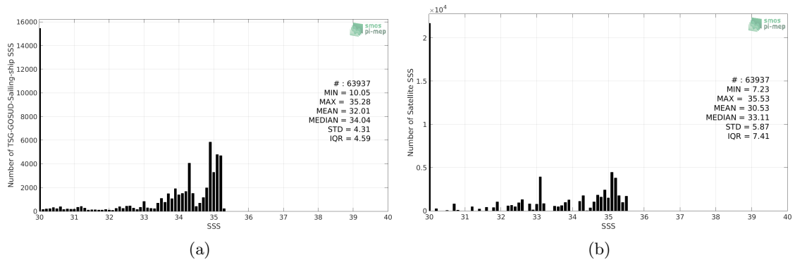
Figure 2: Histograms of SSS from TSG-GOSUD-Sailing-ship (a) and Aquarius-L3-OR-V5-7DAY-RUNNING-1DEG (b) considering all match-up pairs per bins of 0.1 over the Arctic Ocean Pi-MEP region and for the full satellite product period.
