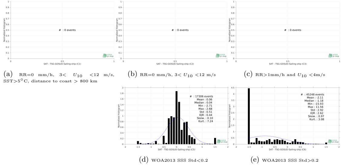
Figure 13: Normalized histogram of \Delta SSS (Aquarius-L3-OR-V5-7DAY-RUNNING-1DEG - TSG-GOSUD-Sailing-ship) for 5 different subdatasets corresponding to: RR=0 mm/h, 3 < U_{10} < 12 m/s, SST >5^{\circ} C, distance to coast > 800 km (a), RR=0 mm/h, 3 < U_{10} < 12 m/s (b), RR >1 mm/h and U_{10} < 4 m/s (c), WOA2013 SSS Std <0.2 (d), WOA2013 SSS Std >0.2 (e).
