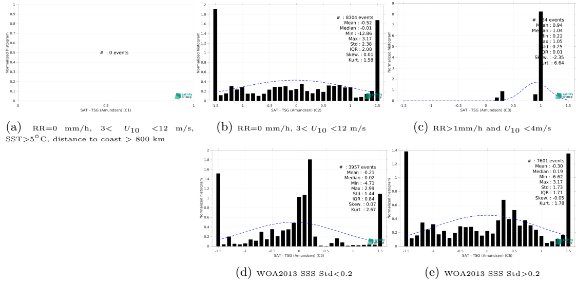
Figure 15: Normalized histogram of \Delta SSS (Aquarius SSS L3 OR v5 - 7-Day running (NASA-GSFC) - TSG (Amundsen)) for 5 different subdatasets corresponding to: RR=0 mm/h, 3 < U_{10} < 12 m/s, SST>5°C, distance to coast > 800 km (a), RR=0 mm/h, 3 < U_{10} < 12 m/s (b), RR>1mm/h and U_{10} < 4 m/s (c), WOA2013 SSS Std<0.2 (d), WOA2013 SSS Std>0.2 (e).
