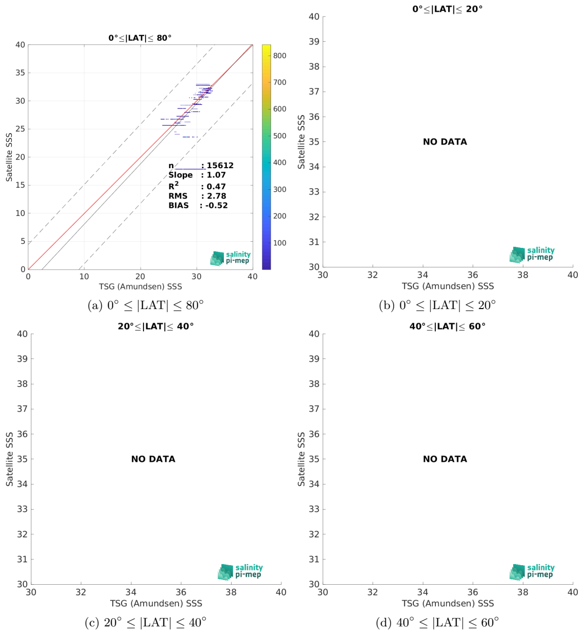
Figure 10: Contour maps of the concentration of Aquarius SSS L3 OR v5 - 7-Day running (NASA-GSFC) SSS (y-axis) versus TSG (Amundsen) SSS (x-axis) at match-up pairs for different latitude bands. For each plot, the red line shows x=y . The black thin and dashed lines indicate a linear fit through the data cloud and the \pm 95\% confidence levels, respectively. The number match-up pairs n , the slope and R^2 coefficient of the linear fit, the root mean square (RMS) and the mean bias between satellite and in situ data are indicated for each latitude band in each plots.
