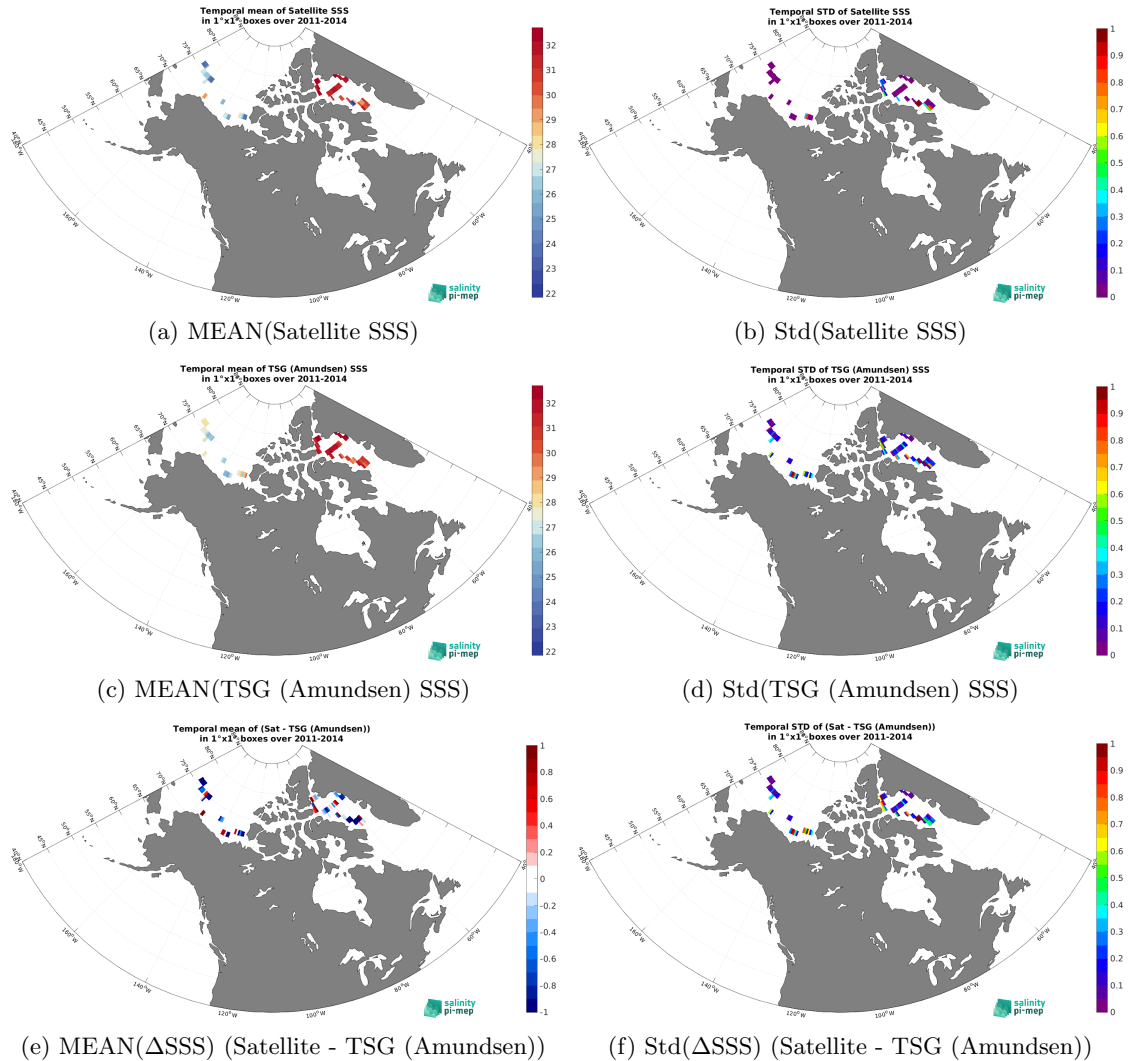
Figure 7: Temporal mean (left) and Std (right) of SSS from Aquarius SSS L3 OR v5 - 7-Day running (NASA-GSFC) (top), TSG (Amundsen) (middle), and of \Delta SSS (Satellite - TSG (Amundsen)). Only match-up pairs are used to generate these maps.
