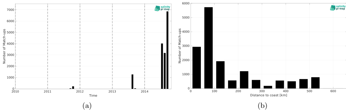
Figure 2: Number of match-ups between TSG (Amundsen) and Aquarius SSS L3 OR v5 - 7-Day running (NASA-GSFC) SSS as a function of time (a) and as function of the distance to coast (b) over the Arctic Ocean Pi-MEP region and for the full satellite product period.
