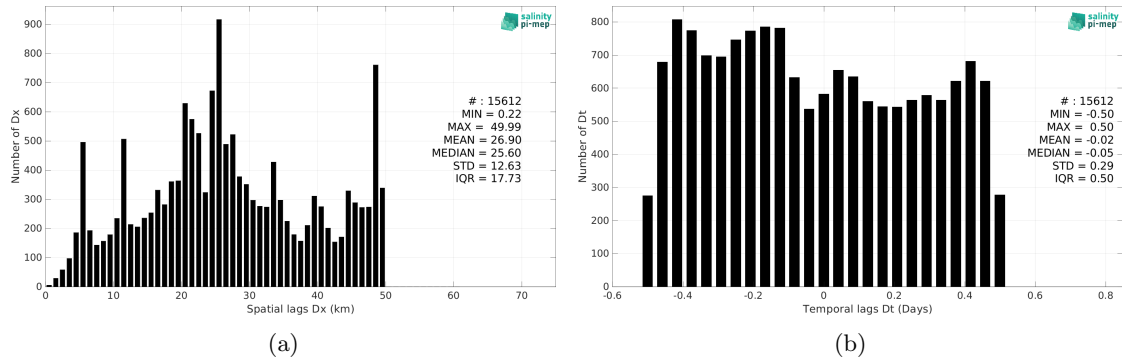
Figure 6: Histograms of the spatial (a) and temporal (b) lags between the location/time of the TSG (Amundsen) measurement and the date of the corresponding Aquarius SSS L3 OR v5 - 7-Day running (NASA-GSFC) SSS pixel.
