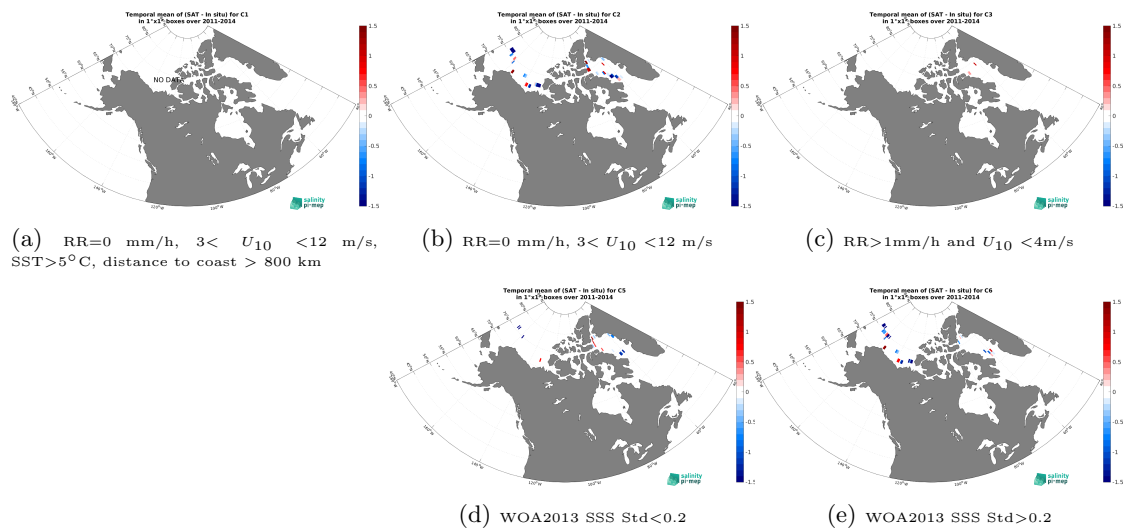
Figure 14: Temporal mean gridded over spatial boxes of size 1^\circ \times 1^\circ of \Delta SSS (Aquarius SSS L3 OR v5 - 7-Day running (NASA-GSFC) - TSG (Amundsen)) for 5 different subdatasets corresponding to: RR=0 mm/h, 3 < U_{10} < 12 m/s, SST > 5°C, distance to coast > 800 km (a), RR=0 mm/h, 3 < U_{10} < 12 m/s (b), RR > 1mm/h and U_{10} < 4 m/s (c), WOA2013 SSS Std < 0.2 (d), WOA2013 SSS Std > 0.2 (e).
