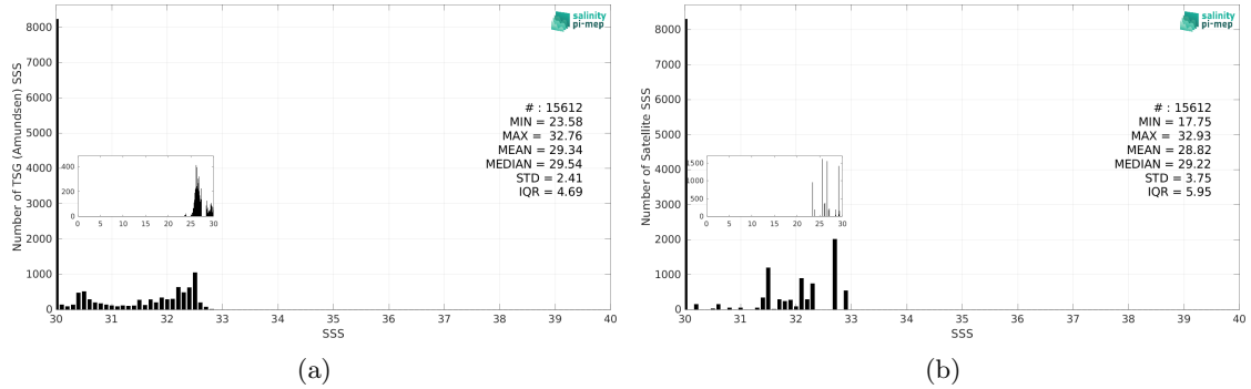
Figure 3: Histograms of SSS from TSG (Amundsen) (a) and Aquarius SSS L3 OR v5 - 7-Day running (NASA-GSFC) (b) considering all match-up pairs per bins of 0.1 over the Arctic Ocean Pi-MEP region and for the full satellite product period.
