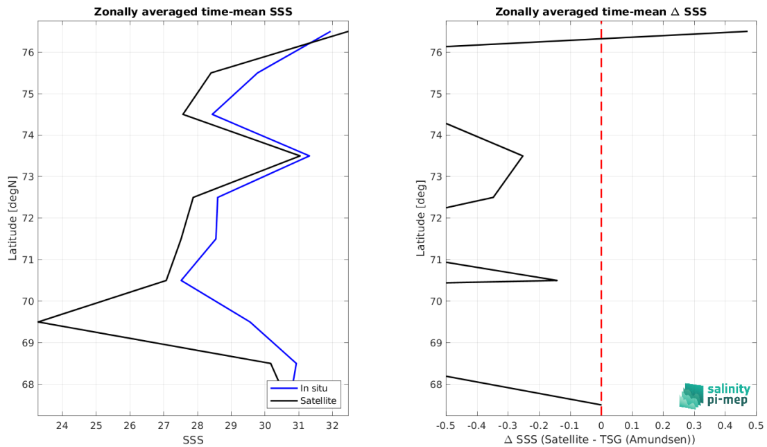
Figure 9: Left panel: Zonal mean SSS from Aquarius SSS L3 OR v5 - 7-Day running (NASA-GSFC) satellite product (black) and from TSG (Amundsen) (blue). Right panel: Zonal mean of \Delta SSS (Satellite - TSG (Amundsen)) for all the collected Pi-MEP match-up pairs estimated over the full satellite product period.
