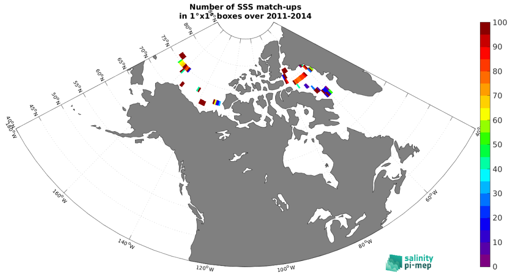
Figure 5: Number of SSS match-ups between TSG (Amundsen) SSS and the Aquarius SSS L3 OR v5 - 7-Day running (NASA-GSFC) SSS product for the Arctic Ocean Pi-MEP region over 1°×1° boxes and for the full satellite product period.
