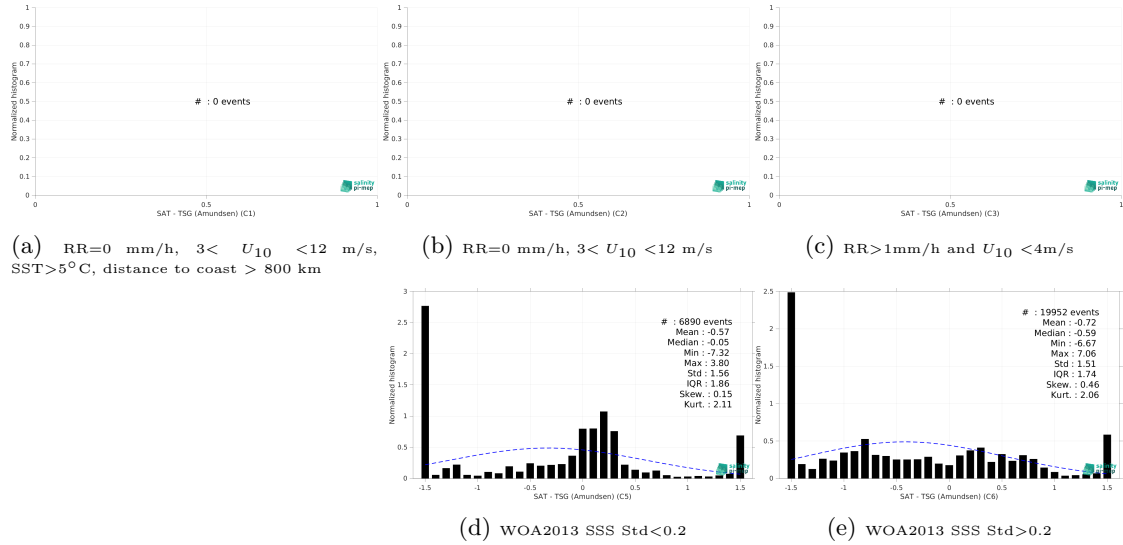
Figure 13: Normalized histogram of \Delta SSS (Aquarius SSS L3 OR v5 - 7-Day running (NASA-GSFC) - TSG (Amundsen)) for 5 different subdatasets corresponding to: RR=0 mm/h, 3 < U_{10} < 12 m/s, SST>5°C, distance to coast > 800 km (a), RR=0 mm/h, 3 < U_{10} < 12 m/s (b), RR>1mm/h and U_{10} < 4 m/s (c), WOA2013 SSS Std<0.2 (d), WOA2013 SSS Std>0.2 (e).
