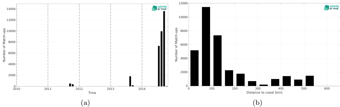
Figure 1: Number of match-ups between TSG (Amundsen) and Aquarius SSS L3 OR v5 - 7-Day running (NASA-GSFC) SSS as a function of time (a) and as function of the distance to coast (b) over the Arctic Ocean Pi-MEP region and for the full satellite product period.
