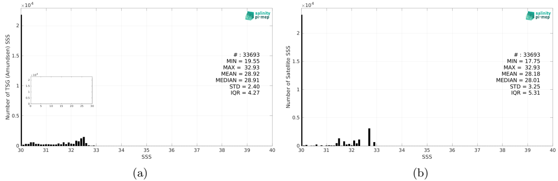
Figure 2: Histograms of SSS from TSG (Amundsen) (a) and Aquarius SSS L3 OR v5 - 7-Day running (NASA-GSFC) (b) considering all match-up pairs per bins of 0.1 over the Arctic Ocean Pi-MEP region and for the full satellite product period.
