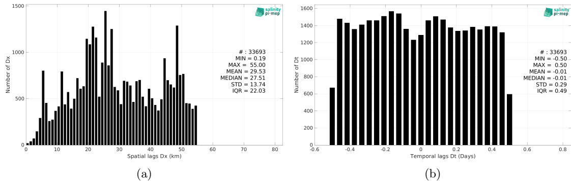
Figure 5: Histograms of the spatial (a) and temporal (b) lags between the location/time of the TSG (Amundsen) measurement and the date of the corresponding Aquarius SSS L3 OR v5 - 7-Day running (NASA-GSFC) SSS pixel.
