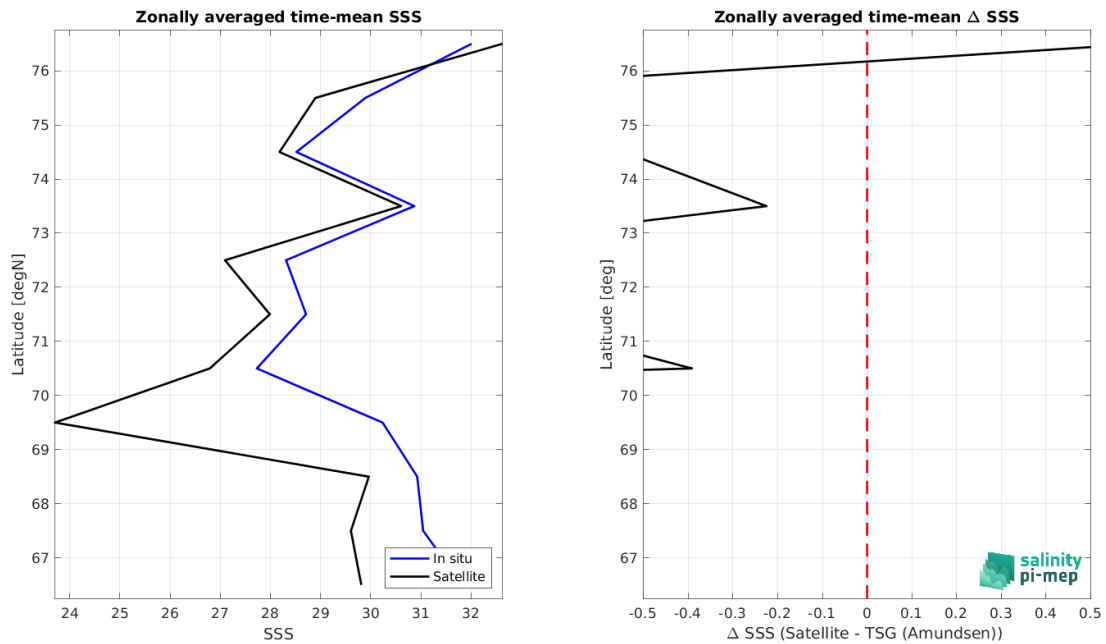
Figure 8: Left panel: Zonal mean SSS from Aquarius SSS L3 OR v5 - 7-Day running (NASA-GSFC) satellite product (black) and from TSG (Amundsen) (blue). Right panel: Zonal mean of \Delta SSS (Satellite - TSG (Amundsen)) for all the collected Pi-MEP match-up pairs estimated over the full satellite product period.
