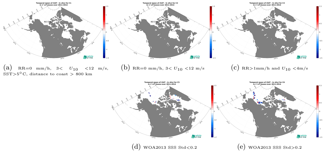
Figure 12: Temporal mean gridded over spatial boxes of size 1^{\circ}\times 1^{\circ} of \Delta\text{SSS} (Aquarius SSS L3 OR v5 - 7-Day running (NASA-GSFC) - TSG (Amundsen)) for 5 different subdatasets corresponding to:RR=0 mm/h, 3 < U_{10} < 12 m/s, SST > 5^{\circ}\text{C} , distance to coast > 800 km (a), RR=0 mm/h, 3 < U_{10} < 12 m/s (b), RR > 1 mm/h and U_{10} < 4 m/s (c), WOA2013 SSS Std < 0.2 (d), WOA2013 SSS Std > 0.2 (e).
