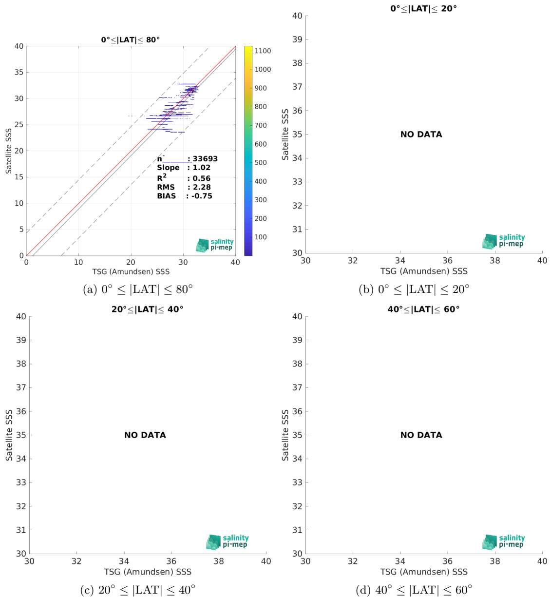
Figure 9: Contour maps of the concentration of Aquarius SSS L3 OR v5 - 7-Day running (NASA-GSFC) SSS (y-axis) versus TSG (Amundsen) SSS (x-axis) at match-up pairs for different latitude bands. For each plot, the red line shows x=y . The black thin and dashed lines indicate a linear fit through the data cloud and the \pm 95\% confidence levels, respectively. The number match-up pairs n , the slope and R^2 coefficient of the linear fit, the root mean square (RMS) and the mean bias between satellite and in situ data are indicated for each latitude band in each plot.
