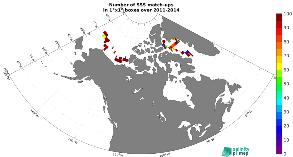
Figure 4: Number of SSS match-ups between TSG (Amundsen) SSS and the Aquarius SSS L3 OR v5 - 7-Day running (NASA-GSFC) SSS product for the Arctic Ocean Pi-MEP region over 1°x1° boxes and for the full satellite product period.
