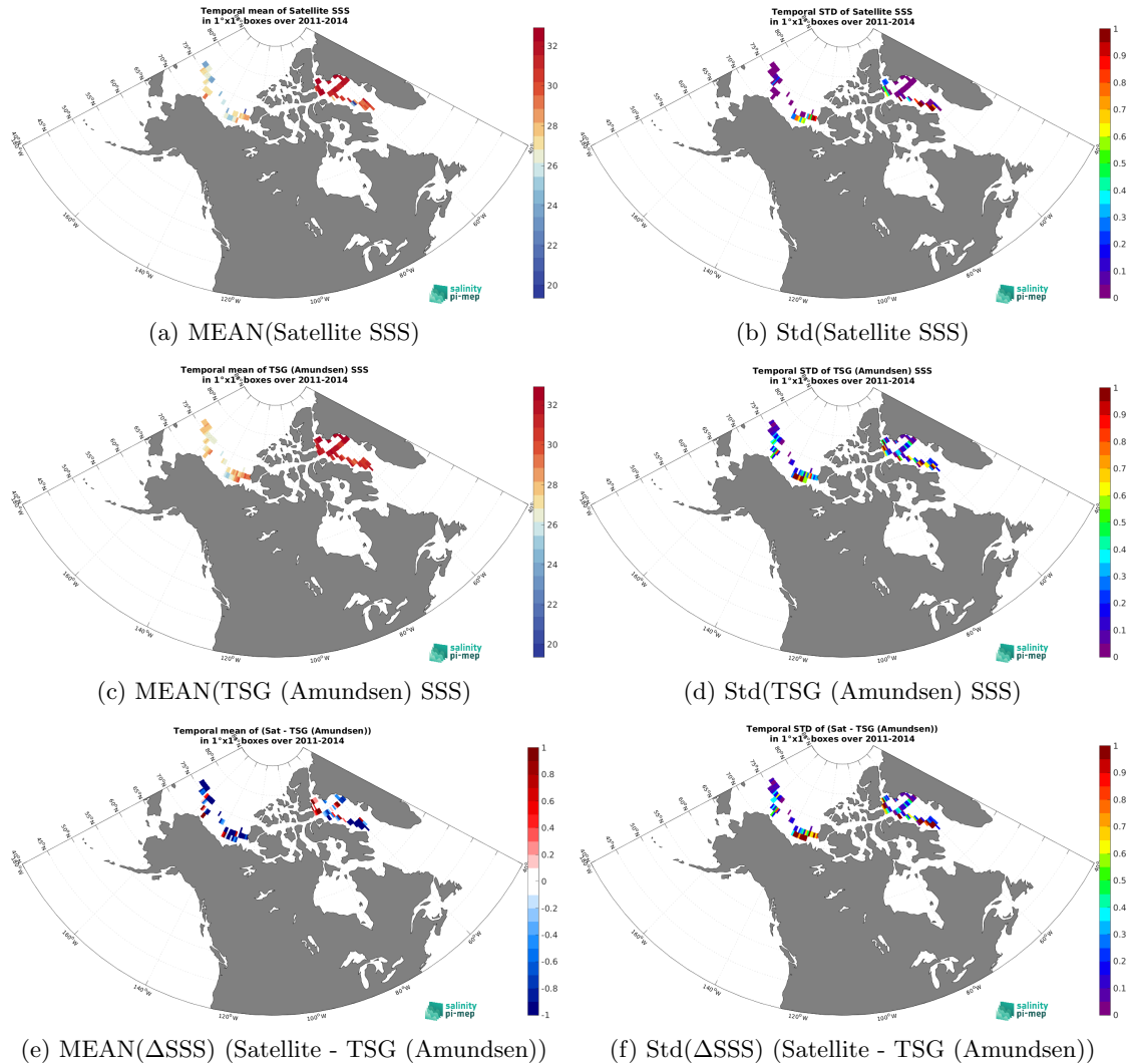
Figure 6: Temporal mean (left) and Std (right) of SSS from Aquarius SSS L3 OR v5 - 7-Day running (NASA-GSFC) (top), TSG (Amundsen) (middle), and of \Delta SSS (Satellite - TSG (Amundsen)). Only match-up pairs are used to generate these maps.
