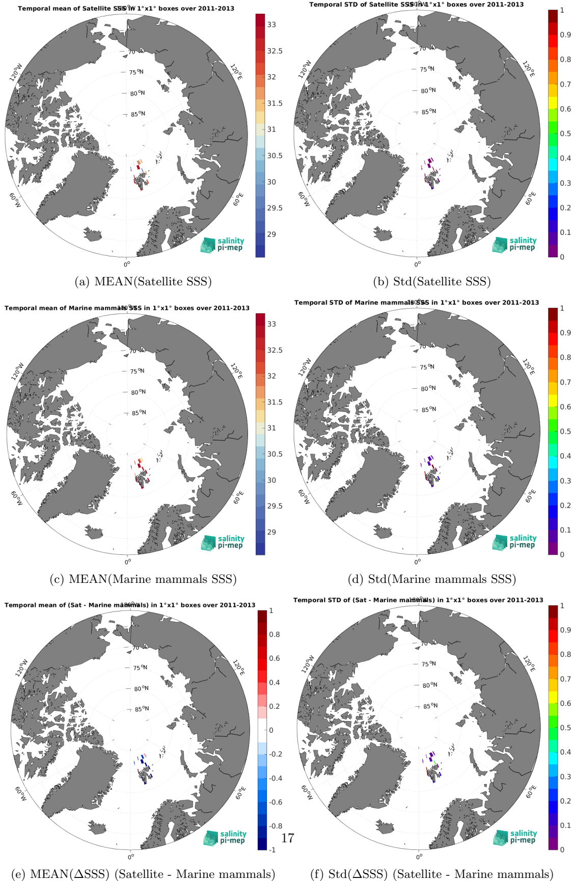
Figure 7: Temporal mean (left) and Std (right) of SSS from Aquarius SSS L3 OR v5 - 7-Day running (NASA-GSFC) (top), Marine mammals (middle), and of \Delta SSS (Satellite - Marine mammals). Only match-up pairs are used to generate these maps.
