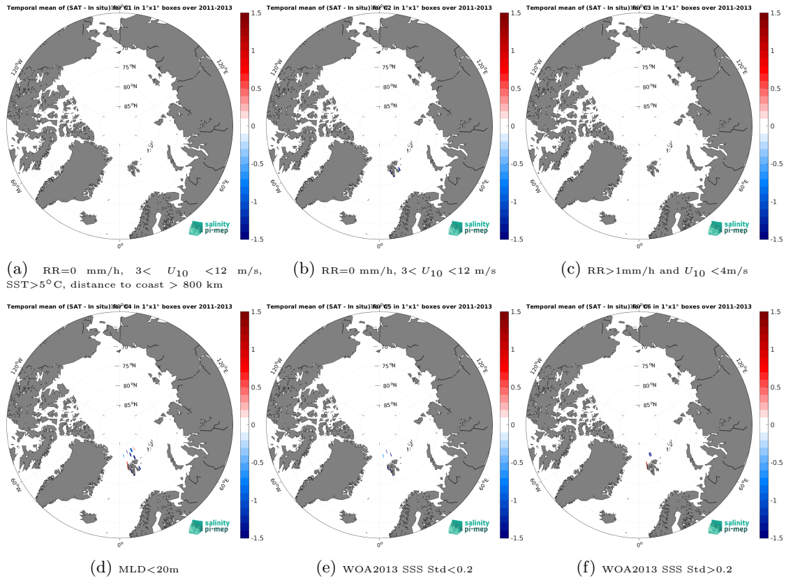
Figure 14: Temporal mean gridded over spatial boxes of size 1^\circ \times 1^\circ of \Delta SSS (Aquarius SSS L3 OR v5 - 7-Day running (NASA-GSFC) - Marine mammals) for 6 different subdatasets corresponding to: RR=0 mm/h, 3 < U_{10} < 12 m/s, SST > 5°C, distance to coast > 800 km (a), RR=0 mm/h, 3 < U_{10} < 12 m/s (b), RR > 1mm/h and U_{10} < 4 m/s (c), MLD < 20m (d), WOA2013 SSS Std < 0.2 (e), WOA2013 SSS Std > 0.2 (f).
