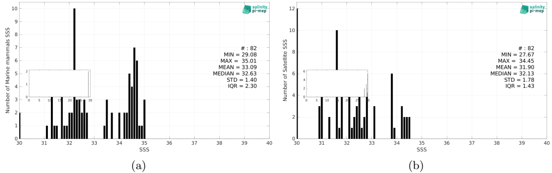
Figure 3: Histograms of SSS from Marine mammals (a) and Aquarius SSS L3 OR v5 - 7-Day running (NASA-GSFC) (b) considering all match-up pairs per bins of 0.1 over the Arctic Ocean Pi-MEP region and for the full satellite product period.
