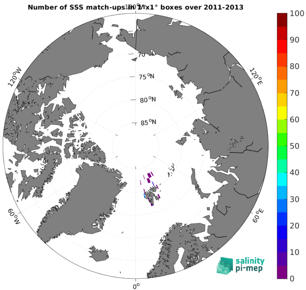
Figure 5: Number of SSS match-ups between Marine mammals SSS and the Aquarius SSS L3 OR v5 - 7-Day running (NASA-GSFC) SSS product for the Arctic Ocean Pi-MEP region over 1^\circ \times 1^\circ boxes and for the full satellite product period.
