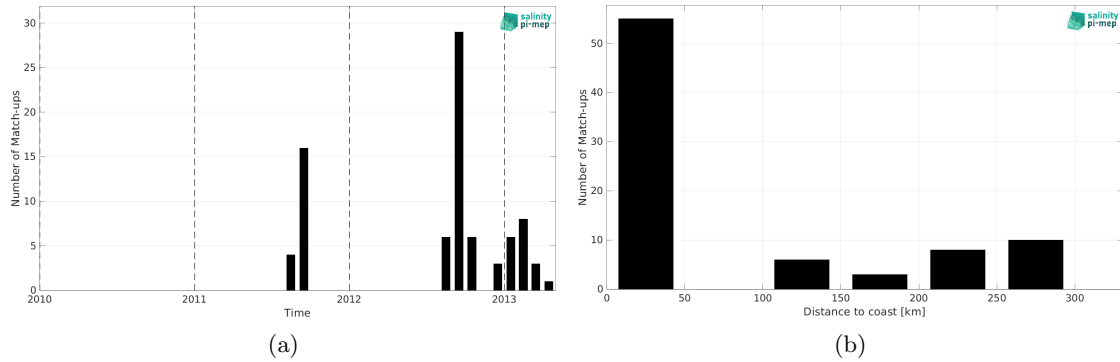
Figure 2: Number of match-ups between Marine mammals and Aquarius SSS L3 OR v5 - 7-Day running (NASA-GSFC) SSS as a function of time (a) and as function of the distance to coast (b) over the Arctic Ocean Pi-MEP region and for the full satellite product period.
