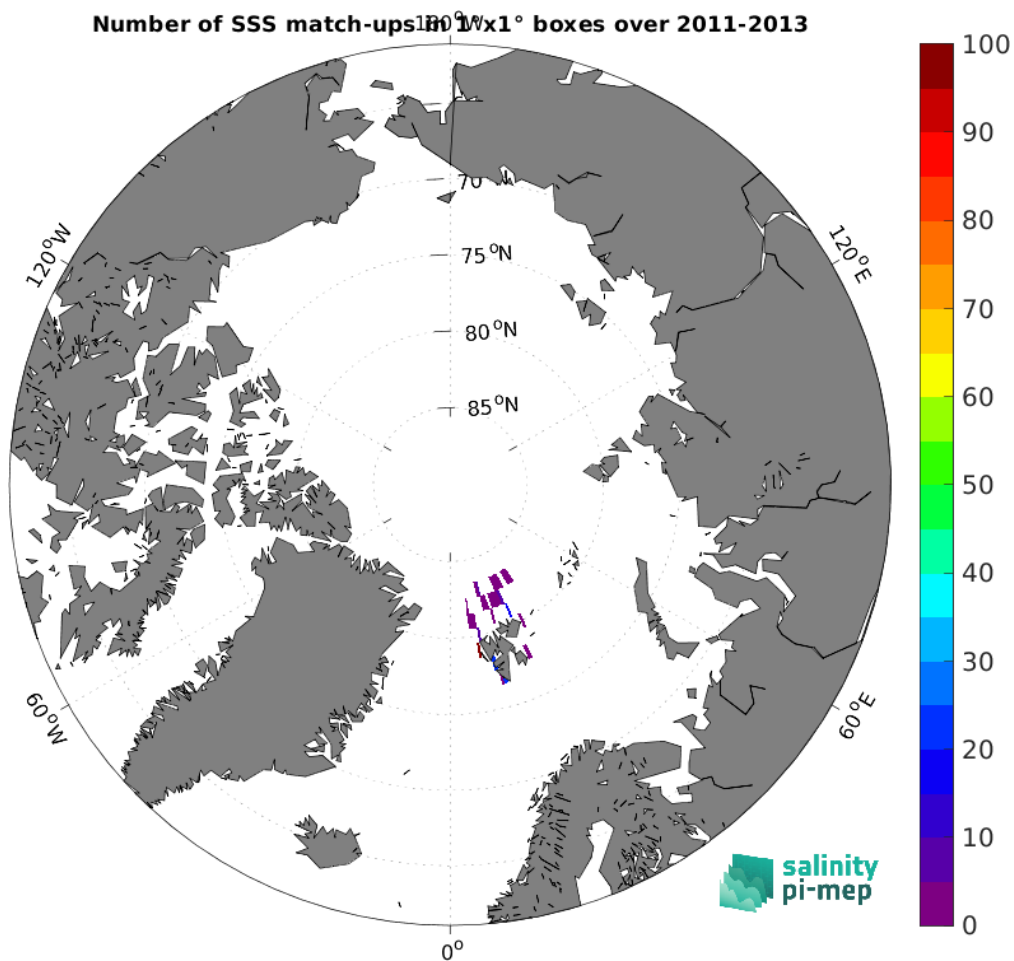
Figure 4: Number of SSS match-ups between Marine mammals SSS and the Aquarius SSS L3 OR v5 - 7-Day running (NASA-GSFC) SSS product for the Arctic Ocean Pi-MEP region over 1^{\circ} \times 1^{\circ} boxes and for the full satellite product period.
