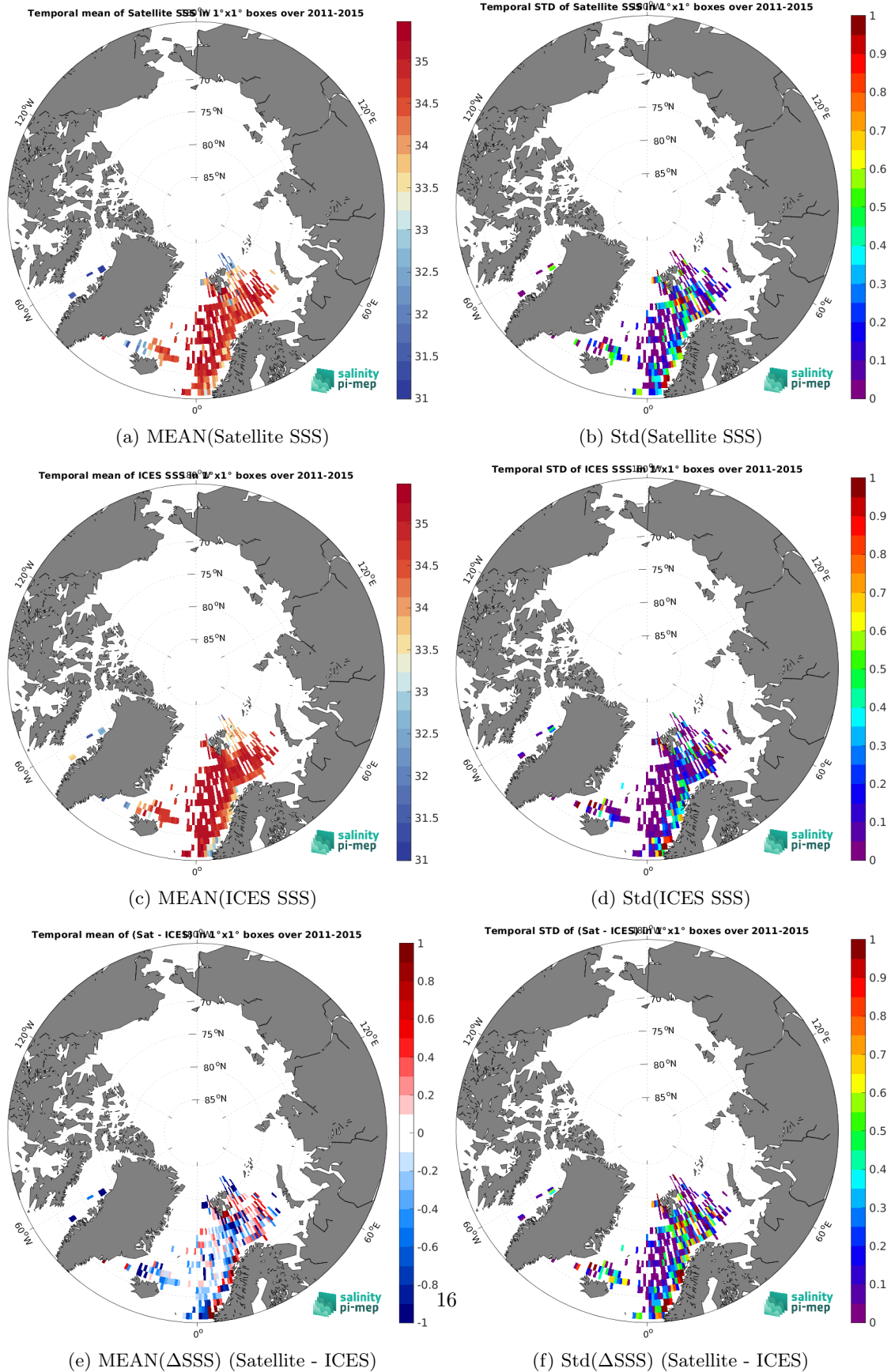
Figure 7: Temporal mean (left) and Std (right) of SSS from Aquarius SSS L3 OR v5 - 7-Day running (NASA-GSFC) (top), ICES (middle), and of \Delta SSS (Satellite - ICES). Only match-up pairs are used to generate these maps.
