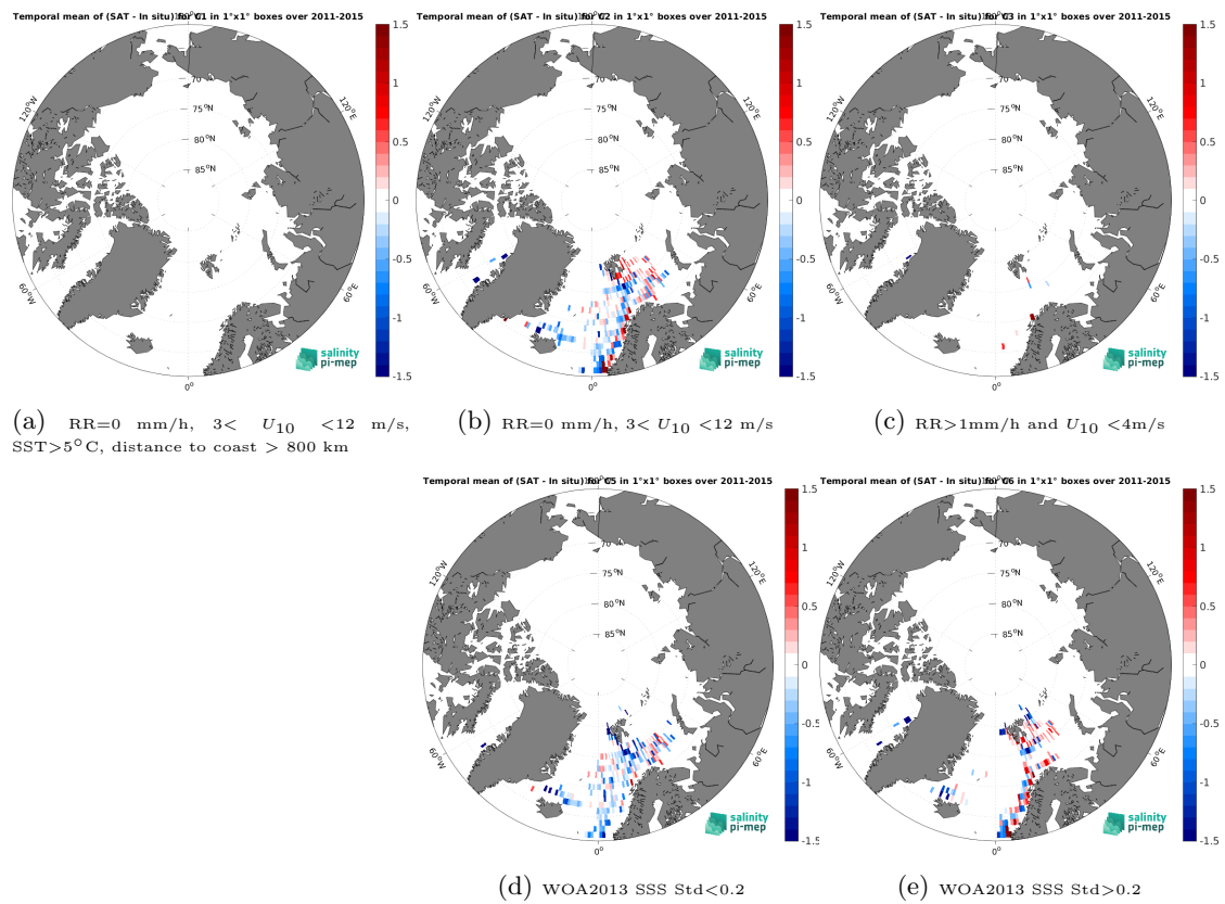
Figure 14: Temporal mean gridded over spatial boxes of size 1^\circ \times 1^\circ of \Delta\text{SSS} (Aquarius SSS L3 OR v5 - 7-Day running (NASA-GSFC) - ICES) for 5 different subdatasets corresponding to: RR=0 mm/h, 3 < U_{10} < 12 m/s, SST > 5°C, distance to coast > 800 km (a), RR=0 mm/h, 3 < U_{10} < 12 m/s (b), RR > 1mm/h and U_{10} < 4 m/s (c), WOA2013 SSS Std < 0.2 (d), WOA2013 SSS Std > 0.2 (e).
