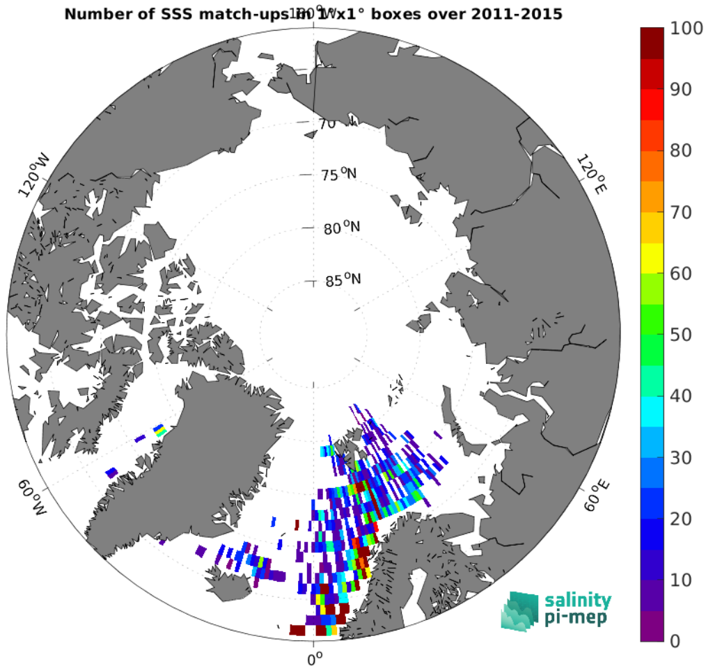
Figure 5: Number of SSS match-ups between ICES SSS and the Aquarius SSS L3 OR v5 - 7-Day running (NASA-GSFC) SSS product for the Arctic Ocean Pi-MEP region over 1^\circ \times 1^\circ boxes and for the full satellite product period.
