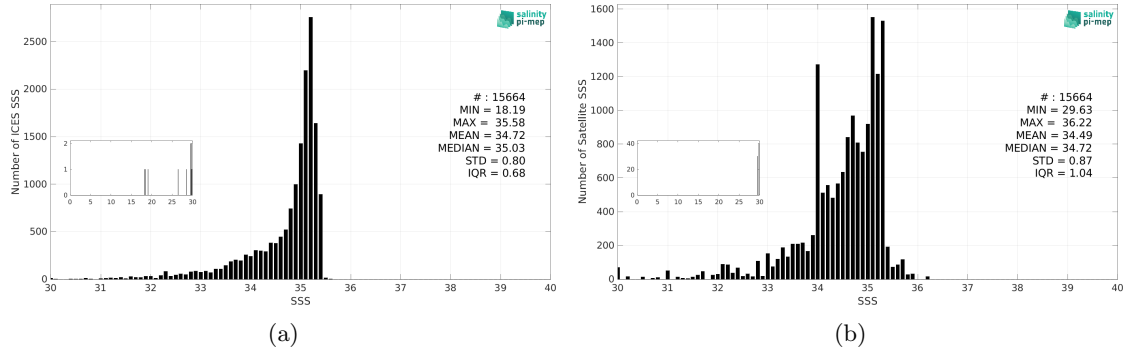
Figure 3: Histograms of SSS from ICES (a) and Aquarius SSS L3 OR v5 - 7-Day running (NASA-GSFC) (b) considering all match-up pairs per bins of 0.1 over the Arctic Ocean Pi-MEP region and for the full satellite product period.
