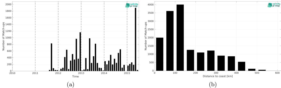
Figure 2: Number of match-ups between ICES and Aquarius SSS L3 OR v5 - 7-Day running (NASA-GSFC) SSS as a function of time (a) and as function of the distance to coast (b) over the Arctic Ocean Pi-MEP region and for the full satellite product period.
