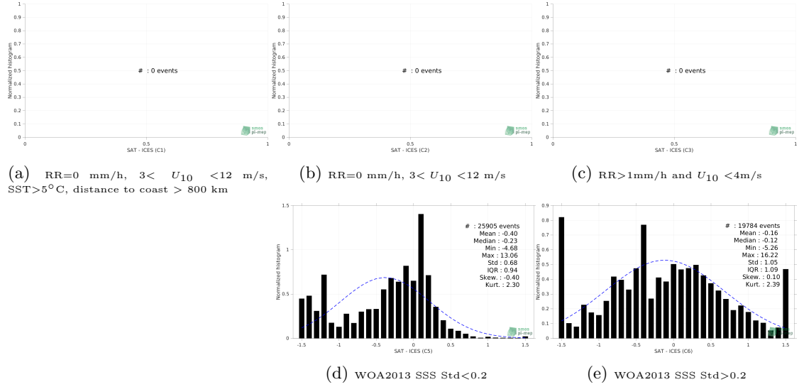
Figure 13: Normalized histogram of \Delta SSS (Aquarius SSS L3 OR v5 - 7-Day running (NASA-GSFC) - ICES) for 5 different subdatasets corresponding to: RR=0 mm/h, 3 < U_{10} < 12 m/s, SST > 5°C, distance to coast > 800 km (a), RR=0 mm/h, 3 < U_{10} < 12 m/s (b), RR > 1mm/h and U_{10} < 4 m/s (c), WOA2013 SSS Std < 0.2 (d), WOA2013 SSS Std > 0.2 (e).
