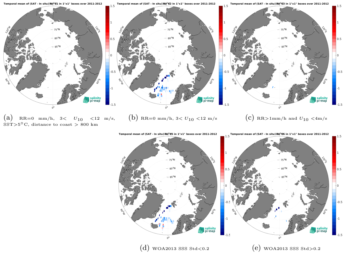
Figure 13: Temporal mean gridded over spatial boxes of size 1^\circ \times 1^\circ of \Delta SSS (Aquarius SSS L3 OR v5 - 7-Day running (NASA-GSFC) - Surface drifters) for 5 different subdatasets corresponding to: RR=0 mm/h, 3 < U_{10} < 12 m/s, SST > 5^\circ\text{C} , distance to coast > 800 km (a), RR=0 mm/h, 3 < U_{10} < 12 m/s (b), RR > 1 mm/h and U_{10} < 4 m/s (c), WOA2013 SSS Std < 0.2 (d), WOA2013 SSS Std > 0.2 (e).
