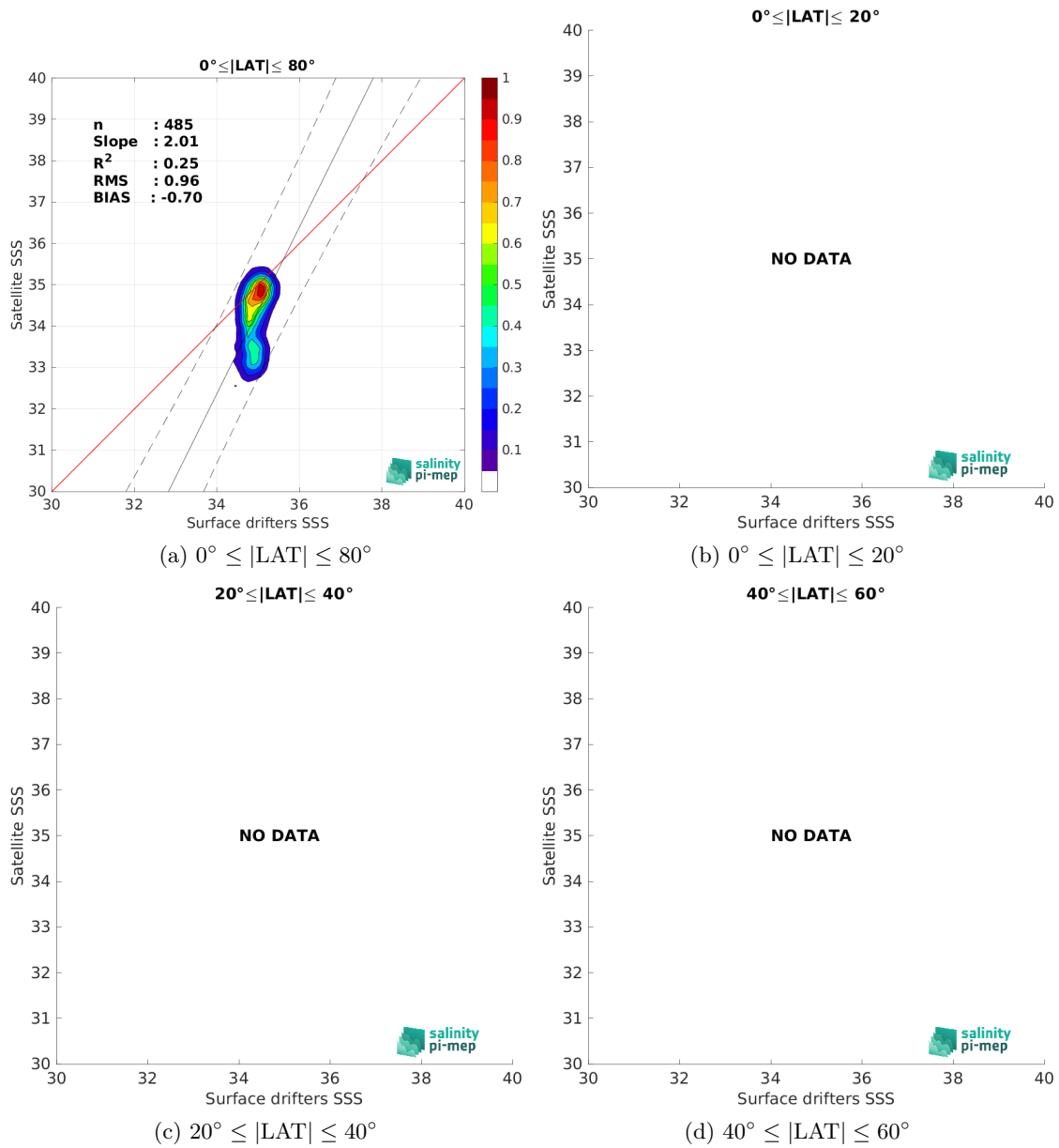
Figure 9: Contour maps of the concentration of Aquarius SSS L3 OR v5 - 7-Day running (NASA-GSFC) SSS (y-axis) versus Surface drifters SSS (x-axis) at match-up pairs for different latitude bands. For each plot, the red line shows x=y . The black thin and dashed lines indicate a linear fit through the data cloud and the \pm 95\% confidence levels, respectively. The number match-up pairs n , the slope and R^2 coefficient of the linear fit, the root mean square (RMS) and the mean bias between satellite and in situ data are indicated for each latitude band in each plots.
