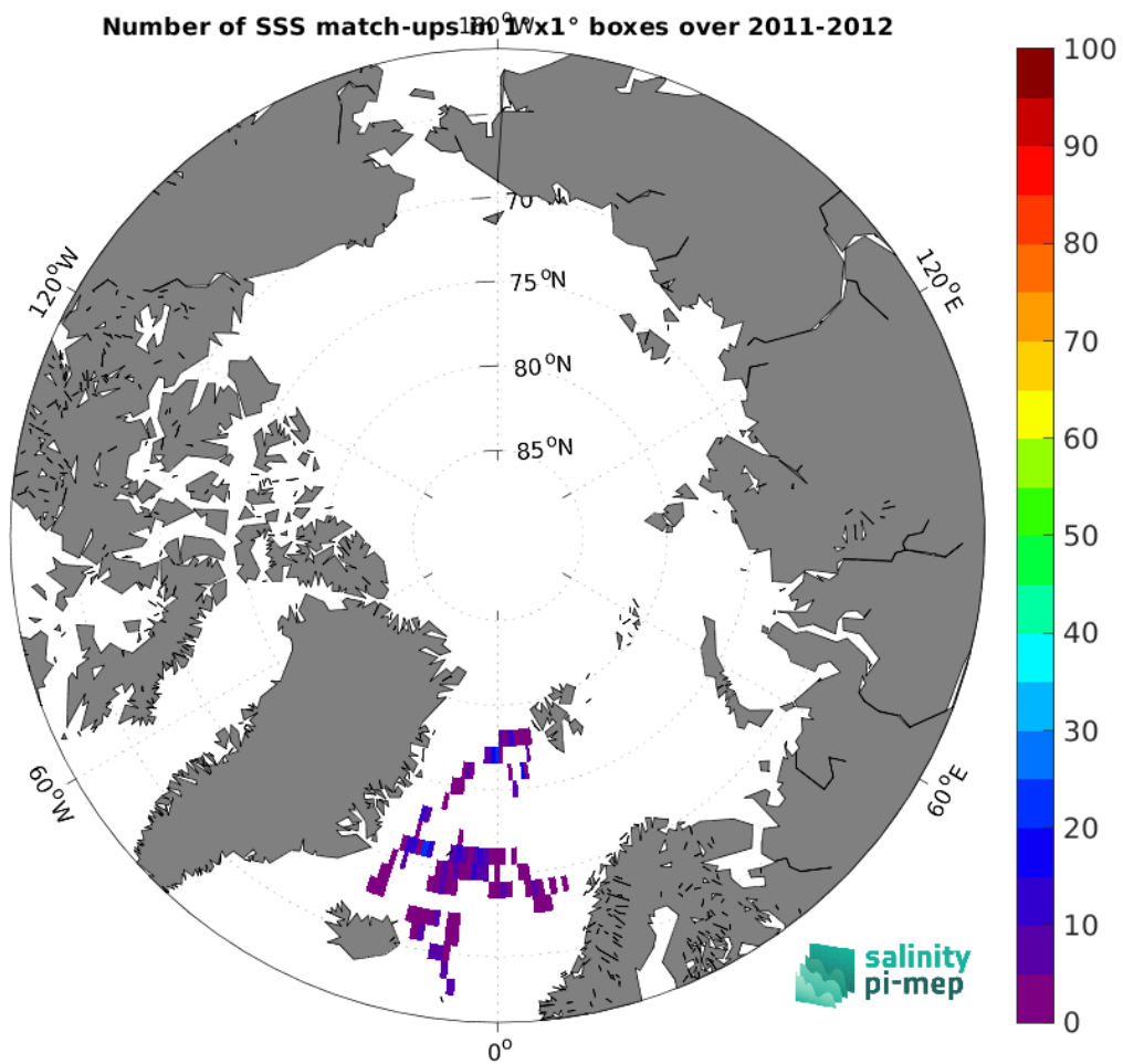
Figure 4: Number of SSS match-ups between Surface drifters SSS and the Aquarius SSS L3 OR v5 - 7-Day running (NASA-GSFC) SSS product for the Arctic Ocean Pi-MEP region over 1^\circ \times 1^\circ boxes and for the full satellite product period.
