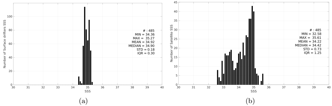
Figure 3: Histograms of SSS from Surface drifters (a) and Aquarius SSS L3 OR v5 - 7-Day running (NASA-GSFC) (b) considering all match-up pairs per bins of 0.1 over the Arctic Ocean Pi-MEP region and for the full satellite product period.
