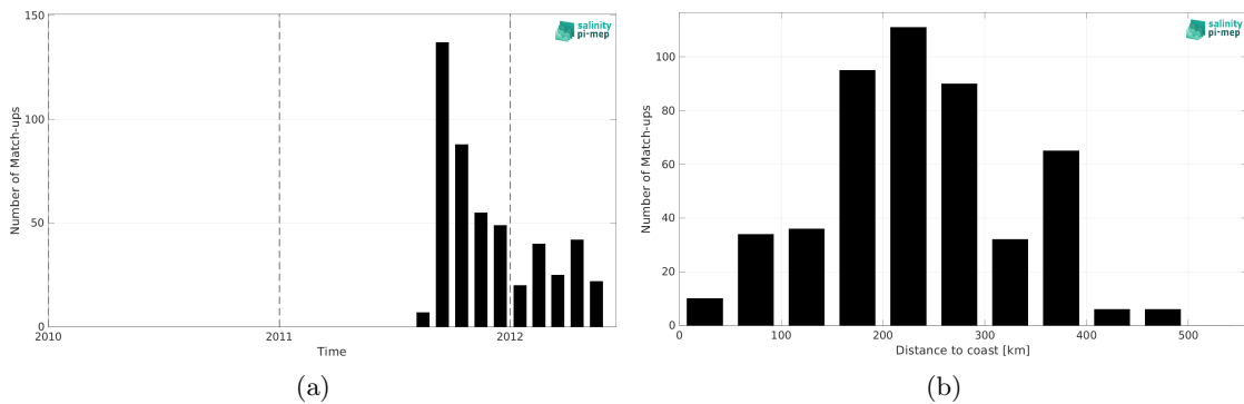
Figure 2: Number of match-ups between Surface drifters and Aquarius SSS L3 OR v5 - 7-Day running (NASA-GSFC) SSS as a function of time (a) and as function of the distance to coast (b) over the Arctic Ocean Pi-MEP region and for the full satellite product period.
