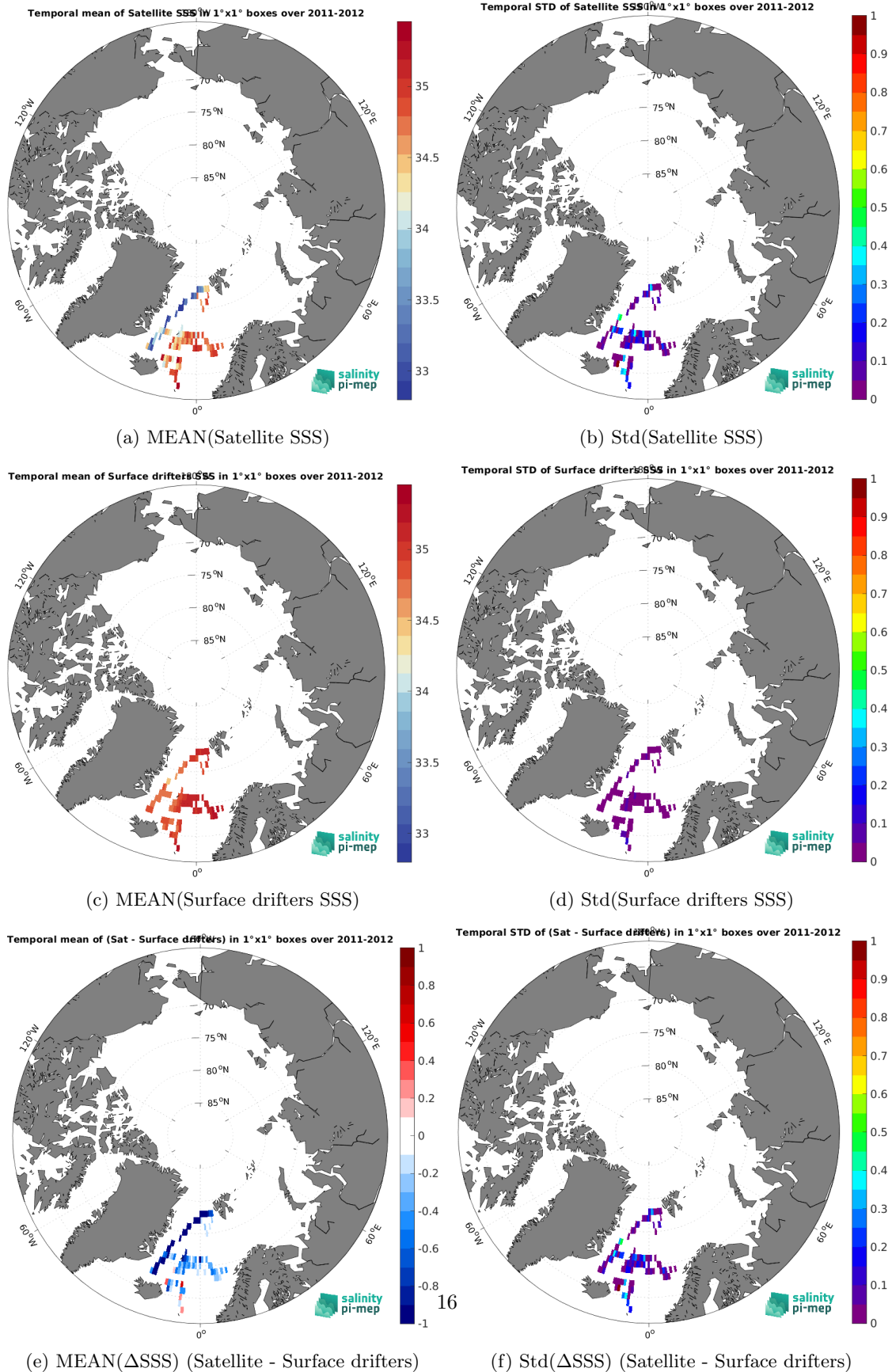
Figure 6: Temporal mean (left) and Std (right) of SSS from Aquarius SSS L3 OR v5 - 7-Day running (NASA-GSFC) (top), Surface drifters (middle), and of \Delta SSS (Satellite - Surface drifters). Only match-up pairs are used to generate these maps.
