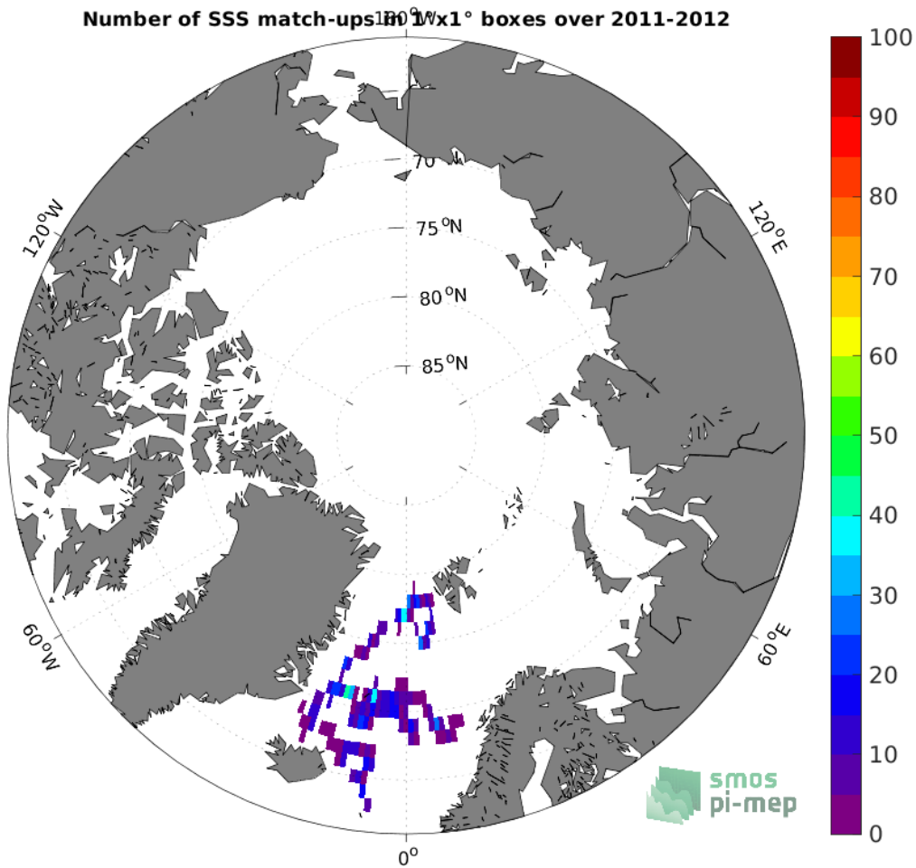
Figure 3: Number of SSS match-ups between Surface drifters SSS and the Aquarius SSS L3 OR v5 - 7-Day running (NASA-GSFC) SSS product for the Arctic Ocean Pi-MEP region over 1^{\circ} \times 1^{\circ} boxes and for the full satellite product period.
