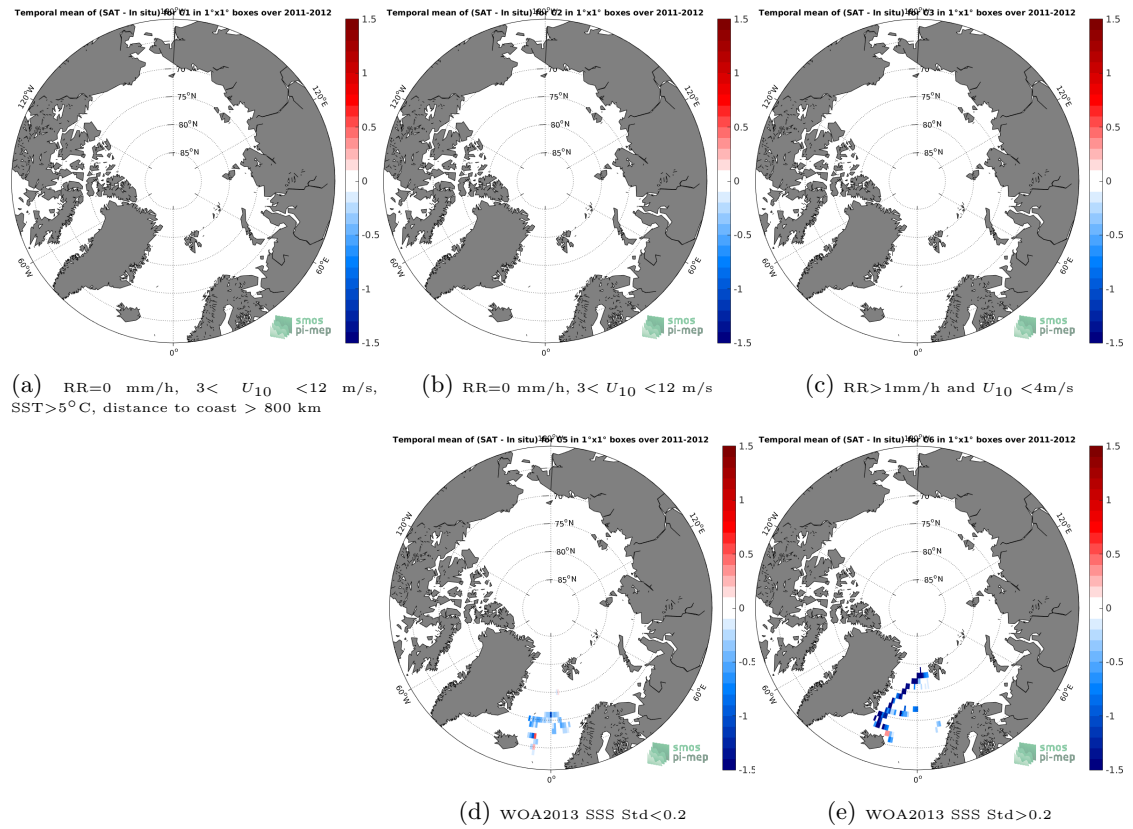
Figure 11: Temporal mean gridded over spatial boxes of size 1^\circ \times 1^\circ of \Delta SSS (Aquarius-L3-OR-V5-7DAY-RUNNING-1DEG - Surface drifters) for 5 different subdatasets corresponding to:RR=0 mm/h, 3 < U_{10} < 12 m/s, SST >5^\circ C, distance to coast > 800 km (a), RR=0 mm/h, 3 < U_{10} < 12 m/s (b), RR >1 mm/h and U_{10} < 4 m/s (c), WOA2013 SSS Std <0.2 (d), WOA2013 SSS Std >0.2 (e).
