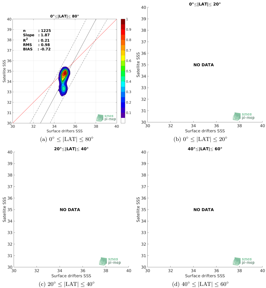
Figure 8: Contour maps of the concentration of Aquarius-L3-OR-V5-7DAY-RUNNING-1DEG SSS (y-axis) versus Surface drifters SSS (x-axis) at match-up pairs for different latitude bands. For each plot, the red line shows x=y . The black thin and dashed lines indicate a linear fit through the data cloud and the \pm 95\% confidence levels, respectively. The number match-up pairs n , the slope and R^2 coefficient of the linear fit, the root mean square (RMS) and the mean bias between satellite and in situ data are indicated for each latitude band in each plots.
