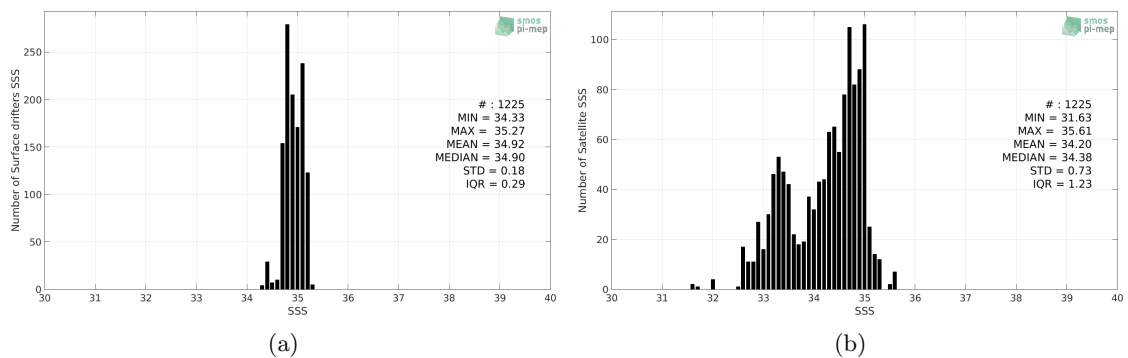
Figure 2: Histograms of SSS from Surface drifters (a) and Aquarius-L3-OR-V5-7DAY-RUNNING-1DEG (b) considering all match-up pairs per bins of 0.1 over the Arctic Ocean Pi-MEP region and for the full satellite product period.
