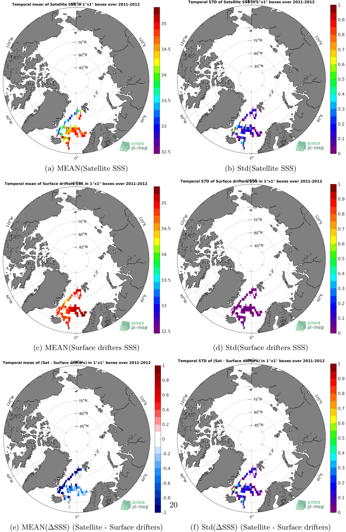
Figure 5: Temporal mean (left) and Std (right) of SSS from Aquarius-L3-OR-V5-7DAY-RUNNING-1DEG (top), Surface drifters (middle), and of \Delta SSS (Satellite - Surface drifters). Only match-up pairs are used to generate these maps.
