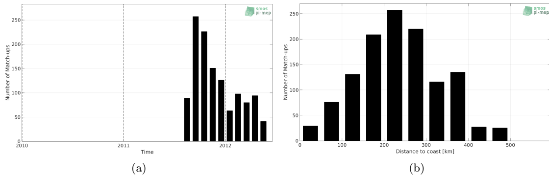
Figure 1: Number of match-ups between Surface drifters and Aquarius-L3-OR-V5-7DAY-RUNNING-1DEG SSS as a function of time (a) and as function of the distance to coast (b) over the Arctic Ocean Pi-MEP region and for the full satellite product period.
