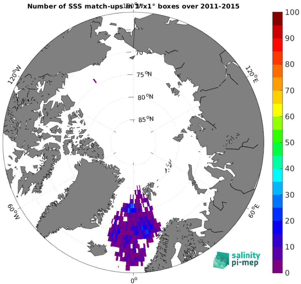
Figure 5: Number of SSS match-ups between Argo SSS and the Aquarius SSS L3 OR v5 - 7-Day running (NASA-GSFC) SSS product for the Arctic Ocean Pi-MEP region over 1^\circ \times 1^\circ boxes and for the full satellite product period.
