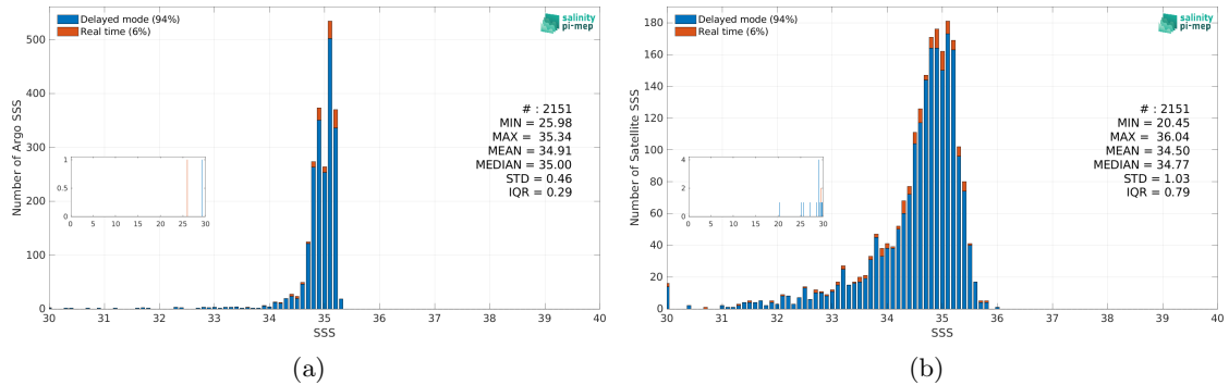
Figure 3: Histograms of SSS from Argo (a) and Aquarius SSS L3 OR v5 - 7-Day running (NASA-GSFC) (b) considering all match-up pairs per bins of 0.1 over the Arctic Ocean Pi-MEP region and for the full satellite product period.
