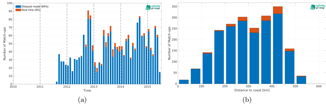
Figure 2: Number of match-ups between Argo and Aquarius SSS L3 OR v5 - 7-Day running (NASA-GSFC) SSS as a function of time (a) and as function of the distance to coast (b) over the Arctic Ocean Pi-MEP region and for the full satellite product period.
