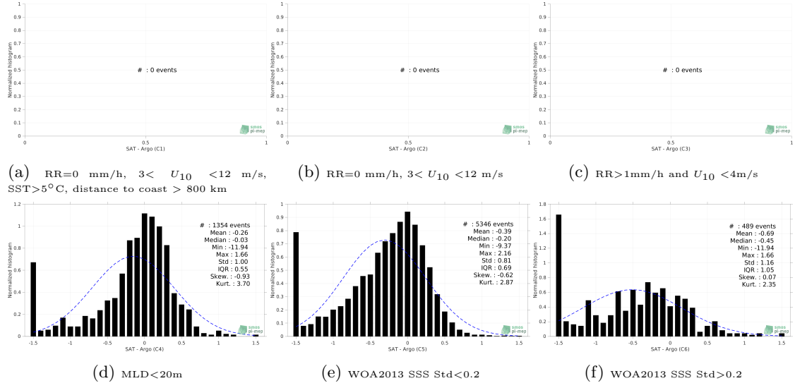
Figure 13: Normalized histogram of \Delta\text{SSS} (Aquarius SSS L3 OR v5 - 7-Day running (NASA-GSFC) - Argo) for 6 different subdatasets corresponding to: RR=0 mm/h, 3 < U_{10} < 12 m/s, SST > 5^{\circ}\text{C} , distance to coast > 800 km (a), RR=0 mm/h, 3 < U_{10} < 12 m/s (b), RR > 1\text{mm/h} and U_{10} < 4\text{m/s} (c), MLD < 20\text{m} (d), WOA2013 SSS Std < 0.2 (e), WOA2013 SSS Std > 0.2 (f).
