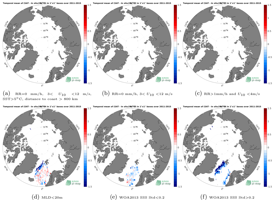
Figure 12: Temporal mean gridded over spatial boxes of size 1^{\circ}\times 1^{\circ} of \Delta\text{SSS} (Aquarius SSS L3 OR v5 - 7-Day running (NASA-GSFC) - Argo) for 6 different subdatasets corresponding to:RR=0 mm/h, 3 < U_{10} < 12 m/s, SST >5^{\circ}\text{C} , distance to coast > 800 km (a), RR=0 mm/h, 3 < U_{10} < 12 m/s (b), RR >1 mm/h and U_{10} < 4 m/s (c),MLD <20 m (d),WOA2013 SSS Std <0.2 (e),WOA2013 SSS Std >0.2 (f).
