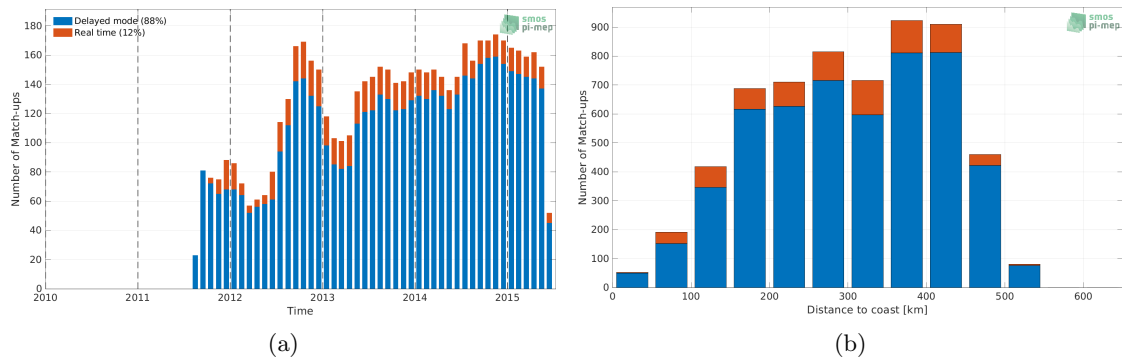
Figure 1: Number of match-ups between Argo and Aquarius SSS L3 OR v5 - 7-Day running (NASA-GSFC) SSS as a function of time (a) and as function of the distance to coast (b) over the Arctic Ocean Pi-MEP region and for the full satellite product period.
