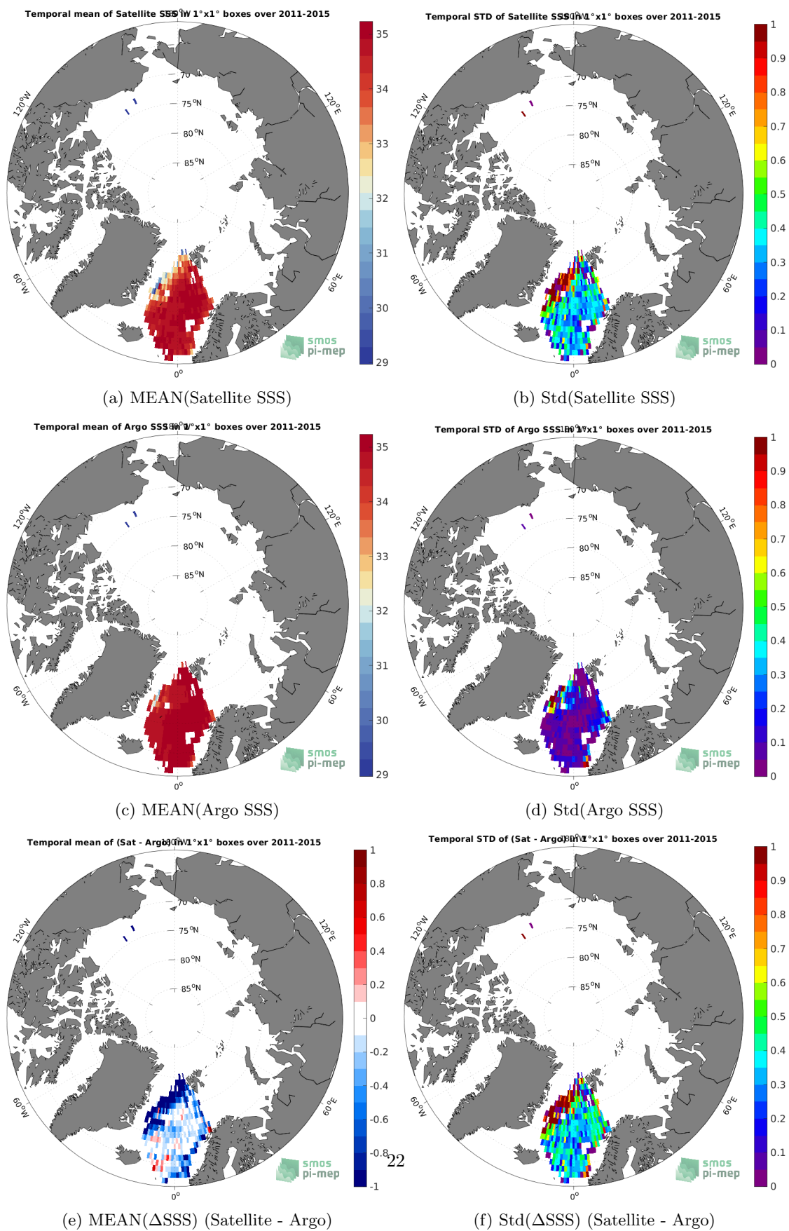
Figure 6: Temporal mean (left) and Std (right) of SSS from Aquarius SSS L3 OR v5 - 7-Day running (NASA-GSFC) (top), Argo (middle), and of \Delta SSS (Satellite - Argo). Only match-up pairs are used to generate these maps.
