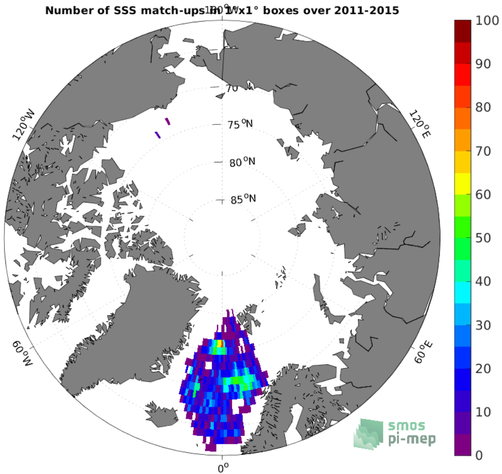
Figure 4: Number of SSS match-ups between Argo SSS and the Aquarius SSS L3 OR v5 - 7-Day running (NASA-GSFC) SSS product for the Arctic Ocean Pi-MEP region over 1^\circ \times 1^\circ boxes and for the full satellite product period.
