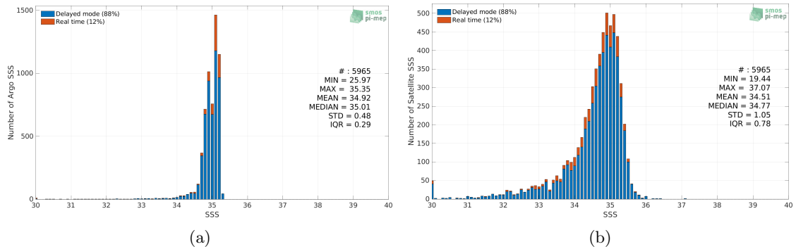
Figure 2: Histograms of SSS from Argo (a) and Aquarius SSS L3 OR v5 - 7-Day running (NASA-GSFC) (b) considering all match-up pairs per bins of 0.1 over the Arctic Ocean Pi-MEP region and for the full satellite product period.
