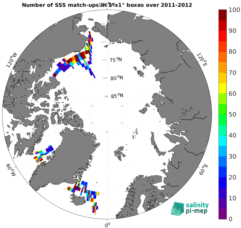
Figure 4: Number of SSS match-ups between TSG (SAMOS) SSS and the Aquarius SSS L3 OR v5 - 7-Day running - Rain mask (NASA-GSFC) SSS product for the Arctic Ocean Pi-MEP region over 1^{\circ} \times 1^{\circ} boxes and for the full satellite product period.
