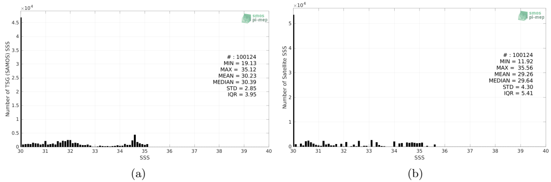
Figure 2: Histograms of SSS from TSG (SAMOS) (a) and Aquarius SSS L3 OR v5 - 7-Day running - Rain mask (NASA-GSFC) (b) considering all match-up pairs per bins of 0.1 over the Arctic Ocean Pi-MEP region and for the full satellite product period.
