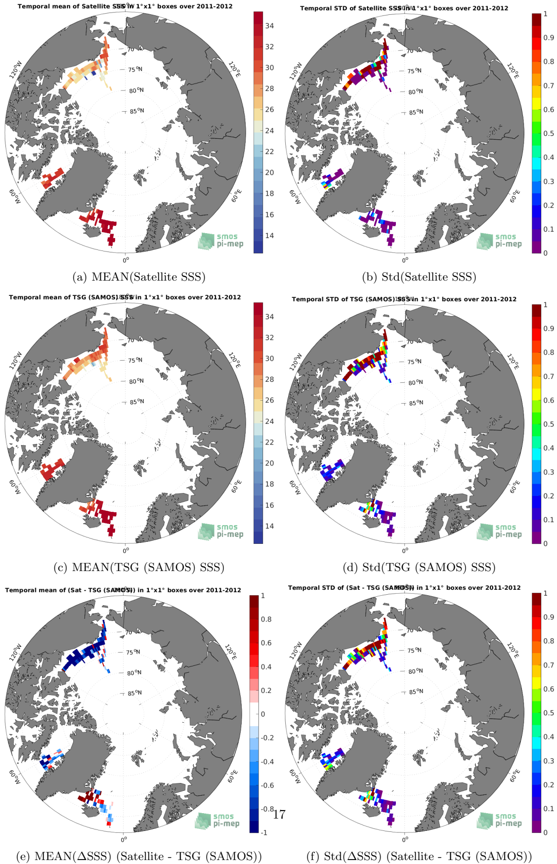
Figure 6: Temporal mean (left) and Std (right) of SSS from Aquarius SSS L3 OR v5 - 7-Day running - Rain mask (NASA-GSFC) (top), TSG (SAMOS) (middle), and of \Delta SSS (Satellite - TSG (SAMOS)). Only match-up pairs are used to generate these maps.
