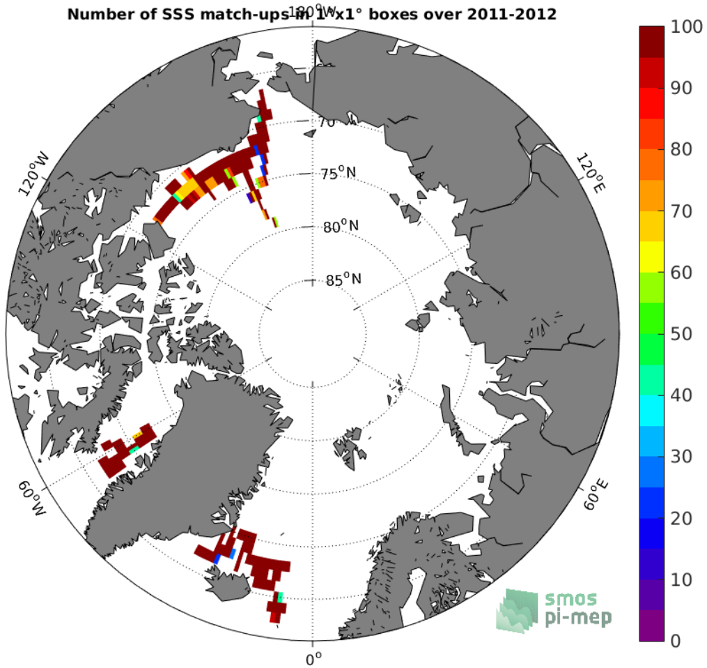
Figure 4: Number of SSS match-ups between TSG-SAMOS SSS and the Aquarius-L3-OR-V5-7DAY-RUNNING-RAIN-MASK-1DEG SSS product for the Arctic Ocean Pi-MEP region over 1°x1° boxes and for the full satellite product period.
