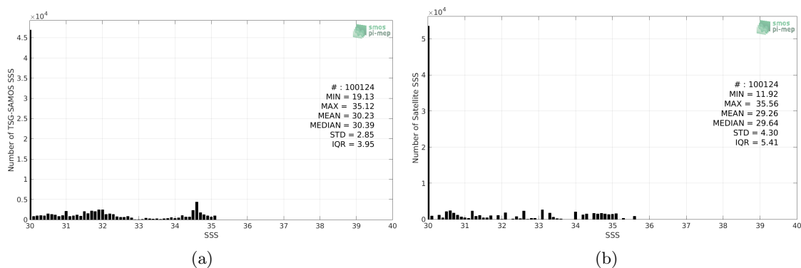
Figure 2: Histograms of SSS from TSG-SAMOS (a) and Aquarius-L3-OR-V5-7DAY-RUNNING-RAIN-MASK-1DEG (b) considering all match-up pairs per bins of 0.1 over the Arctic Ocean Pi-MEP region and for the full satellite product period.
