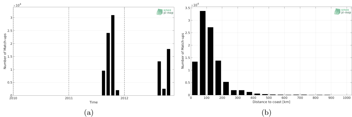
Figure 1: Number of match-ups between TSG-SAMOS and Aquarius-L3-OR-V5-7DAY-RUNNING-RAIN-MASK-1DEG SSS as a function of time (a) and as function of the distance to coast (b) over the Arctic Ocean Pi-MEP region and for the full satellite product period.
