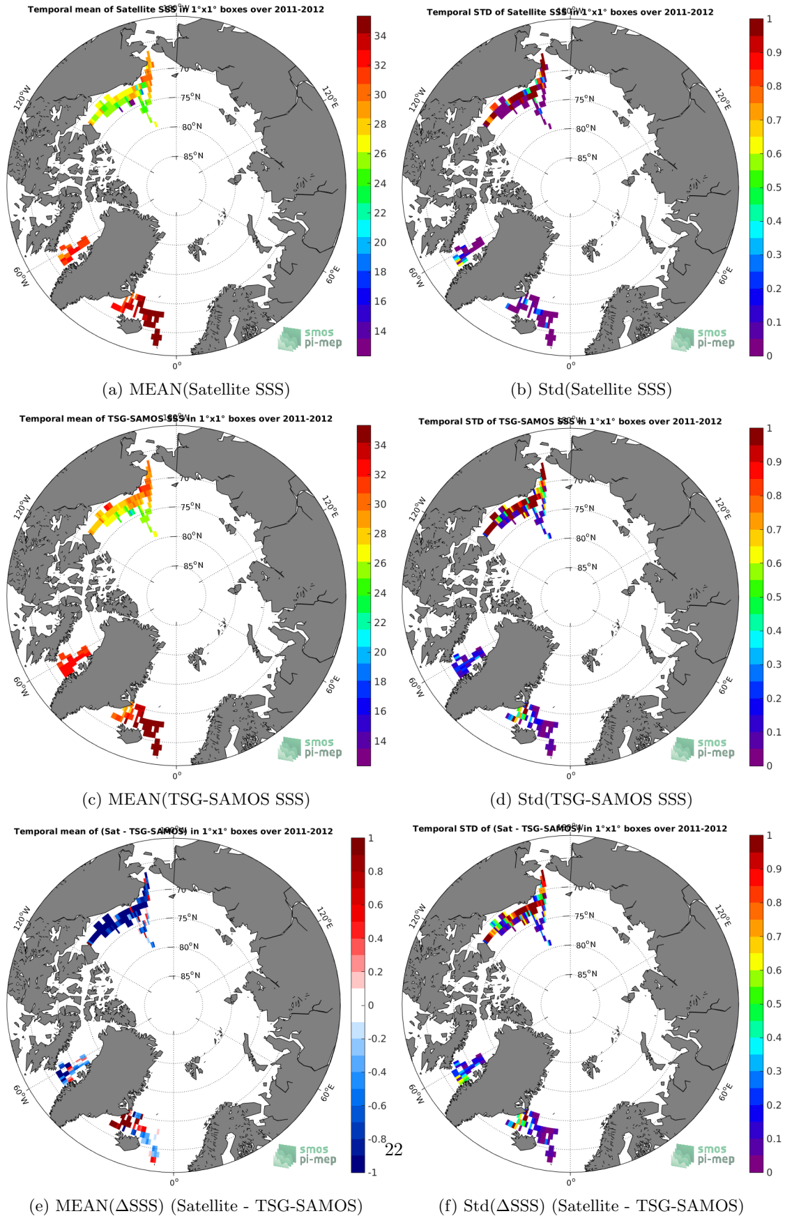
Figure 6: Temporal mean (left) and Std (right) of SSS from Aquarius-L3-OR-V5-7DAY-RUNNING-RAIN-MASK-1DEG (top), TSG-SAMOS (middle), and of \Delta SSS (Satellite - TSG-SAMOS). Only match-up pairs are used to generate these maps.
