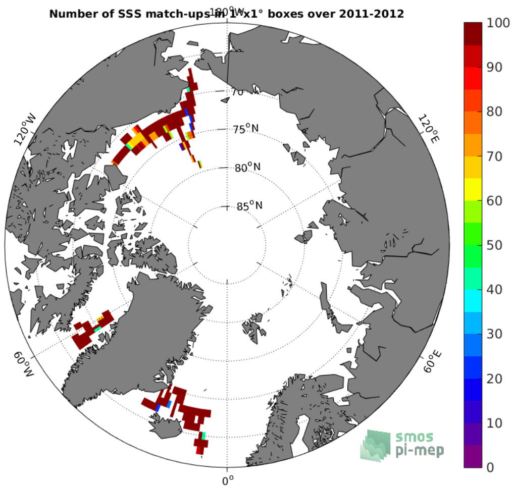
Figure 4: Number of SSS match-ups between TSG-SAMOS SSS and the Aquarius-L3-OR-V5-7DAY-RUNNING-RAIN-MASK-1DEG SSS product for the Arctic Ocean Pi-MEP region over 1^\circ \times 1^\circ boxes and for the full satellite product period.
