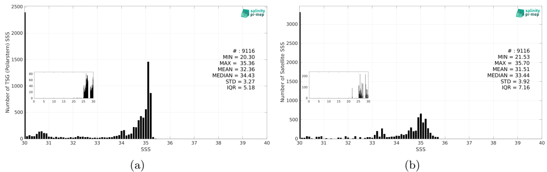
Figure 3: Histograms of SSS from TSG (Polarstern) (a) and Aquarius SSS L3 OR v5 - 7-Day running - Rain mask (NASA-GSFC) (b) considering all match-up pairs per bins of 0.1 over the Arctic Ocean Pi-MEP region and for the full satellite product period.
