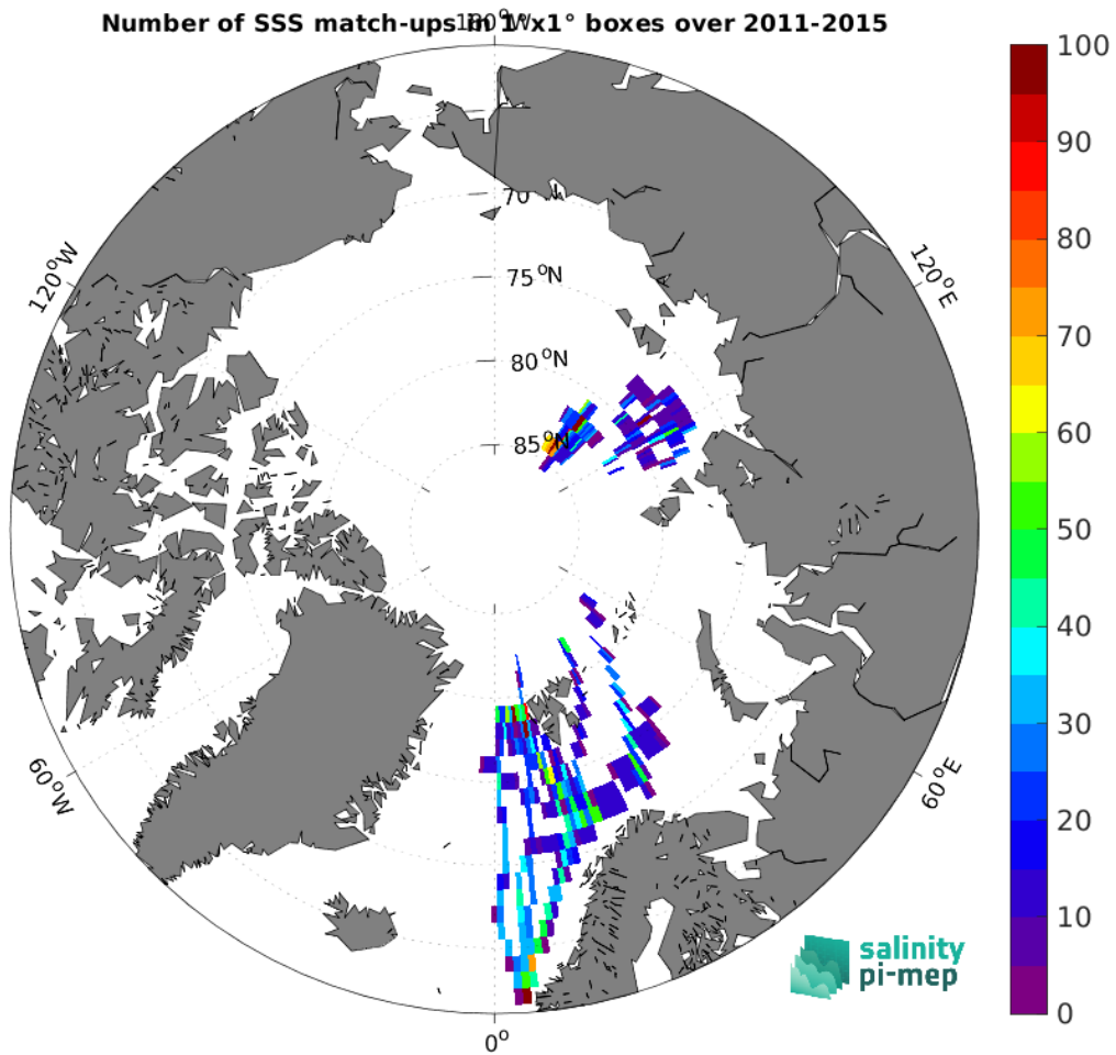
Figure 5: Number of SSS match-ups between TSG (Polarstern) SSS and the Aquarius SSS L3 OR v5 - 7-Day running - Rain mask (NASA-GSFC) SSS product for the Arctic Ocean Pi-MEP region over 1°×1° boxes and for the full satellite product period.
