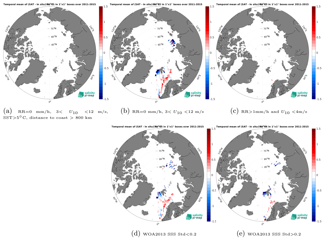
Figure 14: Temporal mean gridded over spatial boxes of size 1^\circ \times 1^\circ of \Delta\text{SSS} (Aquarius SSS L3 OR v5 - 7-Day running - Rain mask (NASA-GSFC) - TSG (Polarstern)) for 5 different subdatasets corresponding to:RR=0 mm/h, 3 < U_{10} < 12 m/s, SST>5°C, distance to coast > 800 km (a), RR=0 mm/h, 3 < U_{10} < 12 m/s (b), RR>1mm/h and U_{10} < 4 m/s (c), WOA2013 SSS Std<0.2 (d), WOA2013 SSS Std>0.2 (e).
