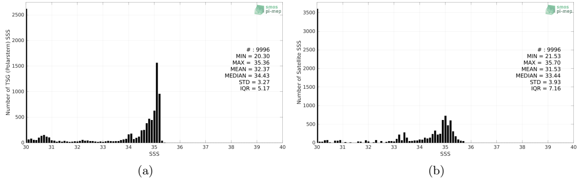
Figure 2: Histograms of SSS from TSG (Polarstern) (a) and Aquarius SSS L3 OR v5 - 7-Day running - Rain mask (NASA-GSFC) (b) considering all match-up pairs per bins of 0.1 over the Arctic Ocean Pi-MEP region and for the full satellite product period.
