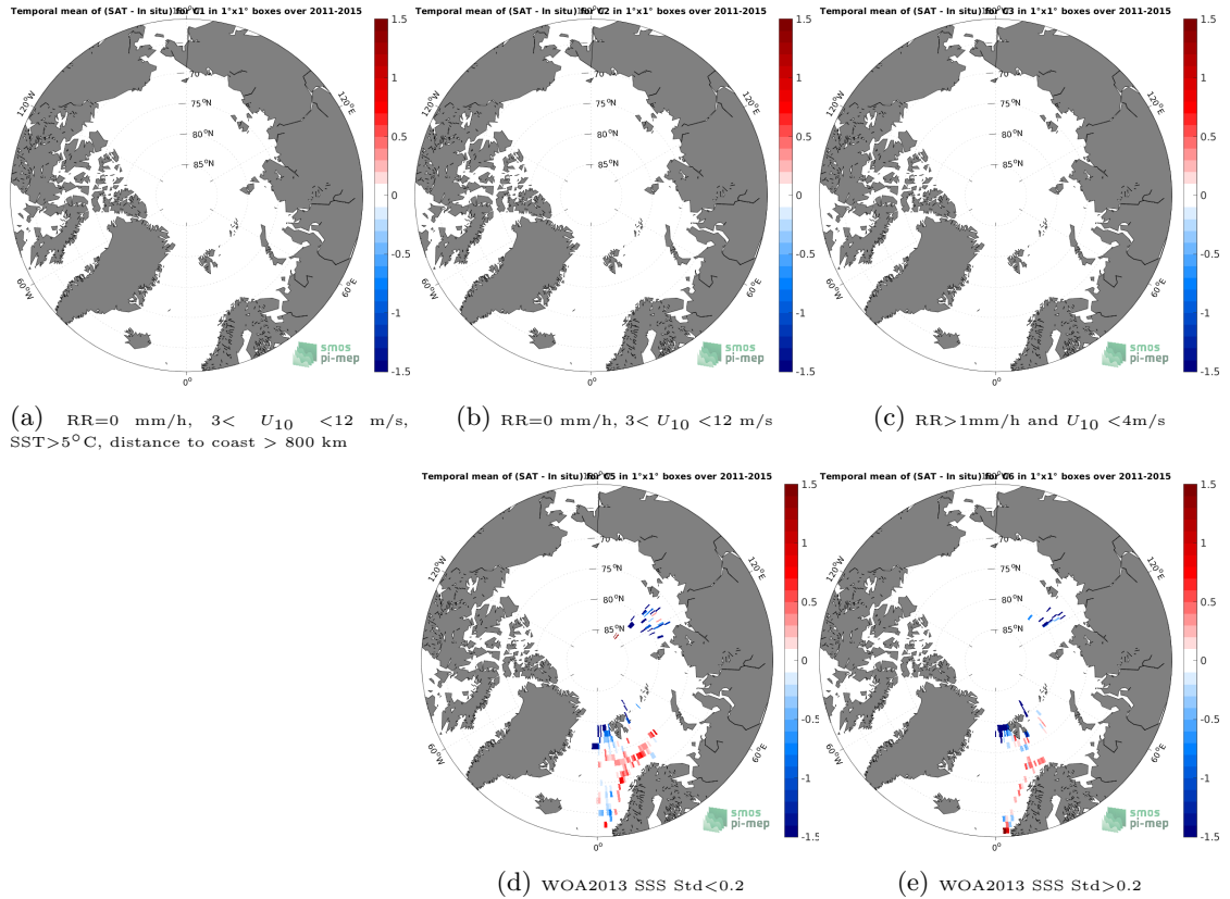
Figure 12: Temporal mean gridded over spatial boxes of size 1^{\circ}\times 1^{\circ} of \Delta\text{SSS} (Aquarius SSS L3 OR v5 - 7-Day running - Rain mask (NASA-GSFC) - TSG (Polarstern)) for 5 different subdatasets corresponding to:RR=0 mm/h, 3 < U_{10} < 12 m/s, SST > 5^{\circ}\text{C} , distance to coast > 800 km (a), RR=0 mm/h, 3 < U_{10} < 12 m/s (b), RR > 1 mm/h and U_{10} < 4 m/s (c), WOA2013 SSS Std < 0.2 (d), WOA2013 SSS Std > 0.2 (e).
