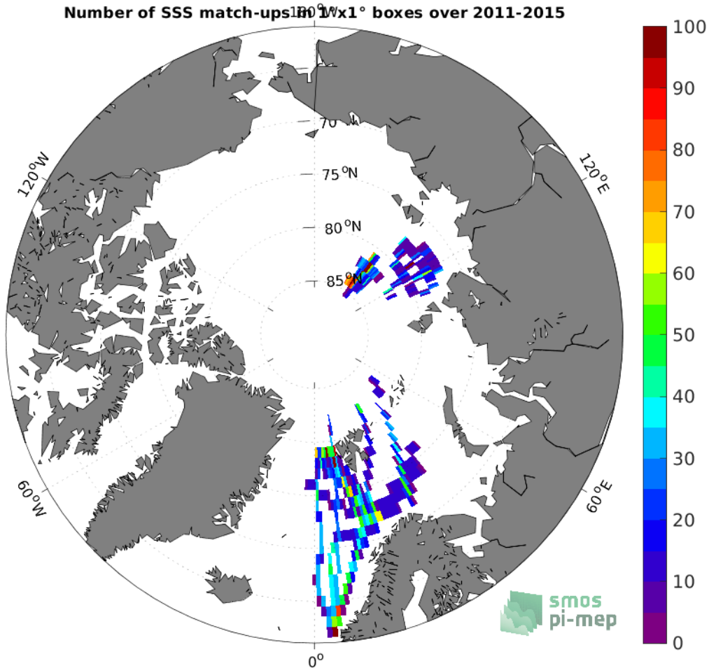
Figure 4: Number of SSS match-ups between TSG (Polarstern) SSS and the Aquarius SSS L3 OR v5 - 7-Day running - Rain mask (NASA-GSFC) SSS product for the Arctic Ocean Pi-MEP region over 1^\circ \times 1^\circ boxes and for the full satellite product period.
