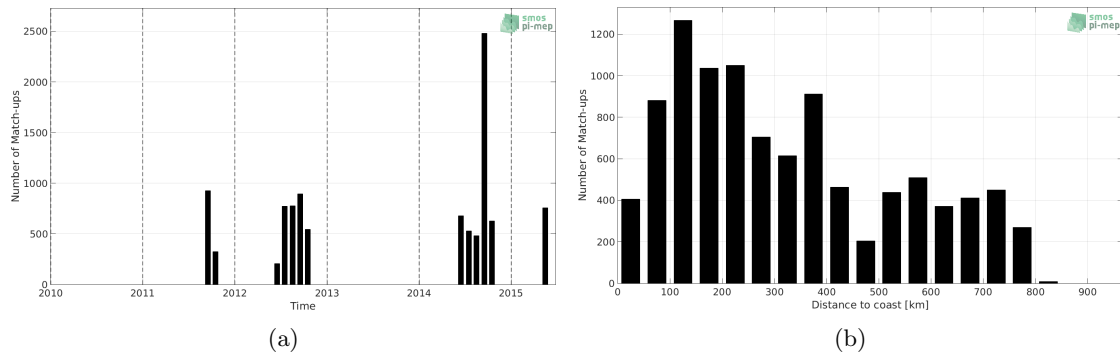
Figure 1: Number of match-ups between TSG-POLARSTERN and Aquarius-L3-OR-V5-7DAY-RUNNING-RAIN-MASK-1DEG SSS as a function of time (a) and as function of the distance to coast (b) over the Arctic Ocean Pi-MEP region and for the full satellite product period.
