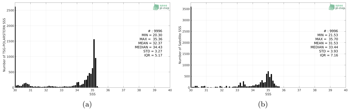
Figure 2: Histograms of SSS from TSG-POLARSTERN (a) and Aquarius-L3-OR-V5-7DAY-RUNNING-RAIN-MASK-1DEG (b) considering all match-up pairs per bins of 0.1 over the Arctic Ocean Pi-MEP region and for the full satellite product period.
