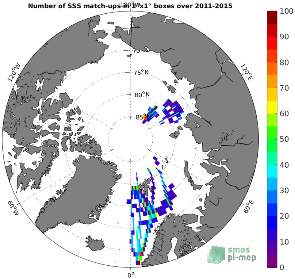
Figure 4: Number of SSS match-ups between TSG-POLARSTERN SSS and the Aquarius-L3-OR-V5-7DAY-RUNNING-RAIN-MASK-1DEG SSS product for the Arctic Ocean Pi-MEP region over 1°x1° boxes and for the full satellite product period.
