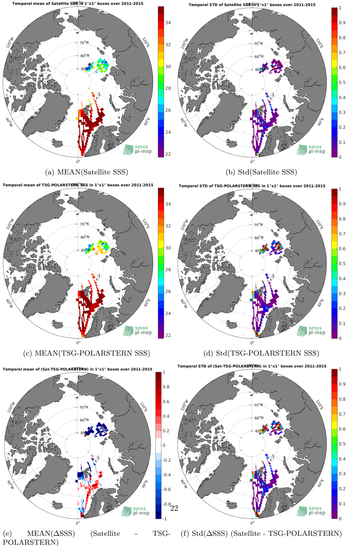
Figure 6: Temporal mean (left) and Std (right) of SSS from Aquarius-L3-OR-V5-7DAY-RUNNING-RAIN-MASK-1DEG (top), TSG-POLARSTERN (middle), and of \Delta SSS (Satellite - TSG-POLARSTERN). Only match-up pairs are used to generate these maps.
