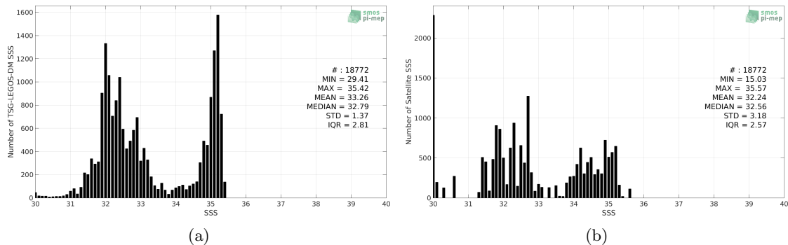
Figure 2: Histograms of SSS from TSG-LEGOS-DM (a) and Aquarius-L3-OR-V5-7DAY-RUNNING-RAIN-MASK-1DEG (b) considering all match-up pairs per bins of 0.1 over the Arctic Ocean Pi-MEP region and for the full satellite product period.
