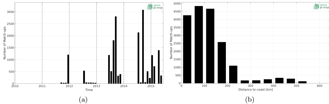
Figure 1: Number of match-ups between TSG-LEGOS-DM and Aquarius-L3-OR-V5-7DAY-RUNNING-RAIN-MASK-1DEG SSS as a function of time (a) and as function of the distance to coast (b) over the Arctic Ocean Pi-MEP region and for the full satellite product period.
