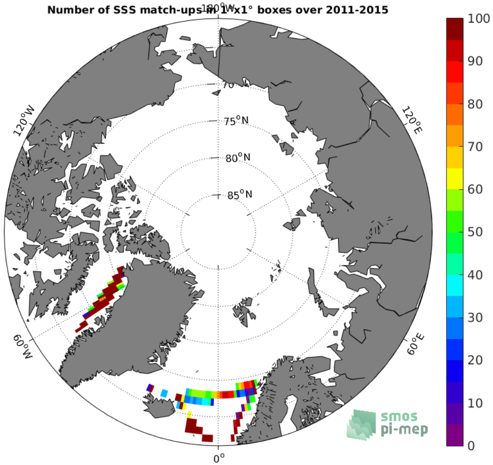
Figure 4: Number of SSS match-ups between TSG-LEGOS-DM SSS and the Aquarius-L3-OR-V5-7DAY-RUNNING-RAIN-MASK-1DEG SSS product for the Arctic Ocean Pi-MEP region over 1°x1° boxes and for the full satellite product period.
