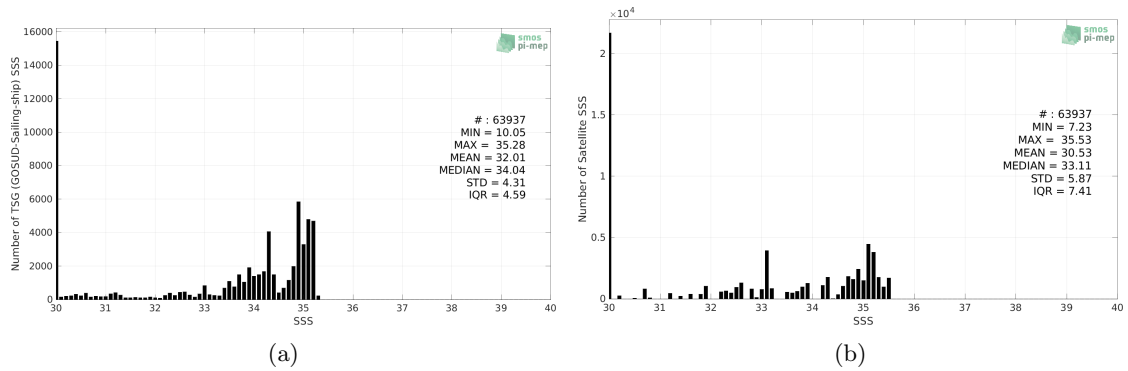
Figure 2: Histograms of SSS from TSG (GOSUD-Sailing-ship) (a) and Aquarius SSS L3 OR v5 - 7-Day running - Rain mask (NASA-GSFC) (b) considering all match-up pairs per bins of 0.1 over the Arctic Ocean Pi-MEP region and for the full satellite product period.
