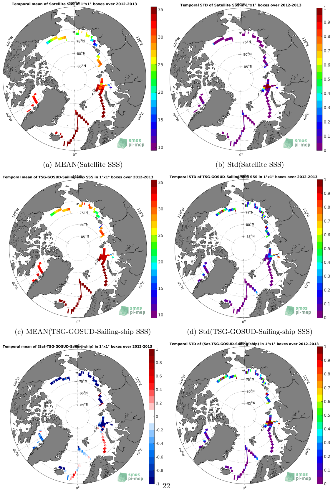
Figure 6: Temporal mean (left) and Std (right) of SSS from Aquarius-L3-OR-V5-7DAY-RUNNING-RAIN-MASK-1DEG (top), TSG-GOSUD-Sailing-ship (middle), and of \Delta SSS (Satellite - TSG-GOSUD-Sailing-ship). Only match-up pairs are used to generate these maps.
