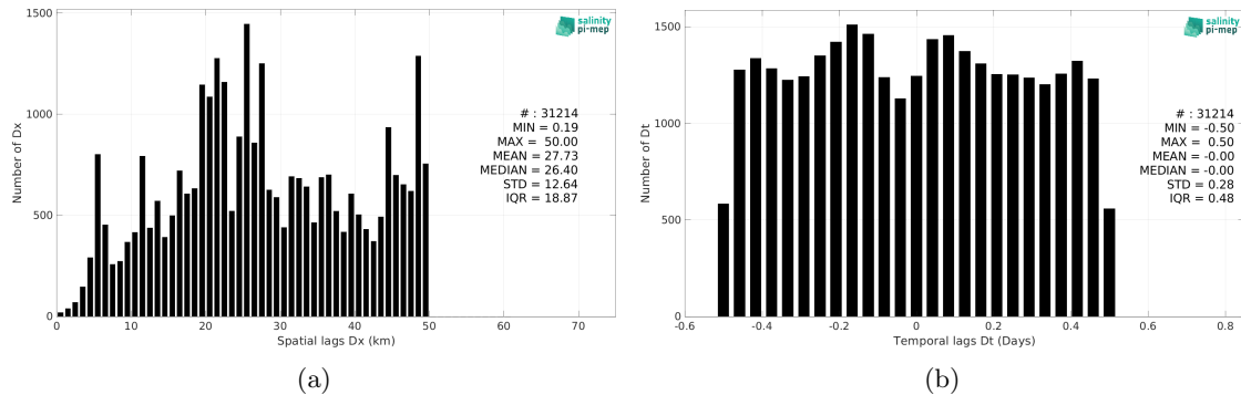
Figure 6: Histograms of the spatial (a) and temporal (b) lags between the location/time of the TSG (Amundsen) measurement and the date of the corresponding Aquarius SSS L3 OR v5 - 7-Day running - Rain mask (NASA-GSFC) SSS pixel.
