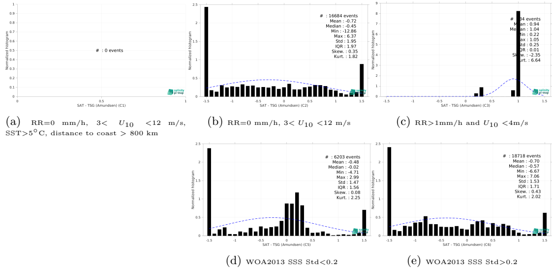
Figure 15: Normalized histogram of \Delta SSS (Aquarius SSS L3 OR v5 - 7-Day running - Rain mask (NASA-GSFC) - TSG (Amundsen)) for 5 different subdatasets corresponding to: RR=0 mm/h, 3 < U_{10} < 12 m/s, SST > 5°C, distance to coast > 800 km (a), RR=0 mm/h, 3 < U_{10} < 12 m/s (b), RR > 1mm/h and U_{10} < 4 m/s (c), WOA2013 SSS Std < 0.2 (d), WOA2013 SSS Std > 0.2 (e).
