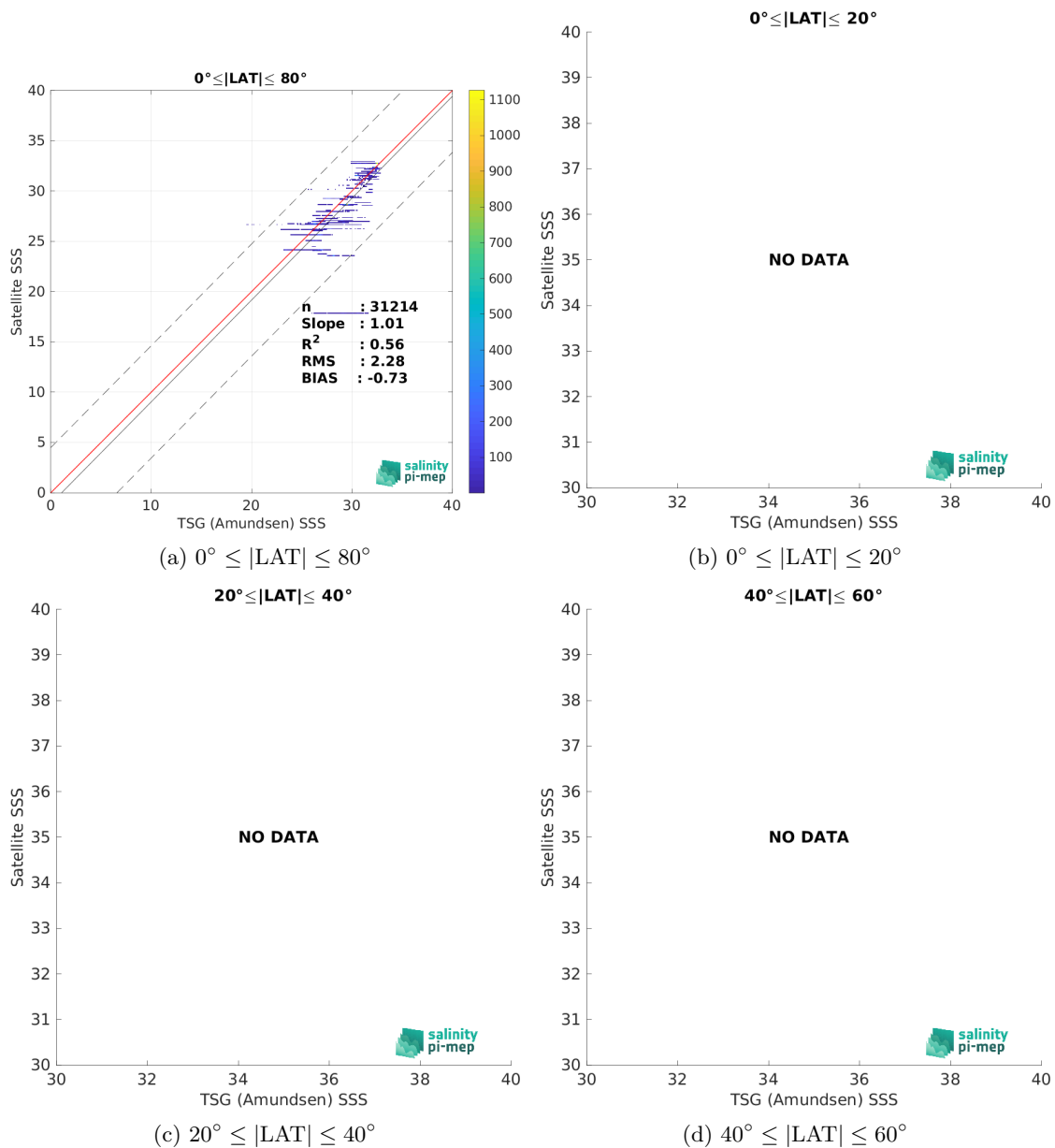
Figure 10: Contour maps of the concentration of Aquarius SSS L3 OR v5 - 7-Day running - Rain mask (NASA-GSFC) SSS (y-axis) versus TSG (Amundsen) SSS (x-axis) at match-up pairs for different latitude bands. For each plot, the red line shows x=y . The black thin and dashed lines indicate a linear fit through the data cloud and the \pm 95\% confidence levels, respectively. The number match-up pairs n , the slope and R^2 coefficient of the linear fit, the root mean square (RMS) and the mean bias between satellite and in situ data are indicated for each latitude band in each plots.
