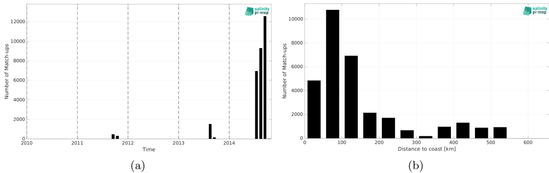
Figure 2: Number of match-ups between TSG (Amundsen) and Aquarius SSS L3 OR v5 - 7-Day running - Rain mask (NASA-GSFC) SSS as a function of time (a) and as function of the distance to coast (b) over the Arctic Ocean Pi-MEP region and for the full satellite product period.
