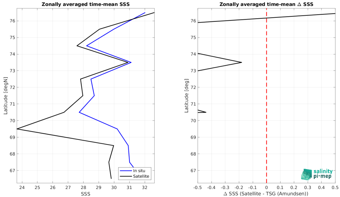
Figure 9: Left panel: Zonal mean SSS from Aquarius SSS L3 OR v5 - 7-Day running - Rain mask (NASA-GSFC) satellite product (black) and from TSG (Amundsen) (blue). Right panel: Zonal mean of \Delta SSS (Satellite - TSG (Amundsen)) for all the collected Pi-MEP match-up pairs estimated over the full satellite product period.
