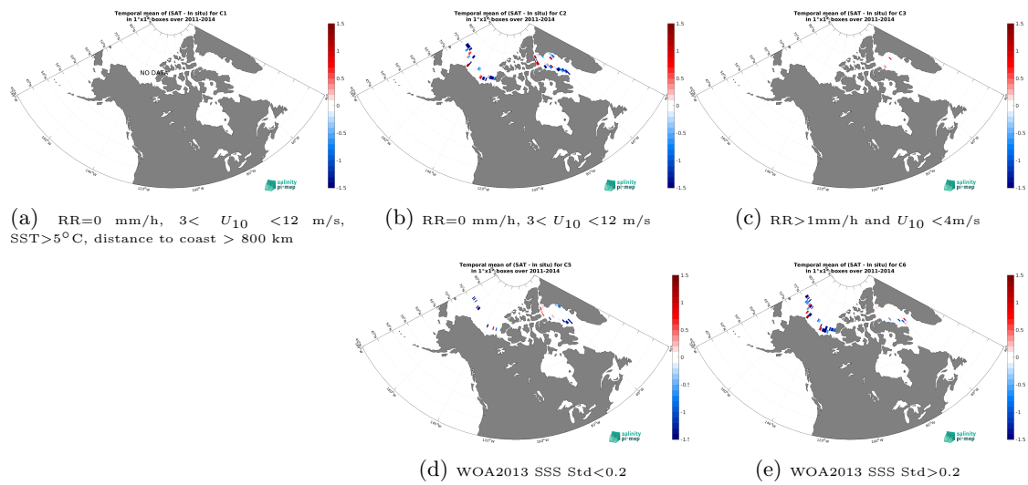
Figure 14: Temporal mean gridded over spatial boxes of size 1^\circ \times 1^\circ of \Delta SSS (Aquarius SSS L3 OR v5 - 7-Day running - Rain mask (NASA-GSFC) - TSG (Amundsen)) for 5 different subdatasets corresponding to:RR=0 mm/h, 3 < U_{10} < 12 m/s, SST > 5^\circ\text{C} , distance to coast > 800 km (a), RR=0 mm/h, 3 < U_{10} < 12 m/s (b), RR > 1 mm/h and U_{10} < 4 m/s (c), WOA2013 SSS Std < 0.2 (d), WOA2013 SSS Std > 0.2 (e).
