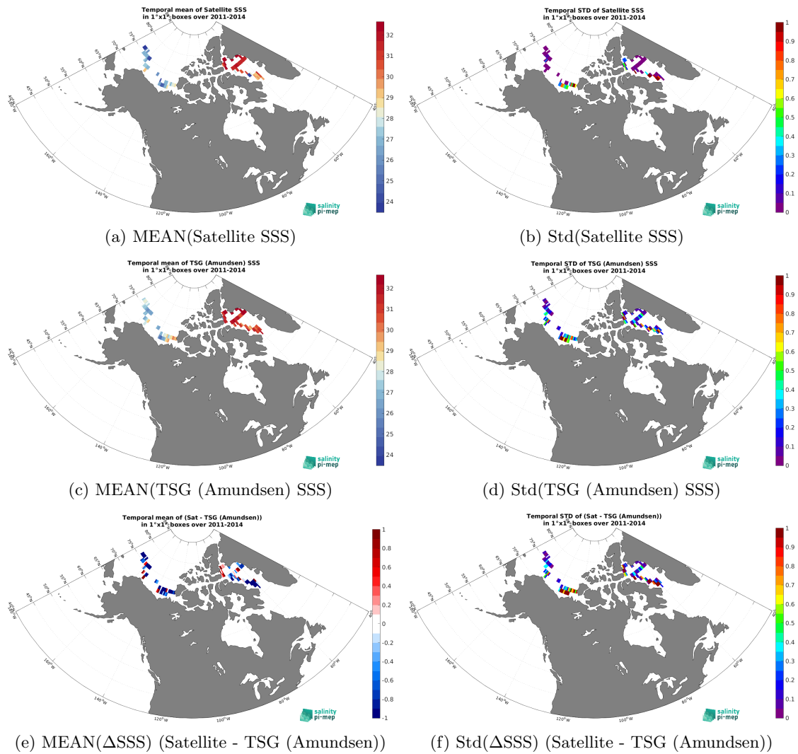
Figure 7: Temporal mean (left) and Std (right) of SSS from Aquarius SSS L3 OR v5 - 7-Day running - Rain mask (NASA-GSFC) (top), TSG (Amundsen) (middle), and of \Delta SSS (Satellite - TSG (Amundsen)). Only match-up pairs are used to generate these maps.
