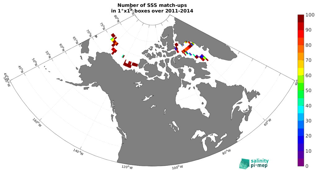
Figure 5: Number of SSS match-ups between TSG (Amundsen) SSS and the Aquarius SSS L3 OR v5 - 7-Day running - Rain mask (NASA-GSFC) SSS product for the Arctic Ocean Pi-MEP region over 1°×1° boxes and for the full satellite product period.
