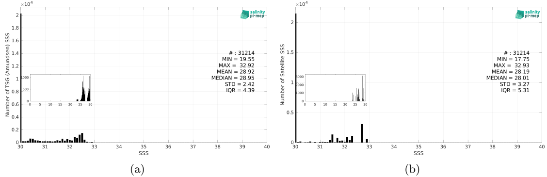
Figure 3: Histograms of SSS from TSG (Amundsen) (a) and Aquarius SSS L3 OR v5 - 7-Day running - Rain mask (NASA-GSFC) (b) considering all match-up pairs per bins of 0.1 over the Arctic Ocean Pi-MEP region and for the full satellite product period.
