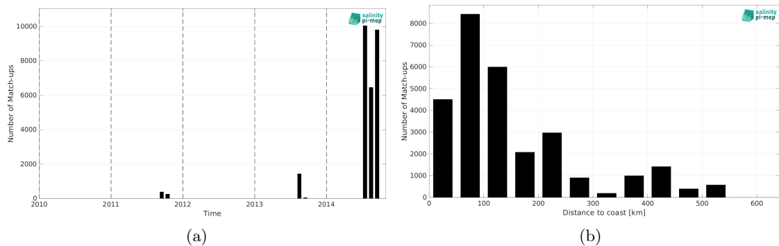
Figure 1: Number of match-ups between TSG (Amundsen) and Aquarius SSS L3 OR v5 - 7-Day running - Rain mask (NASA-GSFC) SSS as a function of time (a) and as function of the distance to coast (b) over the Arctic Ocean Pi-MEP region and for the full satellite product period.
