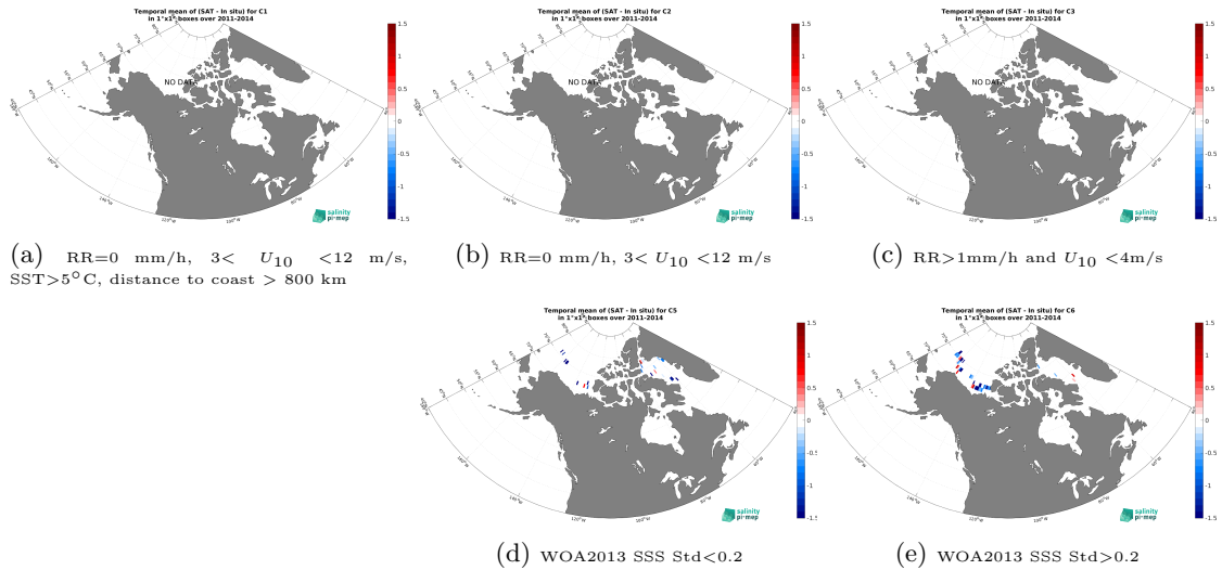
Figure 12: Temporal mean gridded over spatial boxes of size 1^{\circ}\times 1^{\circ} of \Delta\text{SSS} (Aquarius SSS L3 OR v5 - 7-Day running - Rain mask (NASA-GSFC) - TSG (Amundsen)) for 5 different subdatasets corresponding to:RR=0 mm/h, 3 < U_{10} < 12 m/s, SST >5^{\circ}\text{C} , distance to coast > 800 km (a), RR=0 mm/h, 3 < U_{10} < 12 m/s (b), RR >1 mm/h and U_{10} < 4 m/s (c), WOA2013 SSS Std <0.2 (d), WOA2013 SSS Std >0.2 (e).
