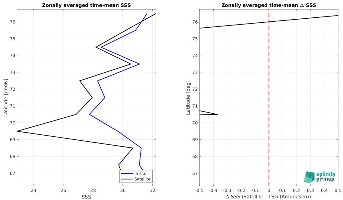
Figure 8: Left panel: Zonal mean SSS from Aquarius SSS L3 OR v5 - 7-Day running - Rain mask (NASA-GSFC) satellite product (black) and from TSG (Amundsen) (blue). Right panel: Zonal mean of \Delta SSS (Satellite - TSG (Amundsen)) for all the collected Pi-MEP match-up pairs estimated over the full satellite product period.
