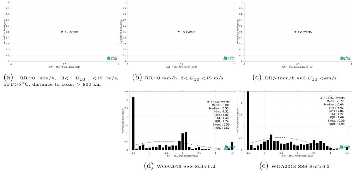
Figure 13: Normalized histogram of \Delta SSS (Aquarius SSS L3 OR v5 - 7-Day running - Rain mask (NASA-GSFC) - TSG (Amundsen)) for 5 different subdatasets corresponding to: RR=0 mm/h, 3 < U_{10} < 12 m/s, SST>5°C, distance to coast > 800 km (a), RR=0 mm/h, 3 < U_{10} < 12 m/s (b), RR>1mm/h and U_{10} < 4 m/s (c), WOA2013 SSS Std<0.2 (d), WOA2013 SSS Std>0.2 (e).
