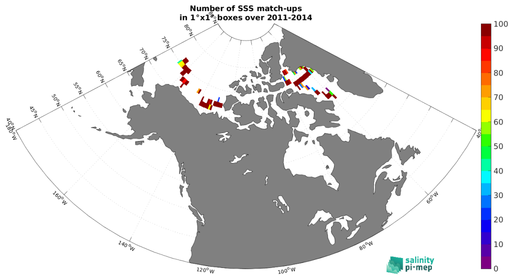
Figure 4: Number of SSS match-ups between TSG (Amundsen) SSS and the Aquarius SSS L3 OR v5 - 7-Day running - Rain mask (NASA-GSFC) SSS product for the Arctic Ocean Pi-MEP region over 1^\circ \times 1^\circ boxes and for the full satellite product period.
