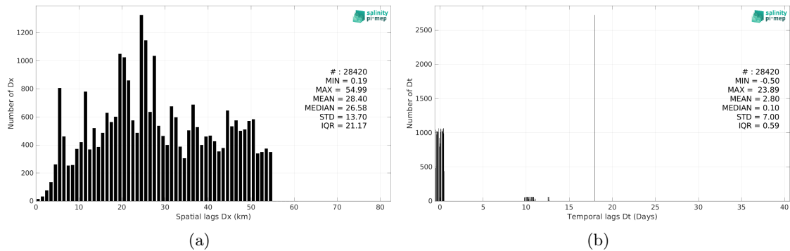
Figure 5: Histograms of the spatial (a) and temporal (b) lags between the location/time of the TSG (Amundsen) measurement and the date of the corresponding Aquarius SSS L3 OR v5 - 7-Day running - Rain mask (NASA-GSFC) SSS pixel.
