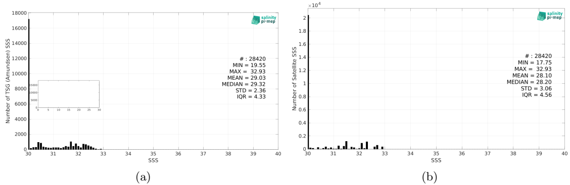
Figure 2: Histograms of SSS from TSG (Amundsen) (a) and Aquarius SSS L3 OR v5 - 7-Day running - Rain mask (NASA-GSFC) (b) considering all match-up pairs per bins of 0.1 over the Arctic Ocean Pi-MEP region and for the full satellite product period.
