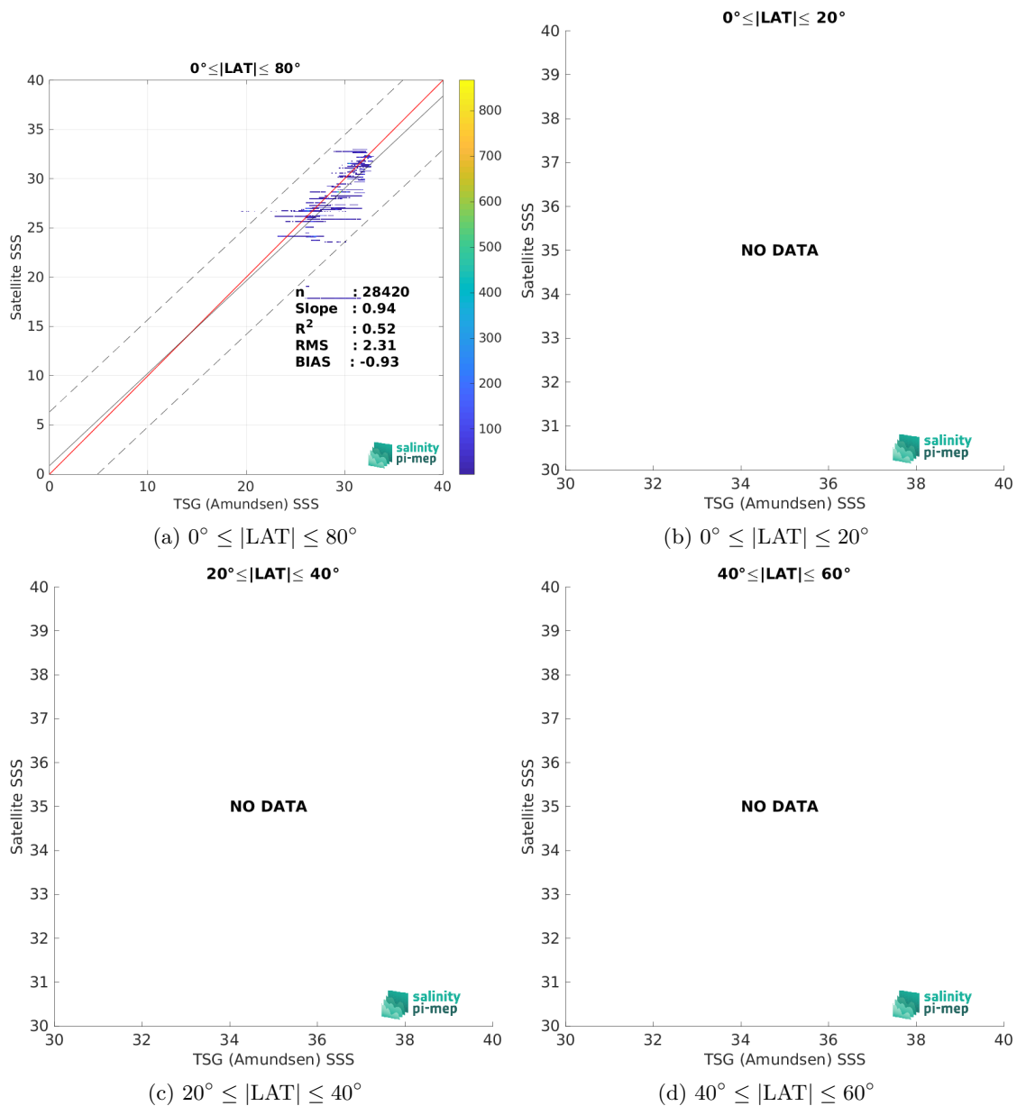
Figure 9: Contour maps of the concentration of Aquarius SSS L3 OR v5 - 7-Day running - Rain mask (NASA-GSFC) SSS (y-axis) versus TSG (Amundsen) SSS (x-axis) at match-up pairs for different latitude bands. For each plot, the red line shows x=y . The black thin and dashed lines indicate a linear fit through the data cloud and the \pm 95\% confidence levels, respectively. The number match-up pairs n , the slope and R^2 coefficient of the linear fit, the root mean square (RMS) and the mean bias between satellite and in situ data are indicated for each latitude band in each plots.
