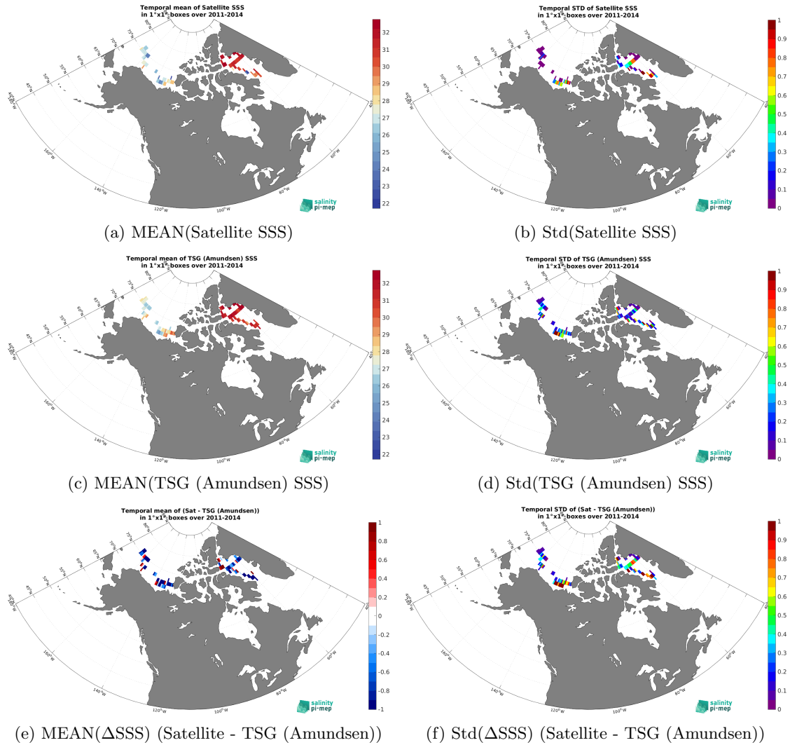
Figure 6: Temporal mean (left) and Std (right) of SSS from Aquarius SSS L3 OR v5 - 7-Day running - Rain mask (NASA-GSFC) (top), TSG (Amundsen) (middle), and of \Delta SSS (Satellite - TSG (Amundsen)). Only match-up pairs are used to generate these maps.
