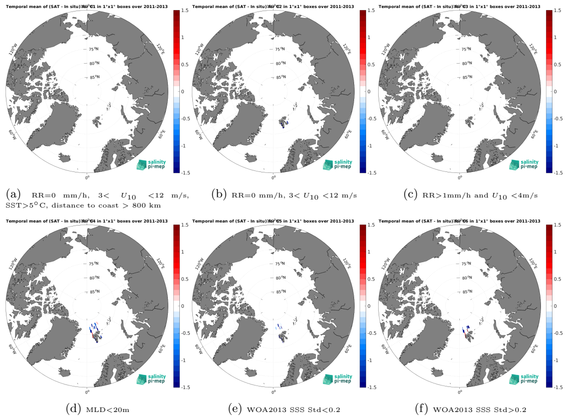
Figure 14: Temporal mean gridded over spatial boxes of size 1^\circ \times 1^\circ of \Delta SSS (Aquarius SSS L3 OR v5 - 7-Day running - Rain mask (NASA-GSFC) - Marine mammals) for 6 different subdatasets corresponding to:RR=0 mm/h, 3 < U_{10} < 12 m/s, SST >5^\circ C, distance to coast > 800 km (a), RR=0 mm/h, 3 < U_{10} < 12 m/s (b), RR >1 mm/h and U_{10} < 4 m/s (c),MLD <20 m (d),WOA2013 SSS Std <0.2 (e),WOA2013 SSS Std >0.2 (f).
