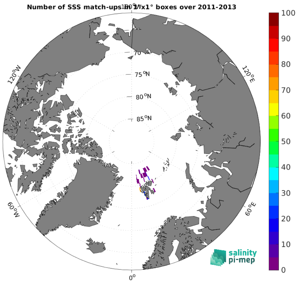
Figure 5: Number of SSS match-ups between Marine mammals SSS and the Aquarius SSS L3 OR v5 - 7-Day running - Rain mask (NASA-GSFC) SSS product for the Arctic Ocean Pi-MEP region over 1^\circ \times 1^\circ boxes and for the full satellite product period.
