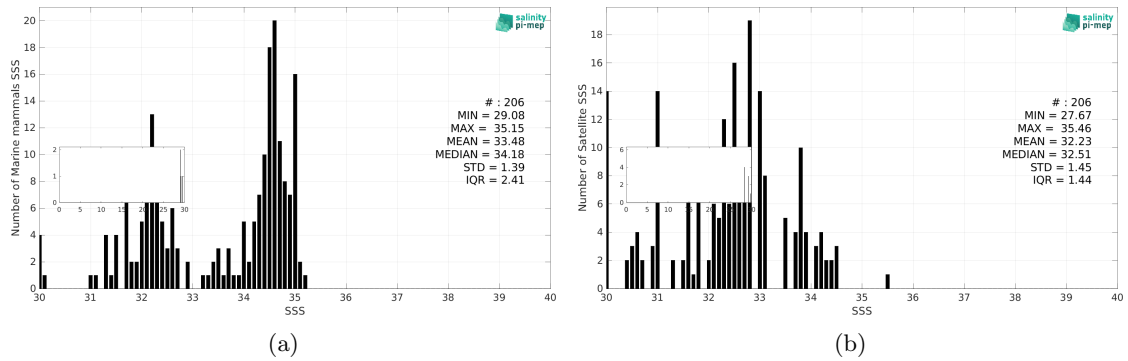
Figure 3: Histograms of SSS from Marine mammals (a) and Aquarius SSS L3 OR v5 - 7-Day running - Rain mask (NASA-GSFC) (b) considering all match-up pairs per bins of 0.1 over the Arctic Ocean Pi-MEP region and for the full satellite product period.
