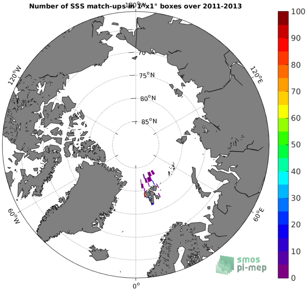
Figure 4: Number of SSS match-ups between Sea mammals SSS and the Aquarius-L3-OR-V5-7DAY-RUNNING-RAIN-MASK-1DEG SSS product for the Arctic Ocean Pi-MEP region over 1°x1° boxes and for the full satellite product period.
