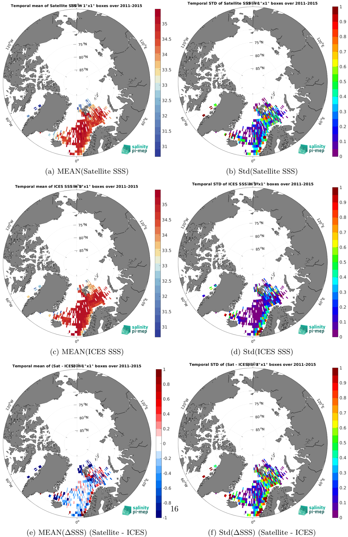
Figure 7: Temporal mean (left) and Std (right) of SSS from Aquarius SSS L3 OR v5 - 7-Day running - Rain mask (NASA-GSFC) (top), ICES (middle), and of \Delta SSS (Satellite - ICES). Only match-up pairs are used to generate these maps.
