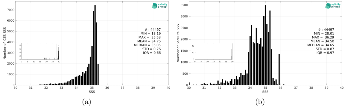
Figure 3: Histograms of SSS from ICES (a) and Aquarius SSS L3 OR v5 - 7-Day running - Rain mask (NASA-GSFC) (b) considering all match-up pairs per bins of 0.1 over the Arctic Ocean Pi-MEP region and for the full satellite product period.
