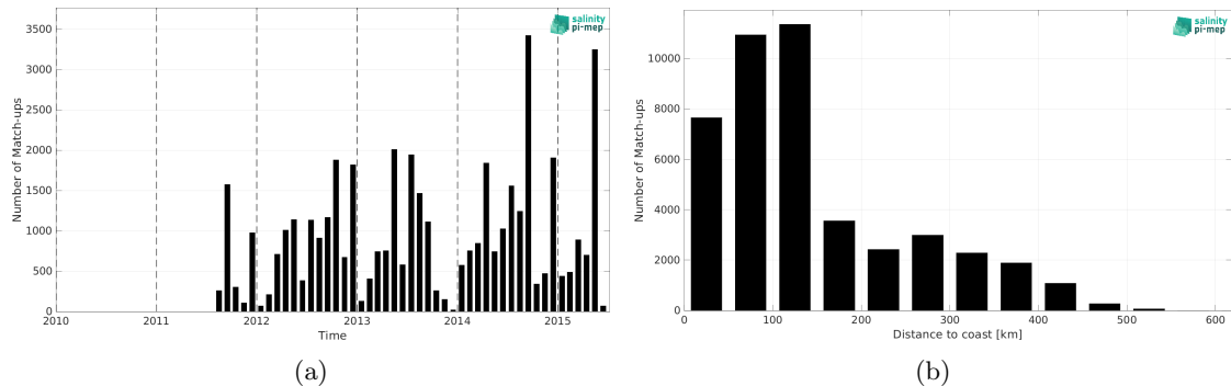
Figure 2: Number of match-ups between ICES and Aquarius SSS L3 OR v5 - 7-Day running - Rain mask (NASA-GSFC) SSS as a function of time (a) and as function of the distance to coast (b) over the Arctic Ocean Pi-MEP region and for the full satellite product period.
