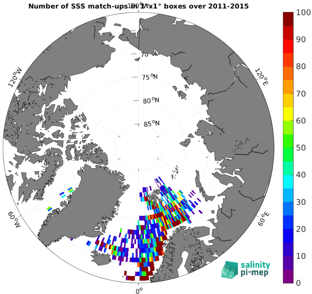
Figure 5: Number of SSS match-ups between ICES SSS and the Aquarius SSS L3 OR v5 - 7-Day running - Rain mask (NASA-GSFC) SSS product for the Arctic Ocean Pi-MEP region over 1^\circ \times 1^\circ boxes and for the full satellite product period.
