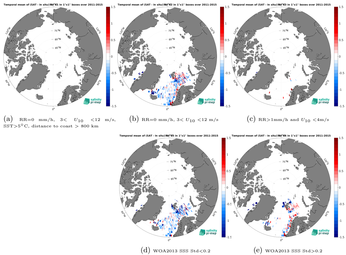
Figure 14: Temporal mean gridded over spatial boxes of size 1^\circ \times 1^\circ of \Delta\text{SSS} (Aquarius SSS L3 OR v5 - 7-Day running - Rain mask (NASA-GSFC) - ICES) for 5 different subdatasets corresponding to: RR=0 mm/h, 3 < U_{10} < 12 m/s, SST > 5°C, distance to coast > 800 km (a), RR=0 mm/h, 3 < U_{10} < 12 m/s (b), RR > 1mm/h and U_{10} < 4 m/s (c), WOA2013 SSS Std < 0.2 (d), WOA2013 SSS Std > 0.2 (e).
