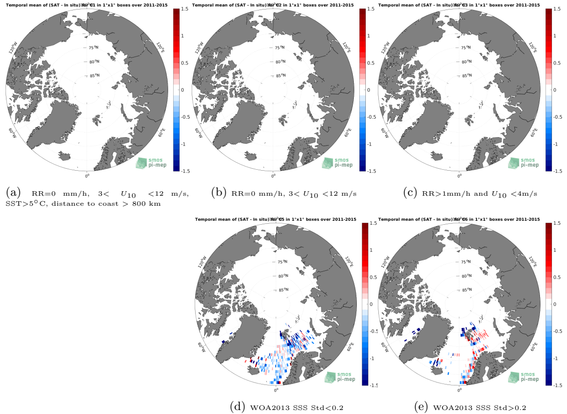
Figure 12: Temporal mean gridded over spatial boxes of size 1^{\circ}\times 1^{\circ} of \Delta\text{SSS} (Aquarius SSS L3 OR v5 - 7-Day running - Rain mask (NASA-GSFC) - ICES) for 5 different subdatasets corresponding to:RR=0 mm/h, 3 < U_{10} < 12 m/s, SST >5^{\circ}\text{C} , distance to coast > 800 km (a), RR=0 mm/h, 3 < U_{10} < 12 m/s (b), RR >1 mm/h and U_{10} < 4 m/s (c), WOA2013 SSS Std <0.2 (d), WOA2013 SSS Std >0.2 (e).
