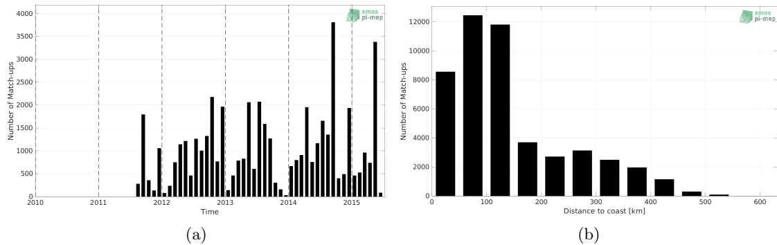
Figure 1: Number of match-ups between ICES and Aquarius SSS L3 OR v5 - 7-Day running - Rain mask (NASA-GSFC) SSS as a function of time (a) and as function of the distance to coast (b) over the Arctic Ocean Pi-MEP region and for the full satellite product period.
