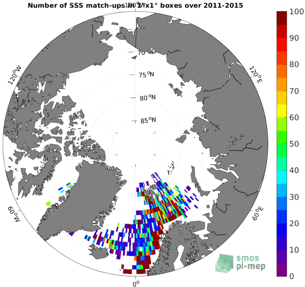
Figure 4: Number of SSS match-ups between ICES SSS and the Aquarius SSS L3 OR v5 - 7-Day running - Rain mask (NASA-GSFC) SSS product for the Arctic Ocean Pi-MEP region over 1^\circ \times 1^\circ boxes and for the full satellite product period.
