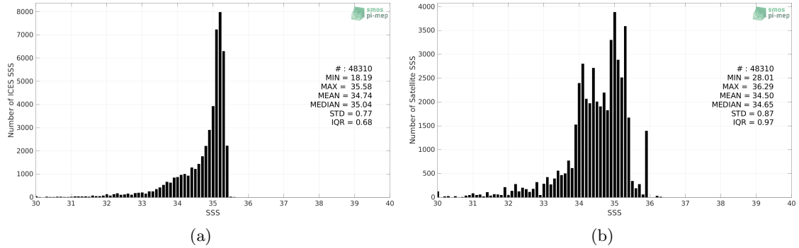
Figure 2: Histograms of SSS from ICES (a) and Aquarius SSS L3 OR v5 - 7-Day running - Rain mask (NASA-GSFC) (b) considering all match-up pairs per bins of 0.1 over the Arctic Ocean Pi-MEP region and for the full satellite product period.
