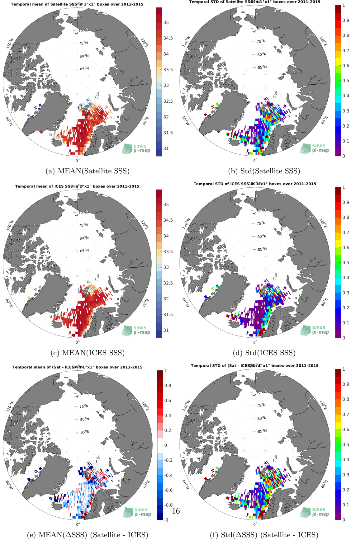
Figure 6: Temporal mean (left) and Std (right) of SSS from Aquarius SSS L3 OR v5 - 7-Day running - Rain mask (NASA-GSFC) (top), ICES (middle), and of \Delta SSS (Satellite - ICES). Only match-up pairs are used to generate these maps.
