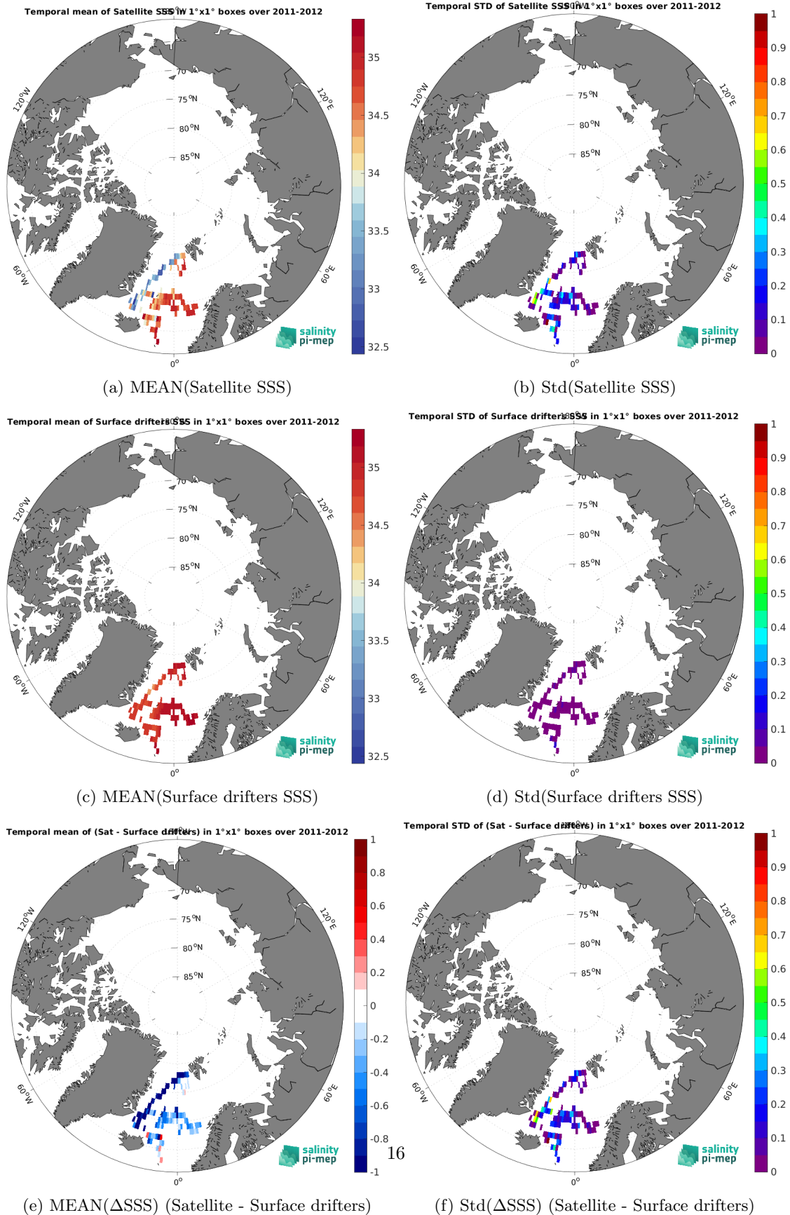
Figure 6: Temporal mean (left) and Std (right) of SSS from Aquarius SSS L3 OR v5 - 7-Day running - Rain mask (NASA-GSFC) (top), Surface drifters (middle), and of \Delta SSS (Satellite - Surface drifters). Only match-up pairs are used to generate these maps.
