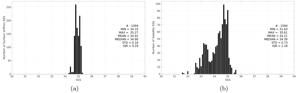
Figure 3: Histograms of SSS from Surface drifters (a) and Aquarius SSS L3 OR v5 - 7-Day running - Rain mask (NASA-GSFC) (b) considering all match-up pairs per bins of 0.1 over the Arctic Ocean Pi-MEP region and for the full satellite product period.
