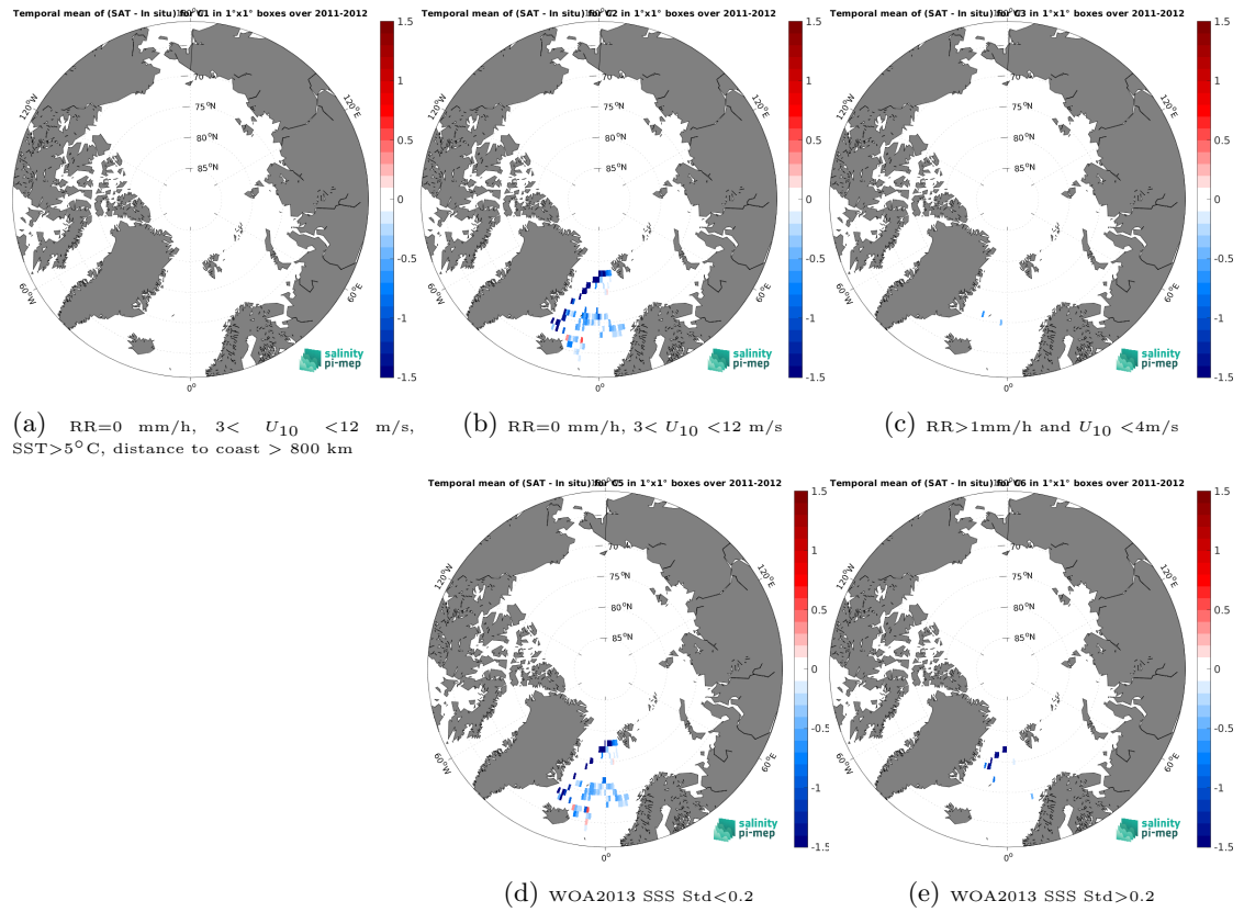
Figure 13: Temporal mean gridded over spatial boxes of size 1^\circ \times 1^\circ of \Delta SSS (Aquarius SSS L3 OR v5 - 7-Day running - Rain mask (NASA-GSFC) - Surface drifters) for 5 different subdatasets corresponding to: RR=0 mm/h, 3 < U_{10} < 12 m/s, SST >5^\circ\text{C} , distance to coast > 800 km (a), RR=0 mm/h, 3 < U_{10} < 12 m/s (b), RR >1 mm/h and U_{10} < 4 m/s (c), WOA2013 SSS Std <0.2 (d), WOA2013 SSS Std >0.2 (e).
