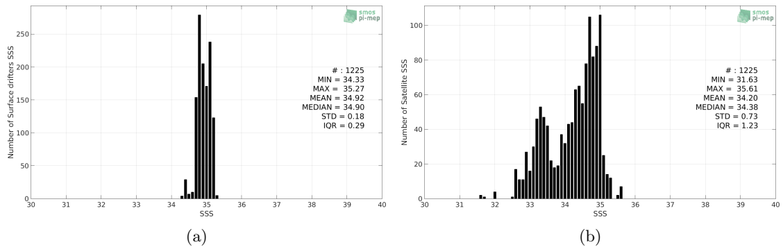
Figure 2: Histograms of SSS from Surface drifters (a) and Aquarius-L3-OR-V5-7DAY-RUNNING-RAIN-MASK-1DEG (b) considering all match-up pairs per bins of 0.1 over the Arctic Ocean Pi-MEP region and for the full satellite product period.
