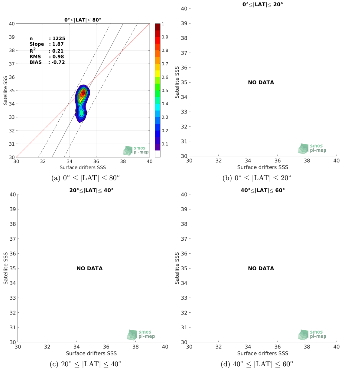
Figure 8: Contour maps of the concentration of Aquarius-L3-OR-V5-7DAY-RUNNING-RAIN-MASK-1DEG SSS (y-axis) versus Surface drifters SSS (x-axis) at match-up pairs for different latitude bands. For each plot, the red line shows x=y . The black thin and dashed lines indicate a linear fit through the data cloud and the \pm 95\% confidence levels, respectively. The number match-up pairs n , the slope and R^2 coefficient of the linear fit, the root mean square (RMS) and the mean bias between satellite and in situ data are indicated for each latitude band in each plots.
