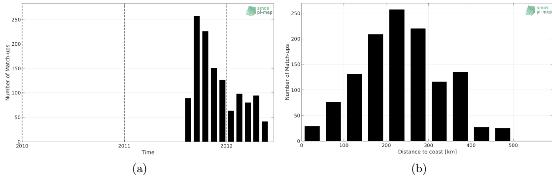
Figure 1: Number of match-ups between Surface drifters and Aquarius-L3-OR-V5-7DAY-RUNNING-RAIN-MASK-1DEG SSS as a function of time (a) and as function of the distance to coast (b) over the Arctic Ocean Pi-MEP region and for the full satellite product period.
