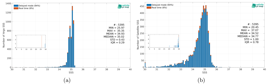
Figure 3: Histograms of SSS from Argo (a) and Aquarius SSS L3 OR v5 - 7-Day running - Rain mask (NASA-GSFC) (b) considering all match-up pairs per bins of 0.1 over the Arctic Ocean Pi-MEP region and for the full satellite product period.
