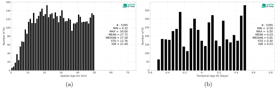
Figure 6: Histograms of the spatial (a) and temporal (b) lags between the location/time of the Argo measurement and the date of the corresponding Aquarius SSS L3 OR v5 - 7-Day running - Rain mask (NASA-GSFC) SSS pixel.
