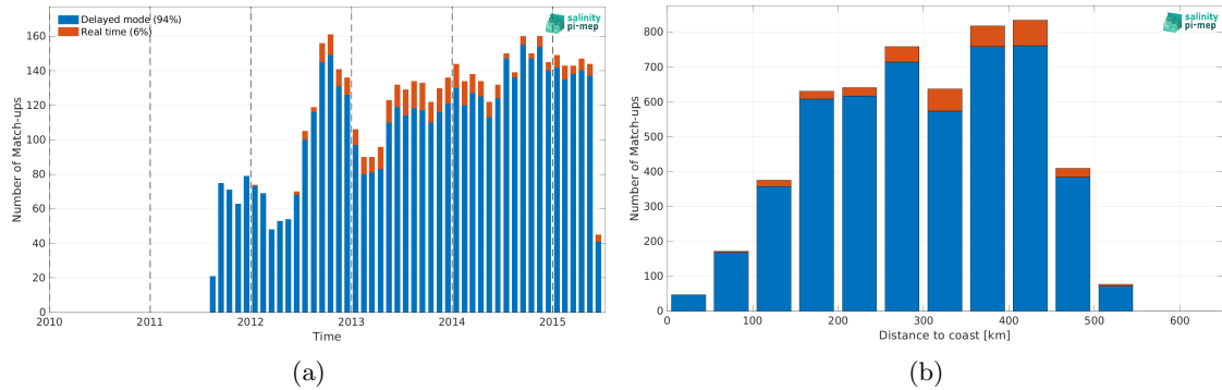
Figure 2: Number of match-ups between Argo and Aquarius SSS L3 OR v5 - 7-Day running - Rain mask (NASA-GSFC) SSS as a function of time (a) and as function of the distance to coast (b) over the Arctic Ocean Pi-MEP region and for the full satellite product period.
