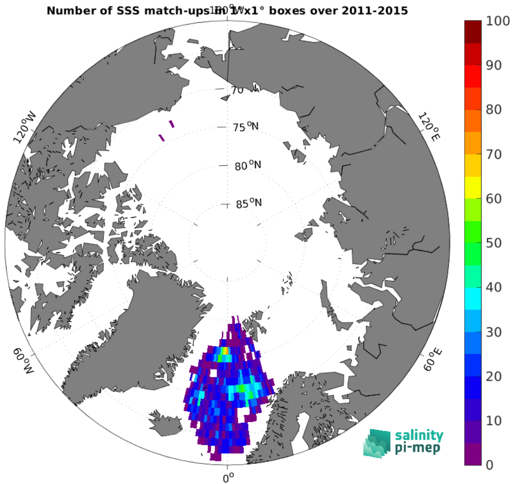
Figure 5: Number of SSS match-ups between Argo SSS and the Aquarius SSS L3 OR v5 - 7-Day running - Rain mask (NASA-GSFC) SSS product for the Arctic Ocean Pi-MEP region over 1^\circ \times 1^\circ boxes and for the full satellite product period.
