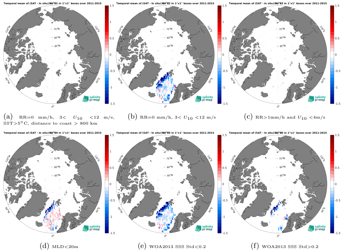
Figure 14: Temporal mean gridded over spatial boxes of size 1^\circ \times 1^\circ of \Delta SSS (Aquarius SSS L3 OR v5 - 7-Day running - Rain mask (NASA-GSFC) - Argo) for 6 different subdatasets corresponding to:RR=0 mm/h, 3 < U_{10} < 12 m/s, SST>5°C, distance to coast > 800 km (a), RR=0 mm/h, 3 < U_{10} < 12 m/s (b), RR>1mm/h and U_{10} < 4 m/s (c),MLD<20m (d),WOA2013 SSS Std<0.2 (e),WOA2013 SSS Std>0.2 (f).
