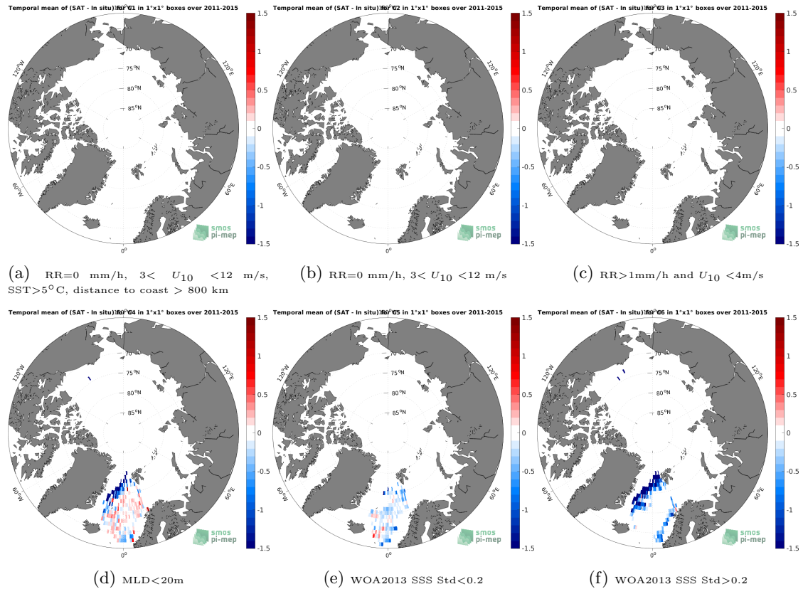
Figure 12: Temporal mean gridded over spatial boxes of size 1^{\circ}\times 1^{\circ} of \Delta\text{SSS} (Aquarius SSS L3 OR v5 - 7-Day running - Rain mask (NASA-GSFC) - Argo) for 6 different subdatasets corresponding to:RR=0 mm/h, 3 < U_{10} < 12 m/s, SST >5^{\circ}\text{C} , distance to coast > 800 km (a), RR=0 mm/h, 3 < U_{10} < 12 m/s (b), RR >1 mm/h and U_{10} < 4 m/s (c),MLD <20 m (d),WOA2013 SSS Std <0.2 (e),WOA2013 SSS Std >0.2 (f).
