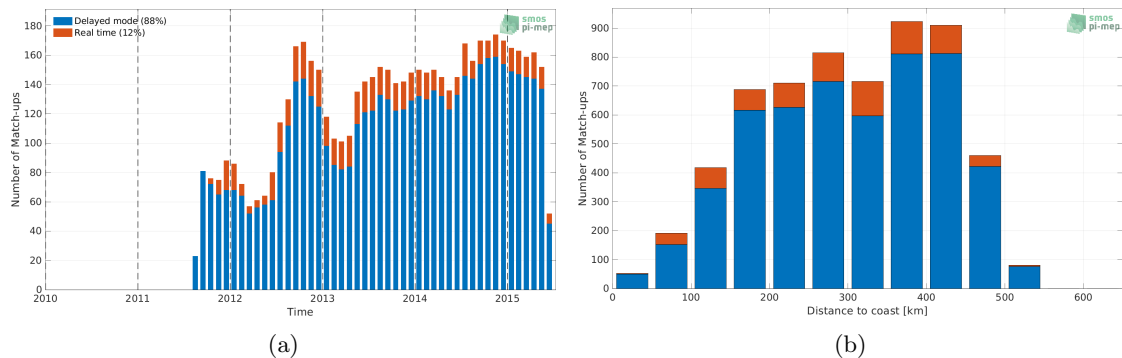
Figure 1: Number of match-ups between Argo and Aquarius SSS L3 OR v5 - 7-Day running - Rain mask (NASA-GSFC) SSS as a function of time (a) and as function of the distance to coast (b) over the Arctic Ocean Pi-MEP region and for the full satellite product period.
