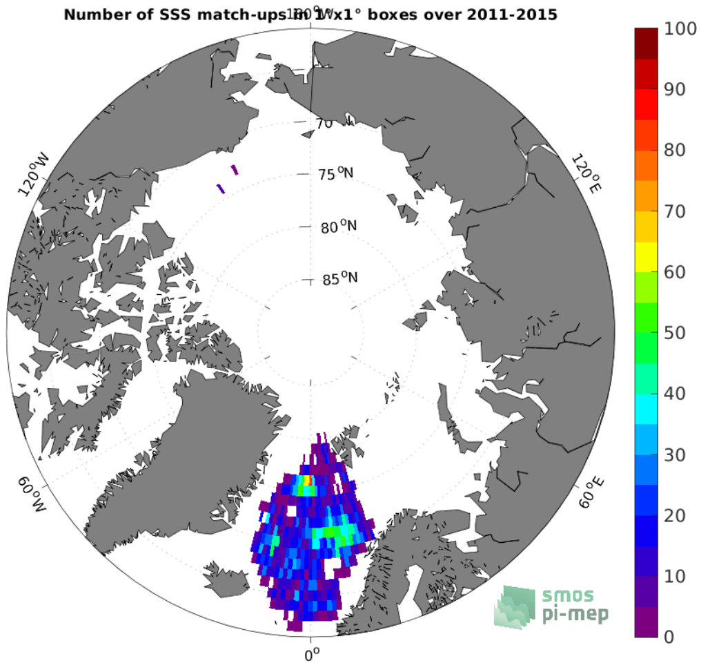
Figure 4: Number of SSS match-ups between Argo SSS and the Aquarius SSS L3 OR v5 - 7-Day running - Rain mask (NASA-GSFC) SSS product for the Arctic Ocean Pi-MEP region over 1^{\circ} \times 1^{\circ} boxes and for the full satellite product period.
