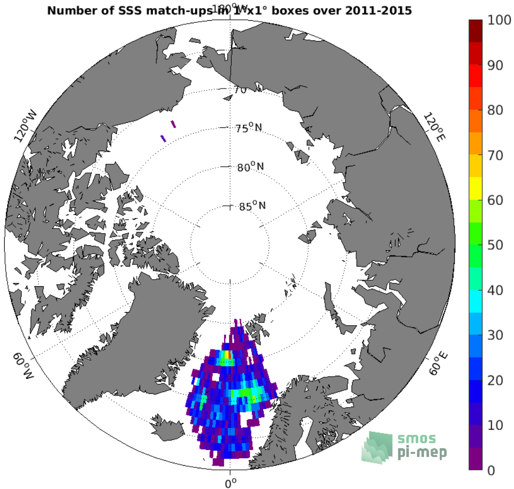
Figure 4: Number of SSS match-ups between Argo SSS and the Aquarius SSS L3 OR v5 - 7-Day running - Rain mask (NASA-GSFC) SSS product for the Arctic Ocean Pi-MEP region over 1^\circ \times 1^\circ boxes and for the full satellite product period.
