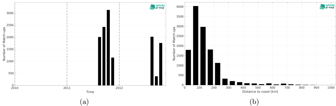
Figure 2: Number of match-ups between TSG (SAMOS) and Aquarius SSS L3 OR v5 - Monthly (NASA-GSFC) SSS as a function of time (a) and as function of the distance to coast (b) over the Arctic Ocean Pi-MEP region and for the full satellite product period.
