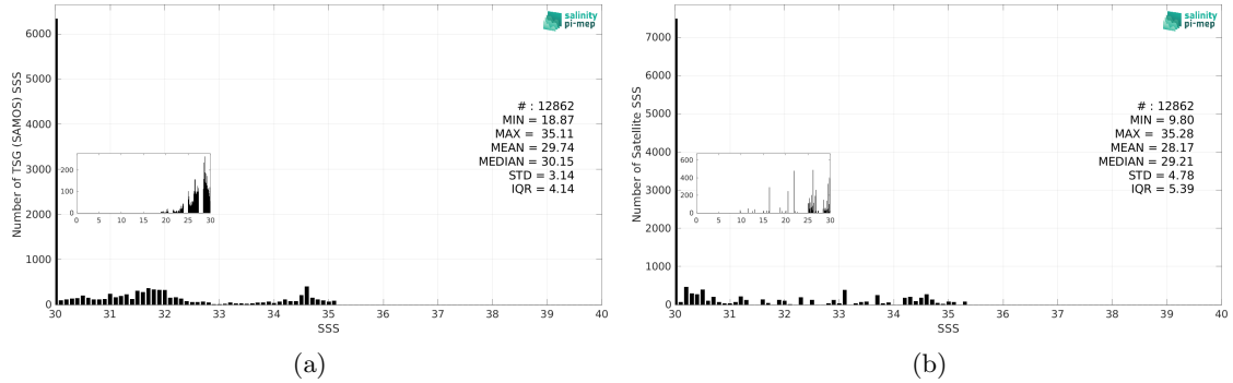
Figure 3: Histograms of SSS from TSG (SAMOS) (a) and Aquarius SSS L3 OR v5 - Monthly (NASA-GSFC) (b) considering all match-up pairs per bins of 0.1 over the Arctic Ocean Pi-MEP region and for the full satellite product period.
