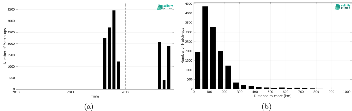
Figure 1: Number of match-ups between TSG (SAMOS) and Aquarius SSS L3 OR v5 - Monthly (NASA-GSFC) SSS as a function of time (a) and as function of the distance to coast (b) over the Arctic Ocean Pi-MEP region and for the full satellite product period.
