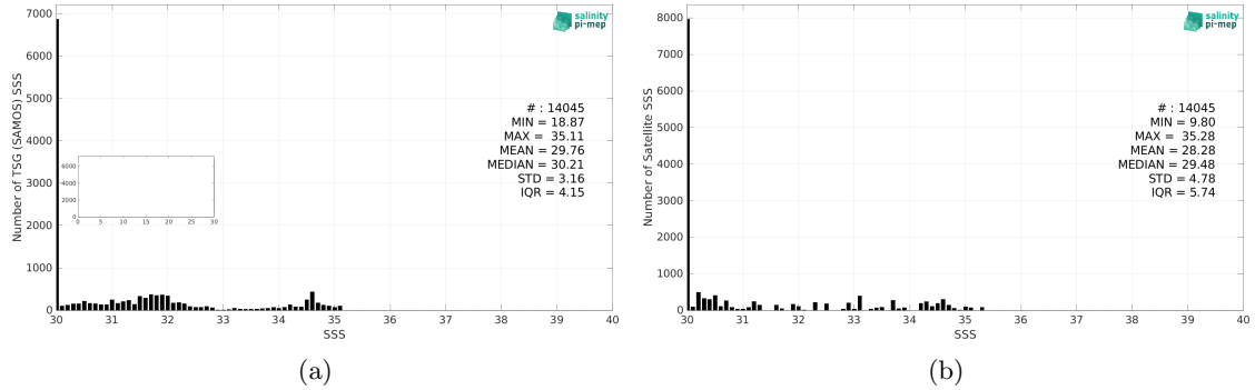
Figure 2: Histograms of SSS from TSG (SAMOS) (a) and Aquarius SSS L3 OR v5 - Monthly (NASA-GSFC) (b) considering all match-up pairs per bins of 0.1 over the Arctic Ocean Pi-MEP region and for the full satellite product period.
