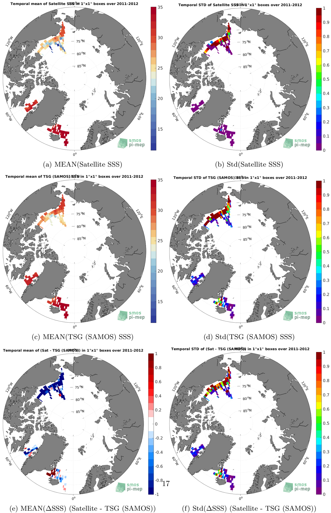
Figure 6: Temporal mean (left) and Std (right) of SSS from Aquarius SSS L3 OR v5 - Monthly (NASA-GSFC) (top), TSG (SAMOS) (middle), and of \Delta SSS (Satellite - TSG (SAMOS)). Only match-up pairs are used to generate these maps.
