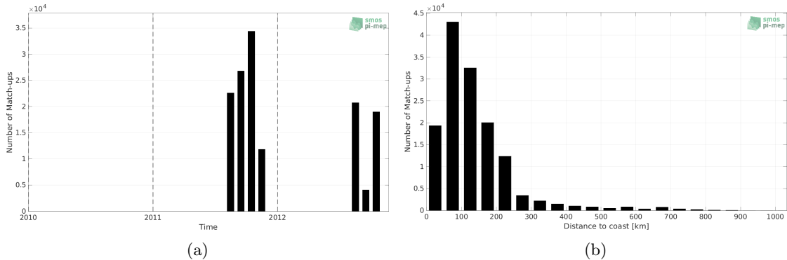
Figure 1: Number of match-ups between TSG (SAMOS) and Aquarius SSS L3 OR v5 - Monthly (NASA-GSFC) SSS as a function of time (a) and as function of the distance to coast (b) over the Arctic Ocean Pi-MEP region and for the full satellite product period.
