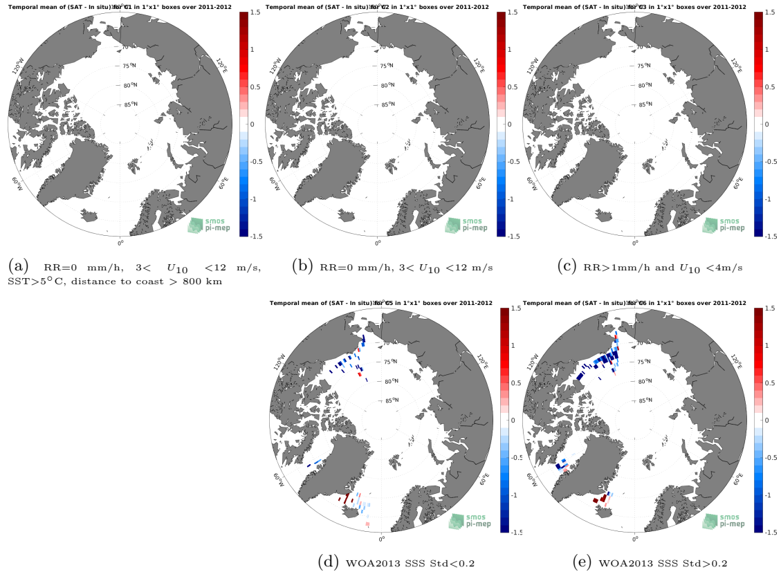
Figure 12: Temporal mean gridded over spatial boxes of size 1^{\circ}\times 1^{\circ} of \Delta\text{SSS} (Aquarius SSS L3 OR v5 - Monthly (NASA-GSFC) - TSG (SAMOS)) for 5 different subdatasets corresponding to: RR=0 mm/h, 3 < U_{10} < 12 m/s, SST > 5^{\circ}\text{C} , distance to coast > 800 km (a), RR=0 mm/h, 3 < U_{10} < 12 m/s (b), RR > 1 mm/h and U_{10} < 4 m/s (c), WOA2013 SSS Std < 0.2 (d), WOA2013 SSS Std > 0.2 (e).
