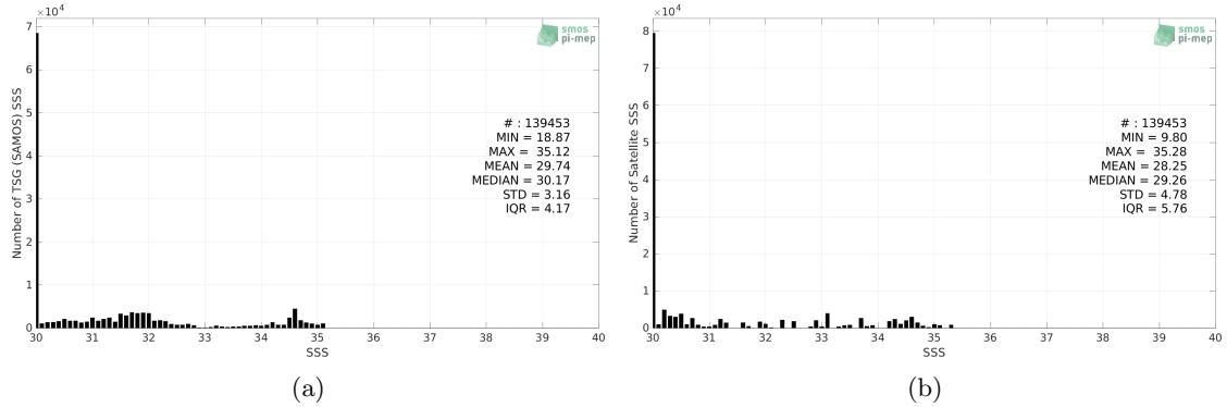
Figure 2: Histograms of SSS from TSG (SAMOS) (a) and Aquarius SSS L3 OR v5 - Monthly (NASA-GSFC) (b) considering all match-up pairs per bins of 0.1 over the Arctic Ocean Pi-MEP region and for the full satellite product period.
