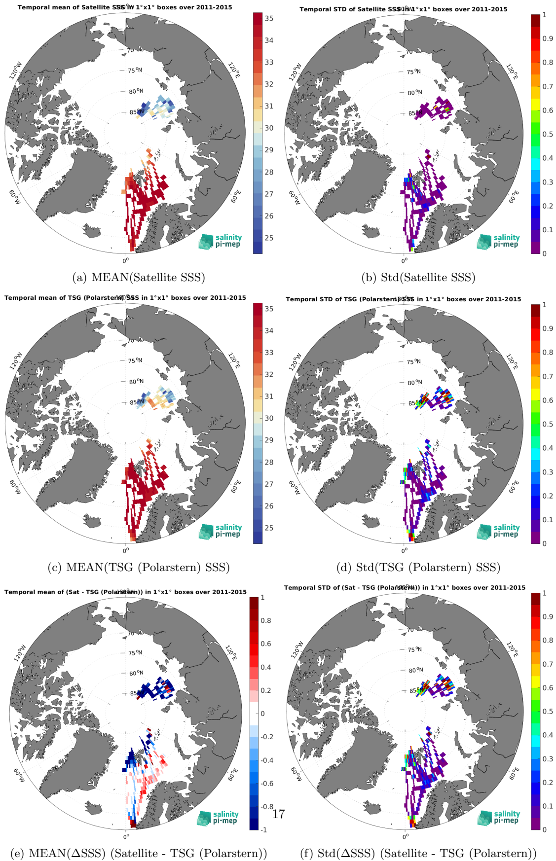
Figure 7: Temporal mean (left) and Std (right) of SSS from Aquarius SSS L3 OR v5 - Monthly (NASA-GSFC) (top), TSG (Polarstern) (middle), and of \Delta SSS (Satellite - TSG (Polarstern)). Only match-up pairs are used to generate these maps.
