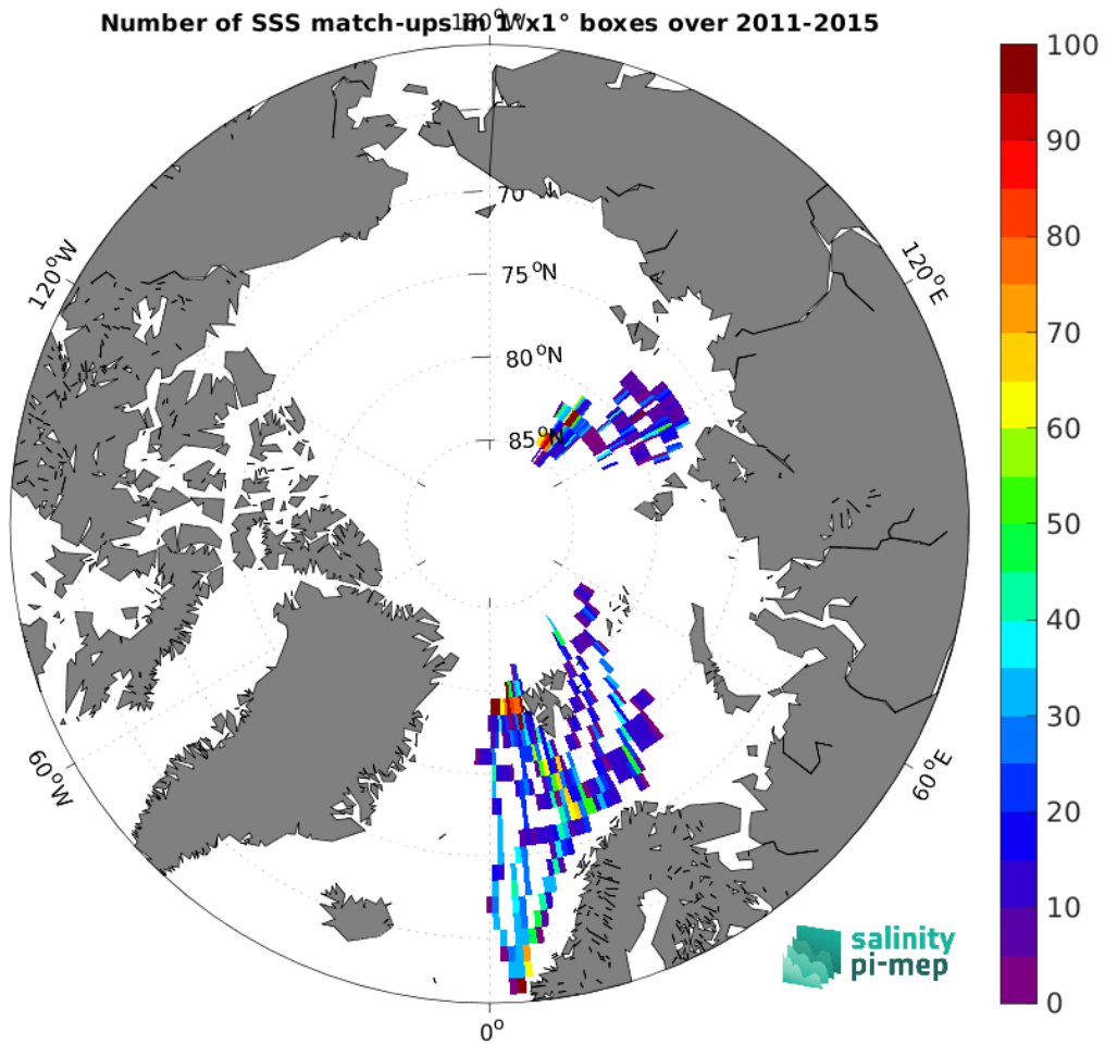
Figure 5: Number of SSS match-ups between TSG (Polarstern) SSS and the Aquarius SSS L3 OR v5 - Monthly (NASA-GSFC) SSS product for the Arctic Ocean Pi-MEP region over 1^\circ \times 1^\circ boxes and for the full satellite product period.
