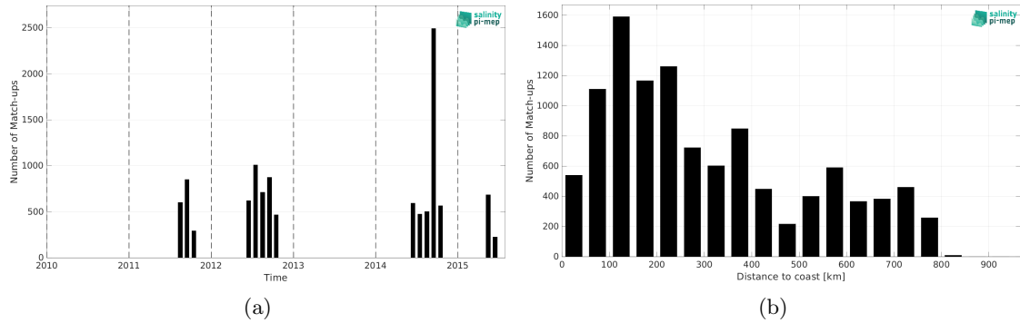
Figure 2: Number of match-ups between TSG (Polarstern) and Aquarius SSS L3 OR v5 - Monthly (NASA-GSFC) SSS as a function of time (a) and as function of the distance to coast (b) over the Arctic Ocean Pi-MEP region and for the full satellite product period.
