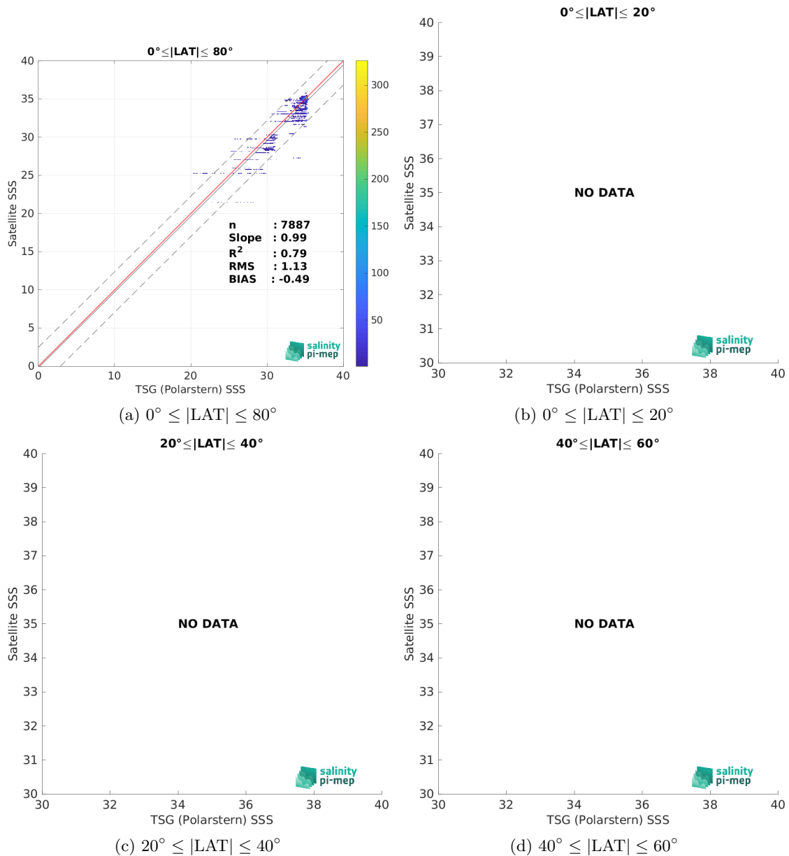
Figure 10: Contour maps of the concentration of Aquarius SSS L3 OR v5 - Monthly (NASA-GSFC) SSS (y-axis) versus TSG (Polarstern) SSS (x-axis) at match-up pairs for different latitude bands. For each plot, the red line shows x=y . The black thin and dashed lines indicate a linear fit through the data cloud and the \pm 95\% confidence levels, respectively. The number match-up pairs n , the slope and R^2 coefficient of the linear fit, the root mean square (RMS) and the mean bias between satellite and in situ data are indicated for each latitude band in each plot.
