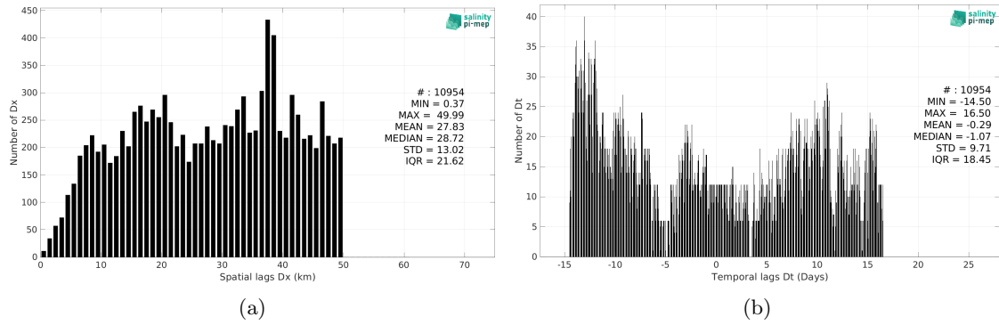
Figure 6: Histograms of the spatial (a) and temporal (b) lags between the location/time of the TSG (Polarstern) measurement and the date of the corresponding Aquarius SSS L3 OR v5 - Monthly (NASA-GSFC) SSS pixel.
