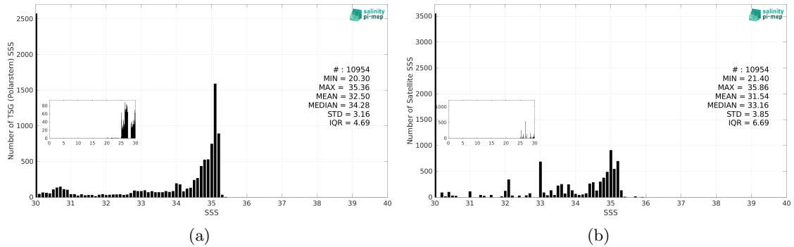
Figure 3: Histograms of SSS from TSG (Polarstern) (a) and Aquarius SSS L3 OR v5 - Monthly (NASA-GSFC) (b) considering all match-up pairs per bins of 0.1 over the Arctic Ocean Pi-MEP region and for the full satellite product period.
