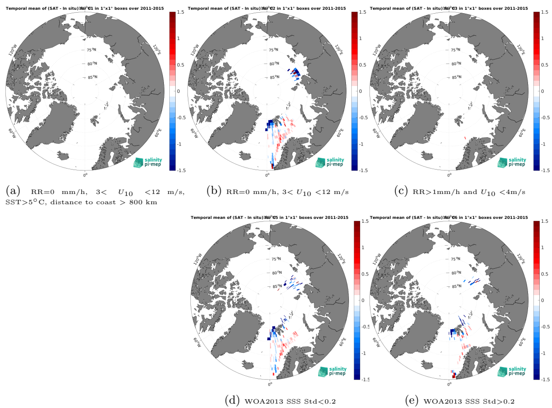
Figure 14: Temporal mean gridded over spatial boxes of size 1^\circ \times 1^\circ of \Delta\text{SSS} (Aquarius SSS L3 OR v5 - Monthly (NASA-GSFC) - TSG (Polarstern)) for 5 different subdatasets corresponding to: RR=0 mm/h, 3 < U_{10} < 12 m/s, SST > 5°C, distance to coast > 800 km (a), RR=0 mm/h, 3 < U_{10} < 12 m/s (b), RR > 1mm/h and U_{10} < 4 m/s (c), WOA2013 SSS Std < 0.2 (d), WOA2013 SSS Std > 0.2 (e).
