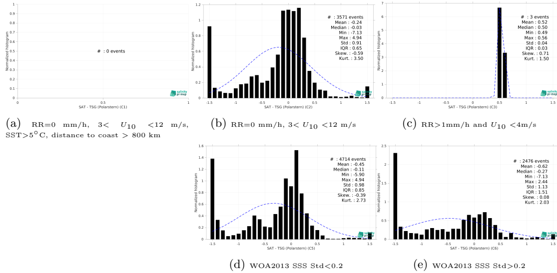
Figure 15: Normalized histogram of \Delta SSS (Aquarius SSS L3 OR v5 - Monthly (NASA-GSFC) - TSG (Polarstern)) for 5 different subdatasets corresponding to: RR=0 mm/h, 3 < U_{10} < 12 m/s, SST > 5°C, distance to coast > 800 km (a), RR=0 mm/h, 3 < U_{10} < 12 m/s (b), RR > 1mm/h and U_{10} < 4 m/s (c), WOA2013 SSS Std < 0.2 (d), WOA2013 SSS Std > 0.2 (e).
