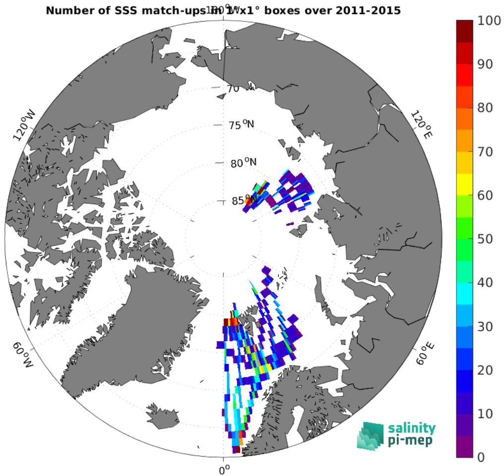
Figure 4: Number of SSS match-ups between TSG (Polarstern) SSS and the Aquarius SSS L3 OR v5 - Monthly (NASA-GSFC) SSS product for the Arctic Ocean Pi-MEP region over 1^\circ \times 1^\circ boxes and for the full satellite product period.
