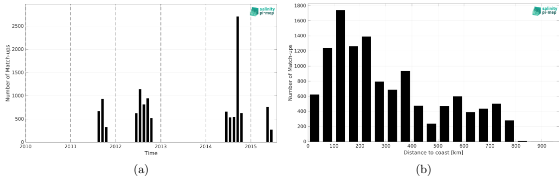
Figure 1: Number of match-ups between TSG (Polarstern) and Aquarius SSS L3 OR v5 - Monthly (NASA-GSFC) SSS as a function of time (a) and as function of the distance to coast (b) over the Arctic Ocean Pi-MEP region and for the full satellite product period.
