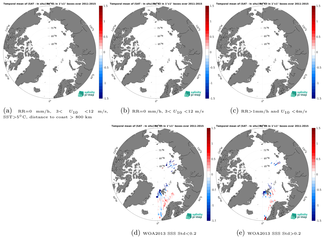
Figure 12: Temporal mean gridded over spatial boxes of size 1^{\circ}\times 1^{\circ} of \Delta\text{SSS} (Aquarius SSS L3 OR v5 - Monthly (NASA-GSFC) - TSG (Polarstern)) for 5 different subdatasets corresponding to: RR=0 mm/h, 3 < U_{10} < 12 m/s, SST > 5^{\circ}\text{C} , distance to coast > 800 km (a), RR=0 mm/h, 3 < U_{10} < 12 m/s (b), RR > 1 mm/h and U_{10} < 4 m/s (c), WOA2013 SSS Std < 0.2 (d), WOA2013 SSS Std > 0.2 (e).
