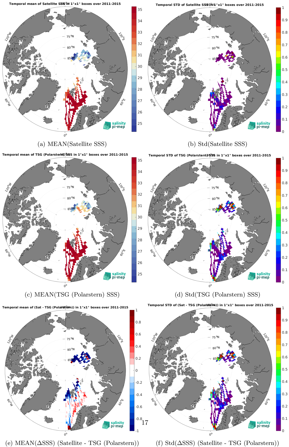
Figure 6: Temporal mean (left) and Std (right) of SSS from Aquarius SSS L3 OR v5 - Monthly (NASA-GSFC) (top), TSG (Polarstern) (middle), and of \Delta SSS (Satellite - TSG (Polarstern)). Only match-up pairs are used to generate these maps.
