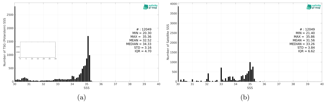
Figure 2: Histograms of SSS from TSG (Polarstern) (a) and Aquarius SSS L3 OR v5 - Monthly (NASA-GSFC) (b) considering all match-up pairs per bins of 0.1 over the Arctic Ocean Pi-MEP region and for the full satellite product period.
