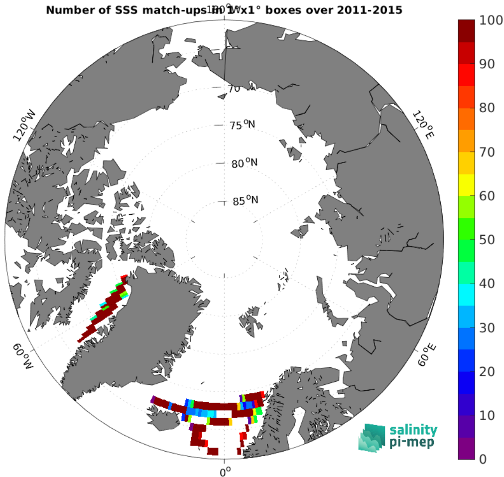
Figure 5: Number of SSS match-ups between TSG (LEGOS-DM) SSS and the Aquarius SSS L3 OR v5 - Monthly (NASA-GSFC) SSS product for the Arctic Ocean Pi-MEP region over 1^\circ \times 1^\circ boxes and for the full satellite product period.
