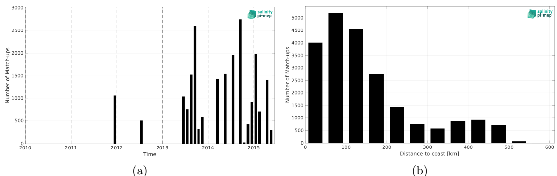
Figure 2: Number of match-ups between TSG (LEGOS-DM) and Aquarius SSS L3 OR v5 - Monthly (NASA-GSFC) SSS as a function of time (a) and as function of the distance to coast (b) over the Arctic Ocean Pi-MEP region and for the full satellite product period.
