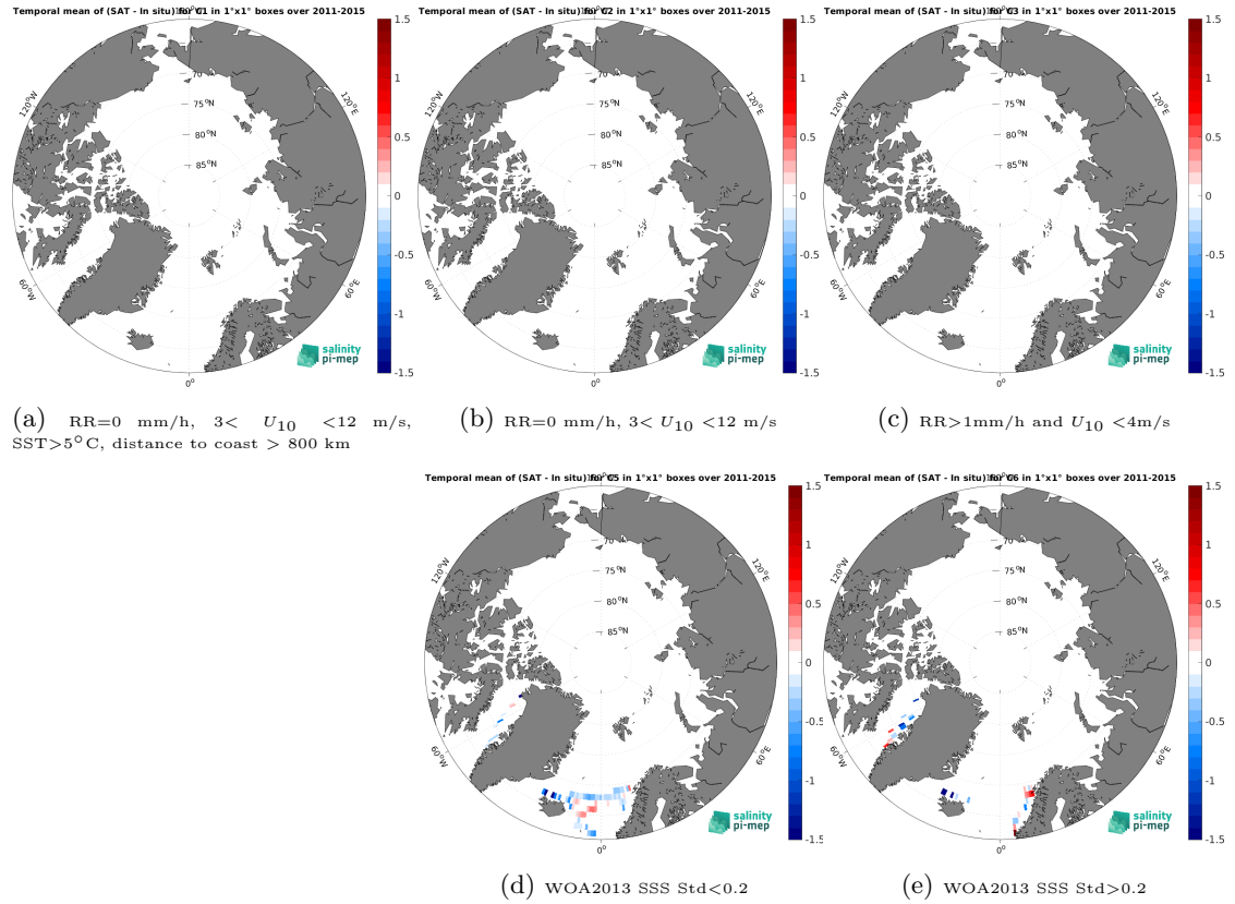
Figure 12: Temporal mean gridded over spatial boxes of size 1^{\circ}\times 1^{\circ} of \Delta\text{SSS} (Aquarius SSS L3 OR v5 - Monthly (NASA-GSFC) - TSG (LEGOS-DM)) for 5 different subdatasets corresponding to:RR=0 mm/h, 3 < U_{10} < 12 m/s, SST >5^{\circ}\text{C} , distance to coast > 800 km (a), RR=0 mm/h, 3 < U_{10} < 12 m/s (b), RR >1 mm/h and U_{10} < 4 m/s (c), WOA2013 SSS Std <0.2 (d), WOA2013 SSS Std >0.2 (e).
