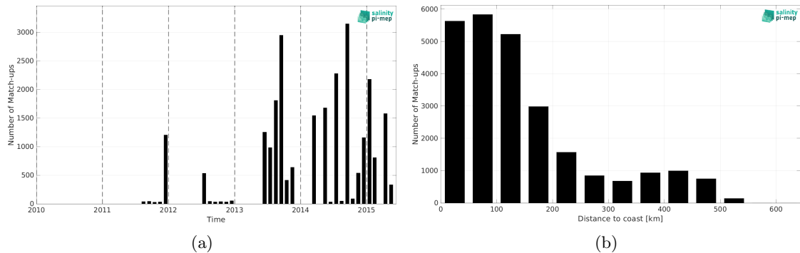
Figure 1: Number of match-ups between TSG (LEGOS-DM) and Aquarius SSS L3 OR v5 - Monthly (NASA-GSFC) SSS as a function of time (a) and as function of the distance to coast (b) over the Arctic Ocean Pi-MEP region and for the full satellite product period.
