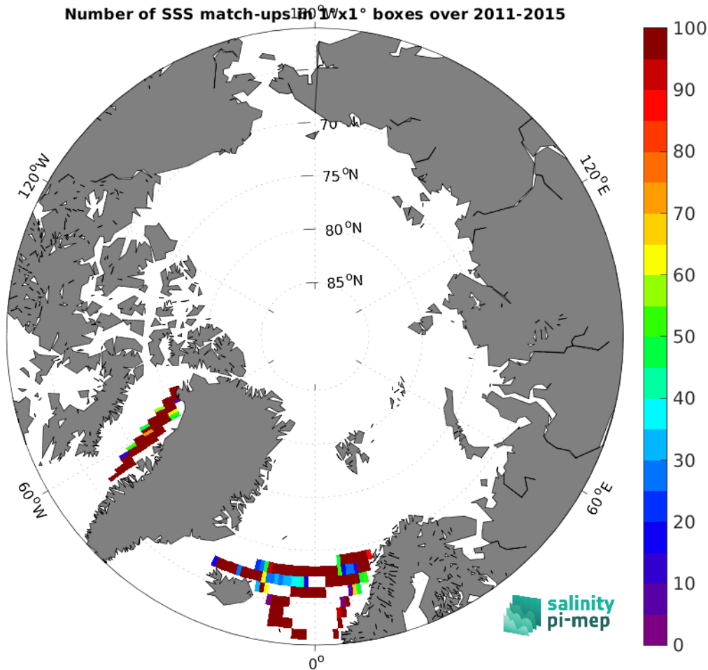
Figure 4: Number of SSS match-ups between TSG (LEGOS-DM) SSS and the Aquarius SSS L3 OR v5 - Monthly (NASA-GSFC) SSS product for the Arctic Ocean Pi-MEP region over 1^\circ \times 1^\circ boxes and for the full satellite product period.
