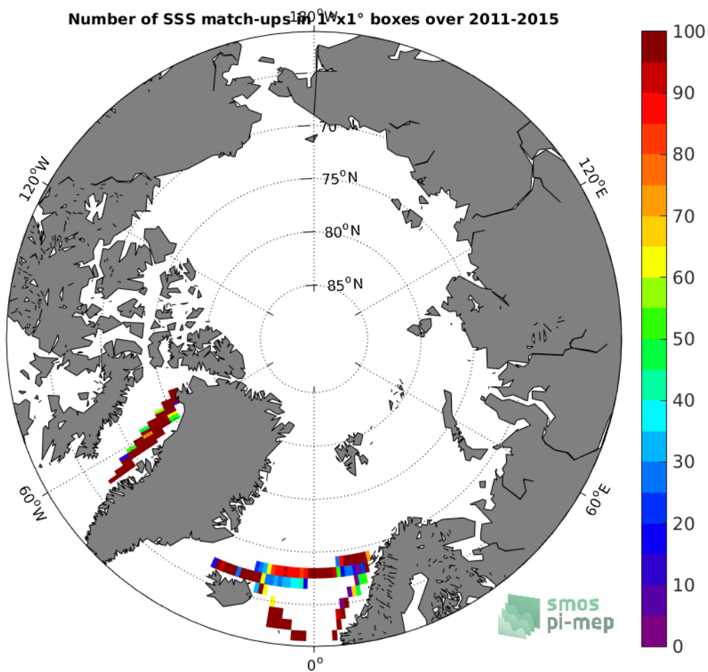
Figure 4: Number of SSS match-ups between TSG-LEGOS-DM SSS and the Aquarius-L3-OR-V5-MONTHLY-1DEG SSS product for the Arctic Ocean Pi-MEP region over 1^\circ \times 1^\circ boxes and for the full satellite product period.
