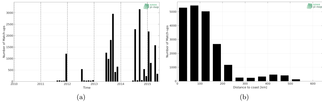
Figure 1: Number of match-ups between TSG-LEGOS-DM and Aquarius-L3-OR-V5-MONTHLY-1DEG SSS as a function of time (a) and as function of the distance to coast (b) over the Arctic Ocean Pi-MEP region and for the full satellite product period.
