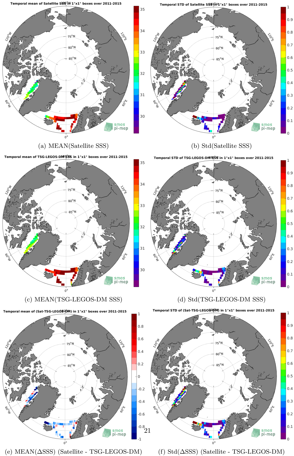
Figure 6: Temporal mean (left) and Std (right) of SSS from Aquarius-L3-OR-V5-MONTHLY-1DEG (top), TSG-LEGOS-DM (middle), and of \Delta SSS (Satellite - TSG-LEGOS-DM). Only match-up pairs are used to generate these maps.
