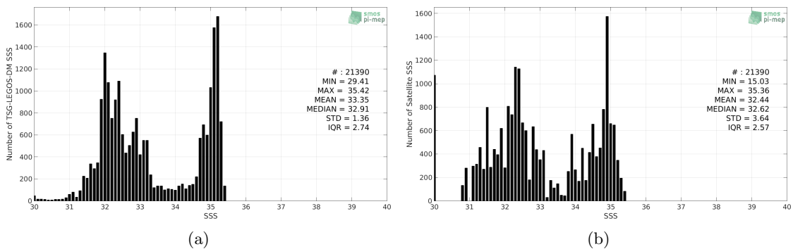
Figure 2: Histograms of SSS from TSG-LEGOS-DM (a) and Aquarius-L3-OR-V5-MONTHLY-1DEG (b) considering all match-up pairs per bins of 0.1 over the Arctic Ocean Pi-MEP region and for the full satellite product period.
