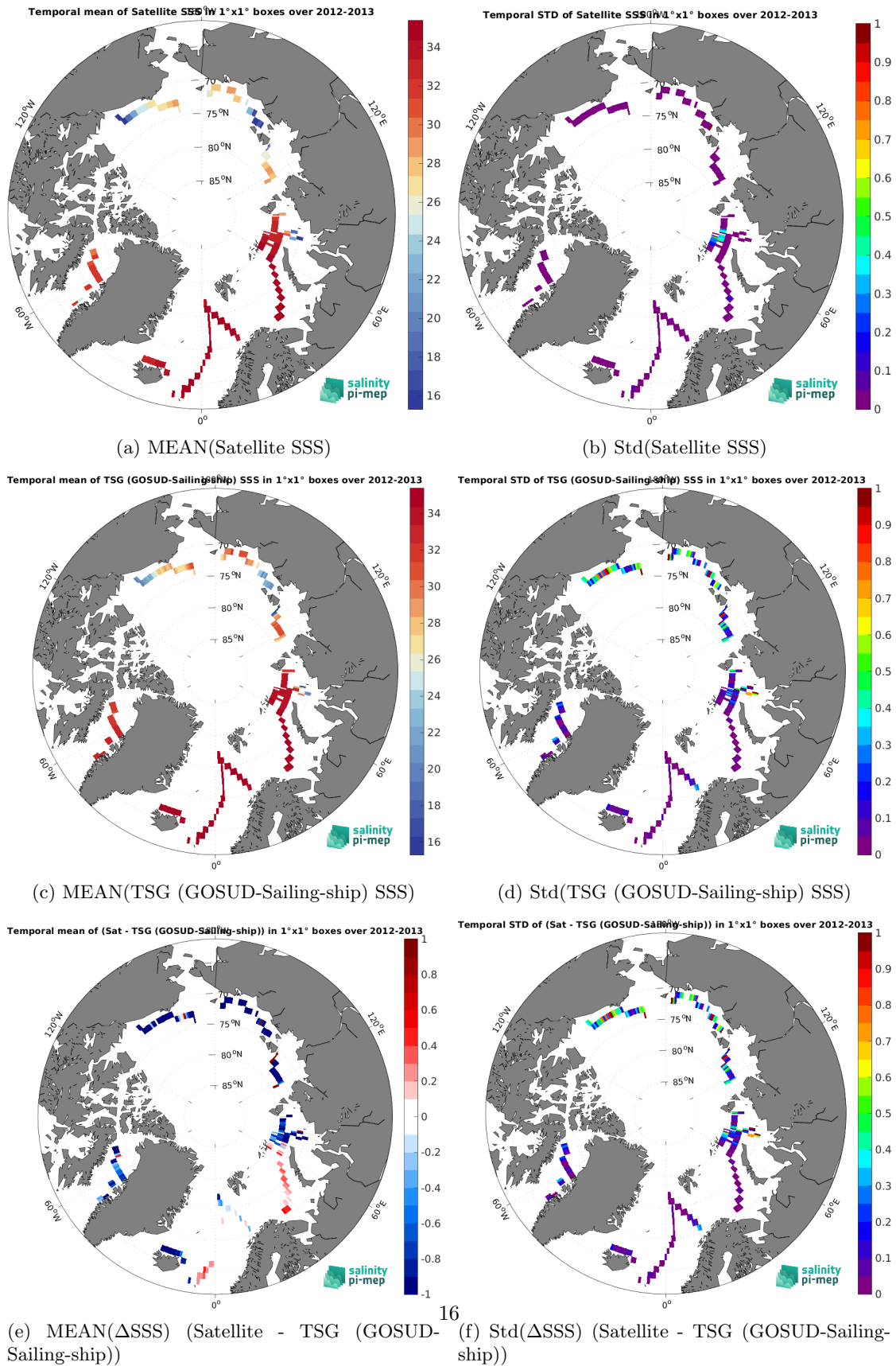
Figure 7: Temporal mean (left) and Std (right) of SSS from Aquarius SSS L3 OR v5 - Monthly (NASA-GSFC) (top), TSG (GOSUD-Sailing-ship) (middle), and of \Delta SSS (Satellite - TSG (GOSUD-Sailing-ship)). Only match-up pairs are used to generate these maps.
