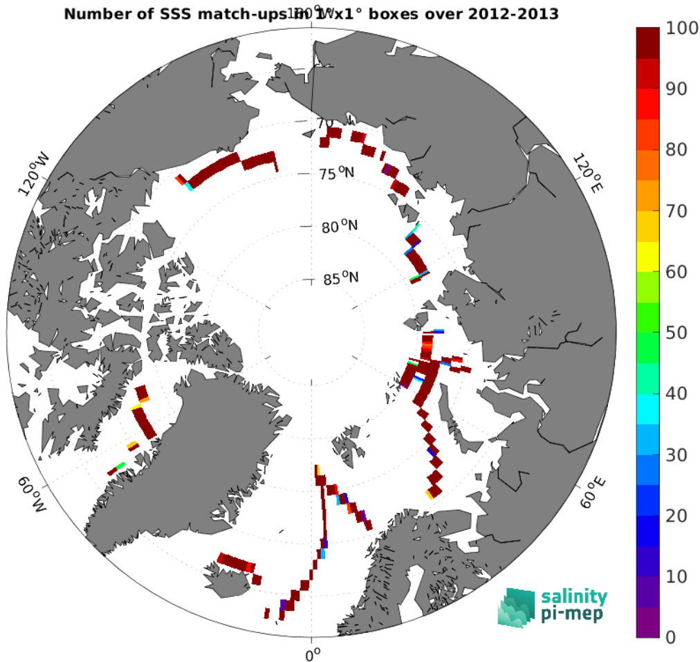
Figure 5: Number of SSS match-ups between TSG (GOSUD-Sailing-ship) SSS and the Aquarius SSS L3 OR v5 - Monthly (NASA-GSFC) SSS product for the Arctic Ocean Pi-MEP region over 1^\circ \times 1^\circ boxes and for the full satellite product period.
