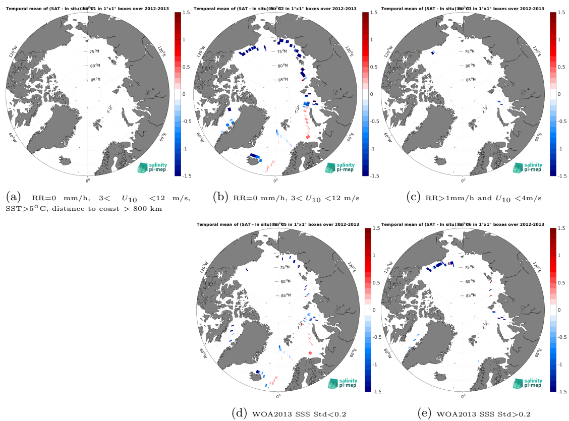
Figure 14: Temporal mean gridded over spatial boxes of size 1^\circ \times 1^\circ of \Delta SSS (Aquarius SSS L3 OR v5 - Monthly (NASA-GSFC) - TSG (GOSUD-Sailing-ship)) for 5 different subdatasets corresponding to: RR=0 mm/h, 3 < U_{10} < 12 m/s, SST >5^\circ\text{C} , distance to coast > 800 km (a), RR=0 mm/h, 3 < U_{10} < 12 m/s (b), RR >1 mm/h and U_{10} < 4 m/s (c), WOA2013 SSS Std <0.2 (d), WOA2013 SSS Std >0.2 (e).
