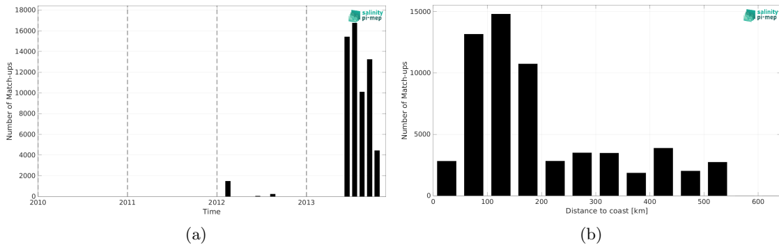
Figure 2: Number of match-ups between TSG (GOSUD-Sailing-ship) and Aquarius SSS L3 OR v5 - Monthly (NASA-GSFC) SSS as a function of time (a) and as function of the distance to coast (b) over the Arctic Ocean Pi-MEP region and for the full satellite product period.
