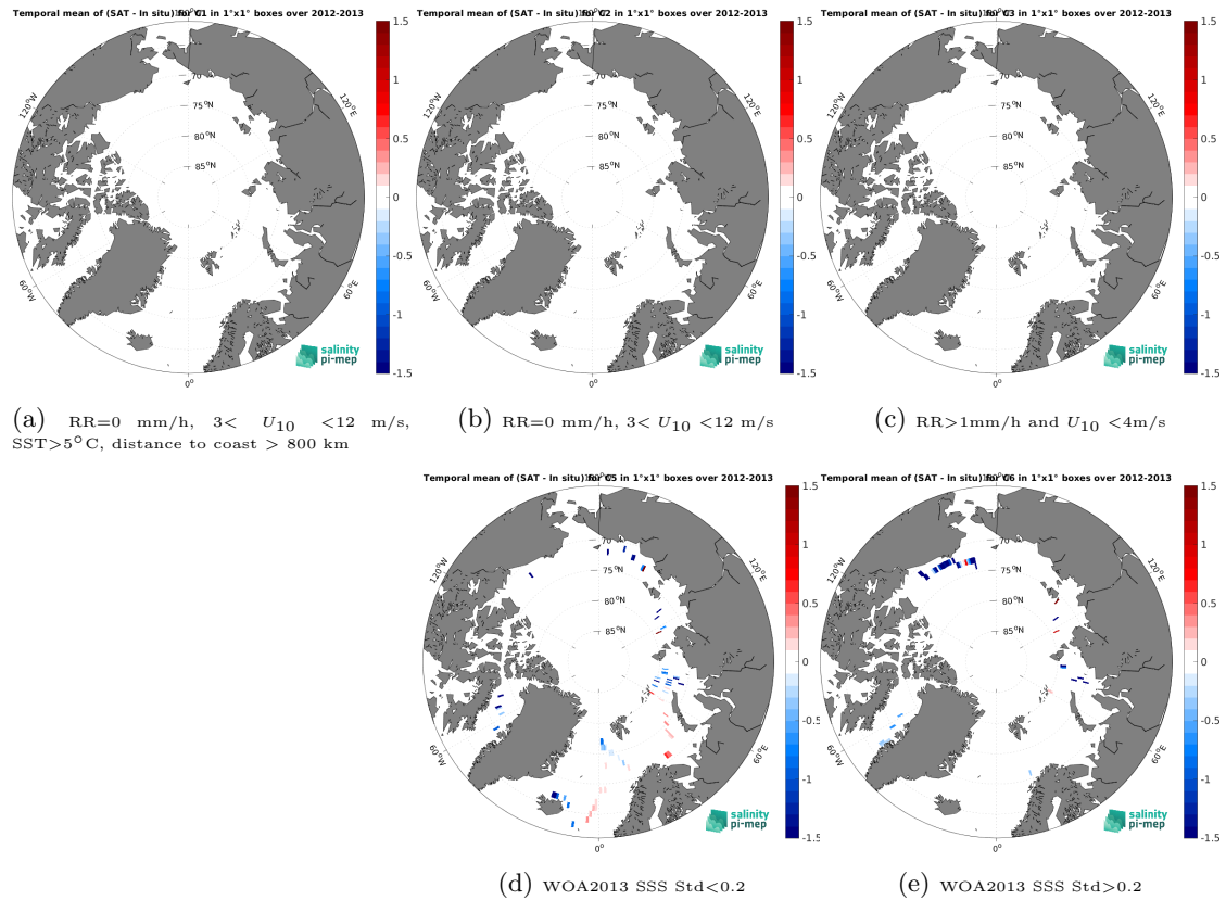
Figure 12: Temporal mean gridded over spatial boxes of size 1^\circ \times 1^\circ of \Delta\text{SSS} (Aquarius SSS L3 OR v5 - Monthly (NASA-GSFC) - TSG (GOSUD-Sailing-ship)) for 5 different subdatasets corresponding to: RR=0 mm/h, 3 < U_{10} < 12 m/s, SST > 5^\circ\text{C} , distance to coast > 800 km (a), RR=0 mm/h, 3 < U_{10} < 12 m/s (b), RR > 1\text{mm/h} and U_{10} < 4\text{m/s} (c), WOA2013 SSS Std < 0.2 (d), WOA2013 SSS Std > 0.2 (e).
