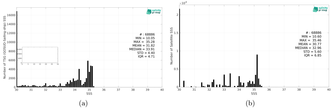
Figure 2: Histograms of SSS from TSG (GOSUD-Sailing-ship) (a) and Aquarius SSS L3 OR v5 - Monthly (NASA-GSFC) (b) considering all match-up pairs per bins of 0.1 over the Arctic Ocean Pi-MEP region and for the full satellite product period.
