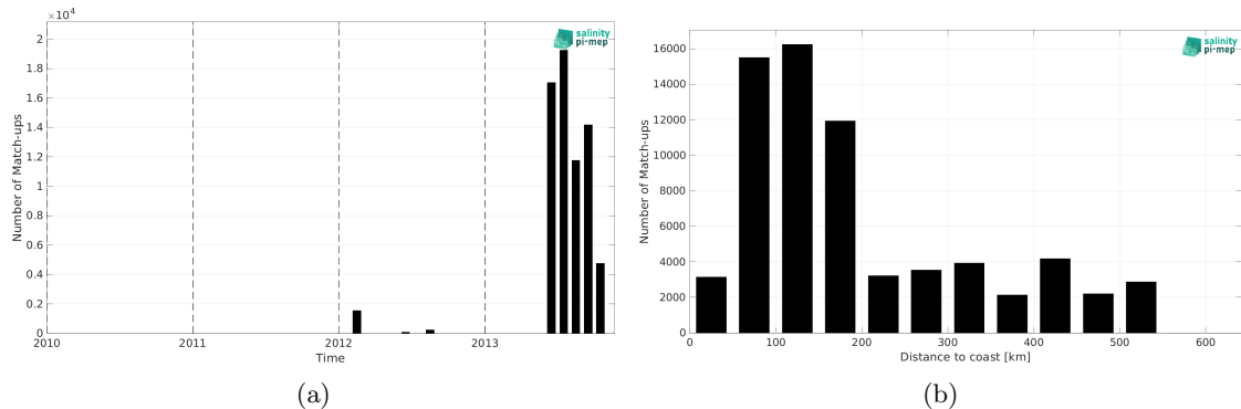
Figure 1: Number of match-ups between TSG (GOSUD-Sailing-ship) and Aquarius SSS L3 OR v5 - Monthly (NASA-GSFC) SSS as a function of time (a) and as function of the distance to coast (b) over the Arctic Ocean Pi-MEP region and for the full satellite product period.
