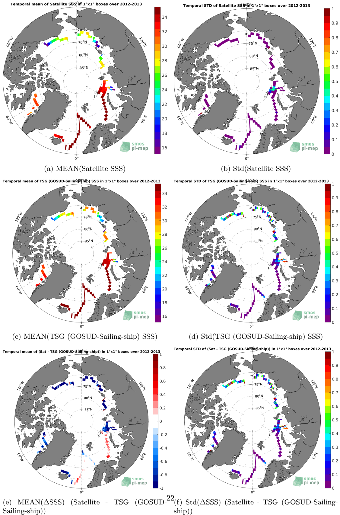
Figure 6: Temporal mean (left) and Std (right) of SSS from Aquarius SSS L3 OR v5 - Monthly (NASA-GSFC) (top), TSG (GOSUD-Sailing-ship) (middle), and of \Delta SSS (Satellite - TSG (GOSUD-Sailing-ship)). Only match-up pairs are used to generate these maps.
