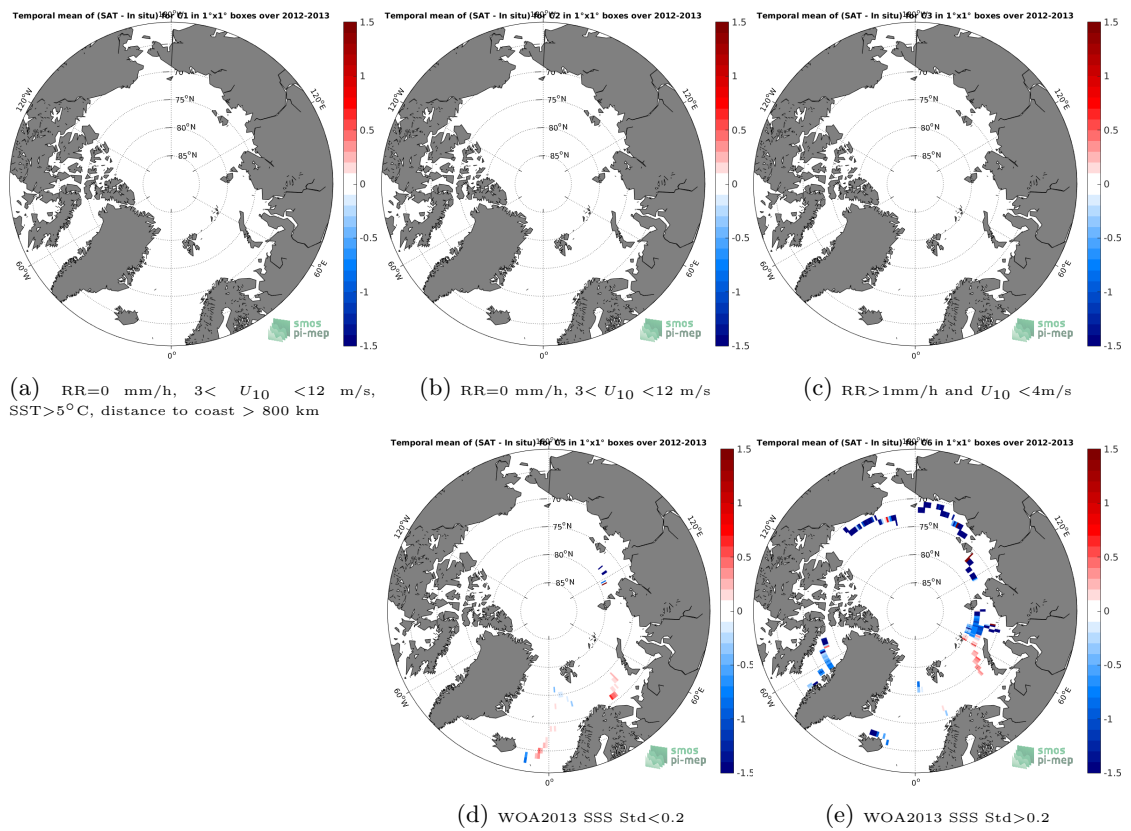
Figure 12: Temporal mean gridded over spatial boxes of size 1°x1° of \Delta SSS (Aquarius-L3-OR-V5-MONTHLY-1DEG - TSG-GOSUD-Sailing-ship) for 5 different subdatasets corresponding to:RR=0 mm/h, 3 < U_{10} < 12 m/s, SST>5°C, distance to coast > 800 km (a), RR=0 mm/h, 3 < U_{10} < 12 m/s (b), RR>1mm/h and U_{10} < 4 m/s (c), WOA2013 SSS Std<0.2 (d), WOA2013 SSS Std>0.2 (e).
