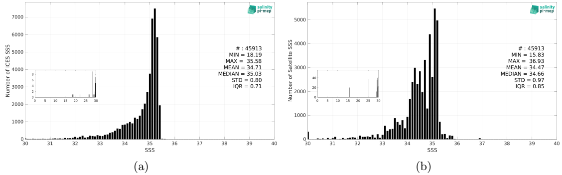
Figure 3: Histograms of SSS from ICES (a) and Aquarius SSS L3 OR v5 - Monthly (NASA-GSFC) (b) considering all match-up pairs per bins of 0.1 over the Arctic Ocean Pi-MEP region and for the full satellite product period.
