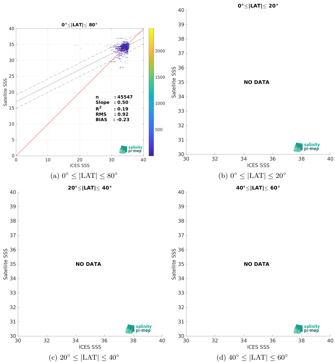
Figure 10: Contour maps of the concentration of Aquarius SSS L3 OR v5 - Monthly (NASA-GSFC) SSS (y-axis) versus ICES SSS (x-axis) at match-up pairs for different latitude bands. For each plot, the red line shows x=y . The black thin and dashed lines indicate a linear fit through the data cloud and the \pm 95\% confidence levels, respectively. The number match-up pairs n , the slope and R^2 coefficient of the linear fit, the root mean square (RMS) and the mean bias between satellite and in situ data are indicated for each latitude band in each plots.
