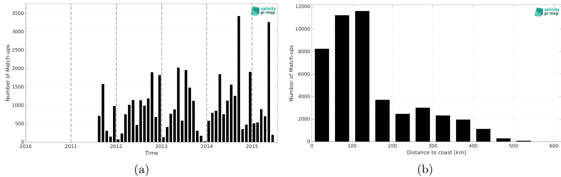
Figure 2: Number of match-ups between ICES and Aquarius SSS L3 OR v5 - Monthly (NASA-GSFC) SSS as a function of time (a) and as function of the distance to coast (b) over the Arctic Ocean Pi-MEP region and for the full satellite product period.
