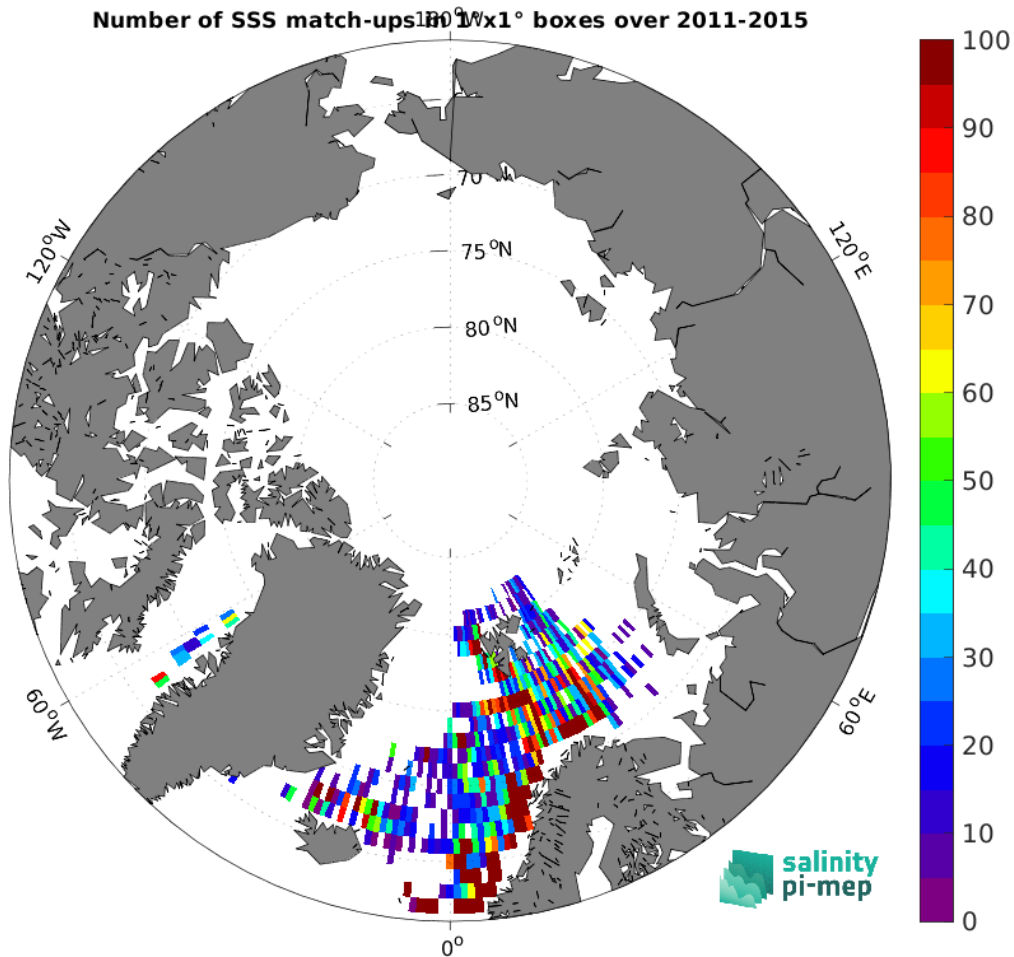
Figure 5: Number of SSS match-ups between ICES SSS and the Aquarius SSS L3 OR v5 - Monthly (NASA-GSFC) SSS product for the Arctic Ocean Pi-MEP region over 1^\circ \times 1^\circ boxes and for the full satellite product period.
