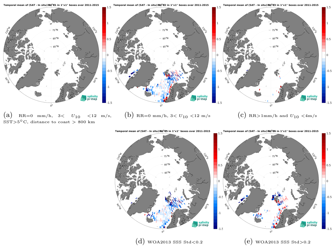
Figure 14: Temporal mean gridded over spatial boxes of size 1^\circ \times 1^\circ of \Delta SSS (Aquarius SSS L3 OR v5 - Monthly (NASA-GSFC) - ICES) for 5 different subdatasets corresponding to:RR=0 mm/h, 3 < U_{10} < 12 m/s, SST > 5^\circ\text{C} , distance to coast > 800 km (a), RR=0 mm/h, 3 < U_{10} < 12 m/s (b), RR > 1 mm/h and U_{10} < 4 m/s (c), WOA2013 SSS Std < 0.2 (d), WOA2013 SSS Std > 0.2 (e).
