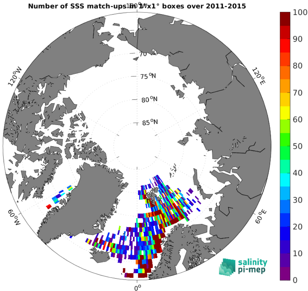
Figure 4: Number of SSS match-ups between ICES SSS and the Aquarius SSS L3 OR v5 - Monthly (NASA-GSFC) SSS product for the Arctic Ocean Pi-MEP region over 1^\circ \times 1^\circ boxes and for the full satellite product period.
