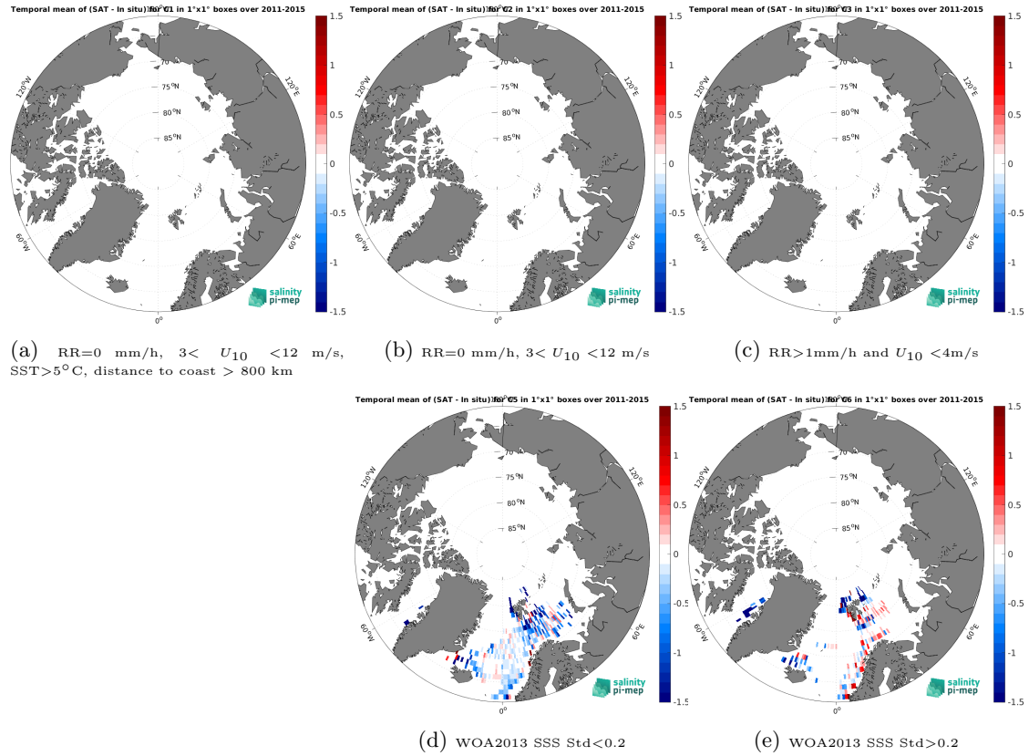
Figure 12: Temporal mean gridded over spatial boxes of size 1^{\circ}\times 1^{\circ} of \Delta\text{SSS} (Aquarius SSS L3 OR v5 - Monthly (NASA-GSFC) - ICES) for 5 different subdatasets corresponding to:RR=0 mm/h, 3 < U_{10} < 12 m/s, SST > 5^{\circ}\text{C} , distance to coast > 800 km (a), RR=0 mm/h, 3 < U_{10} < 12 m/s (b), RR > 1 mm/h and U_{10} < 4 m/s (c), WOA2013 SSS Std < 0.2 (d), WOA2013 SSS Std > 0.2 (e).
