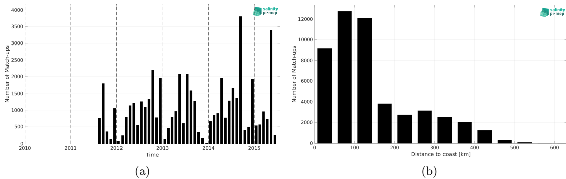
Figure 1: Number of match-ups between ICES and Aquarius SSS L3 OR v5 - Monthly (NASA-GSFC) SSS as a function of time (a) and as function of the distance to coast (b) over the Arctic Ocean Pi-MEP region and for the full satellite product period.
