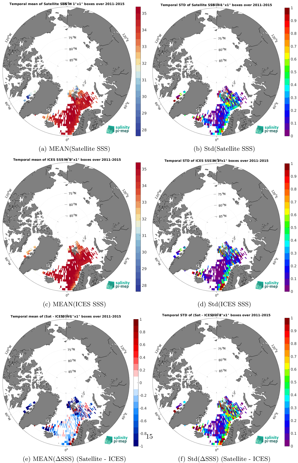
Figure 6: Temporal mean (left) and Std (right) of SSS from Aquarius SSS L3 OR v5 - Monthly (NASA-GSFC) (top), ICES (middle), and of \Delta SSS (Satellite - ICES). Only match-up pairs are used to generate these maps.
