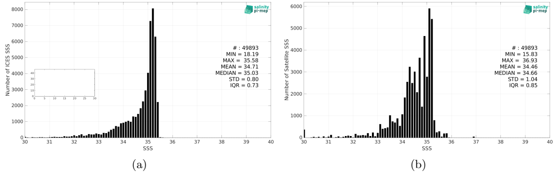
Figure 2: Histograms of SSS from ICES (a) and Aquarius SSS L3 OR v5 - Monthly (NASA-GSFC) (b) considering all match-up pairs per bins of 0.1 over the Arctic Ocean Pi-MEP region and for the full satellite product period.
