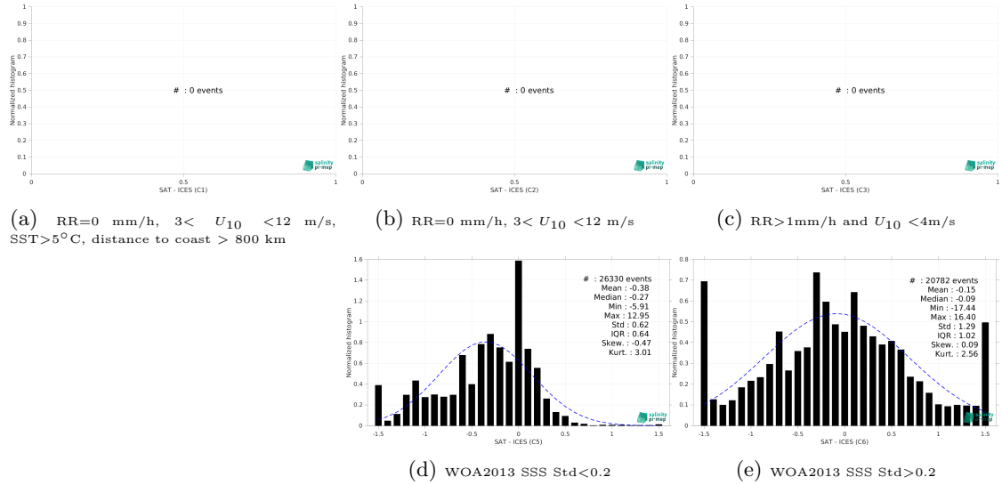
Figure 13: Normalized histogram of \Delta SSS (Aquarius SSS L3 OR v5 - Monthly (NASA-GSFC) - ICES) for 5 different subdatasets corresponding to: RR=0 mm/h, 3 < U_{10} < 12 m/s, SST > 5°C, distance to coast > 800 km (a), RR=0 mm/h, 3 < U_{10} < 12 m/s (b), RR > 1mm/h and U_{10} < 4 m/s (c), WOA2013 SSS Std < 0.2 (d), WOA2013 SSS Std > 0.2 (e).
