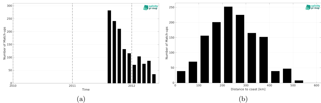
Figure 2: Number of match-ups between Surface drifters and Aquarius SSS L3 OR v5 - Monthly (NASA-GSFC) SSS as a function of time (a) and as function of the distance to coast (b) over the Arctic Ocean Pi-MEP region and for the full satellite product period.
