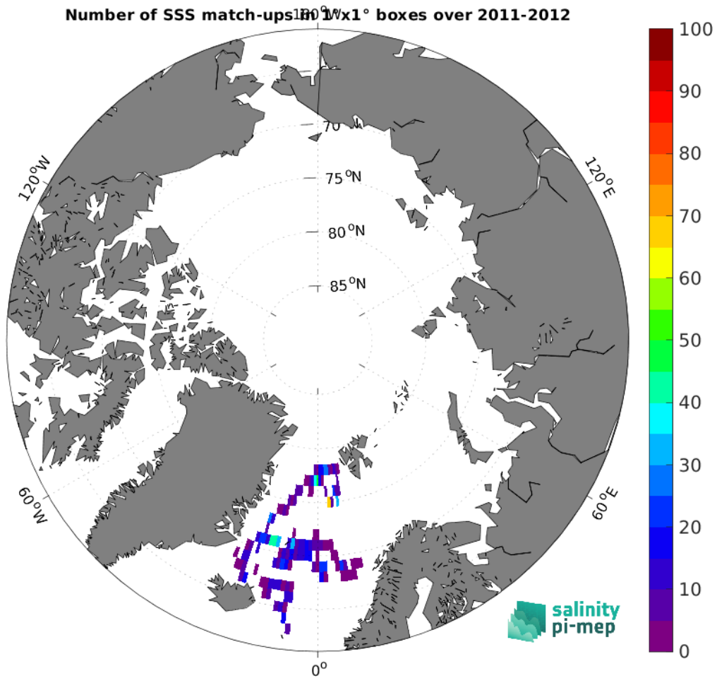
Figure 4: Number of SSS match-ups between Surface drifters SSS and the Aquarius SSS L3 OR v5 - Monthly (NASA-GSFC) SSS product for the Arctic Ocean Pi-MEP region over 1^{\circ} \times 1^{\circ} boxes and for the full satellite product period.
