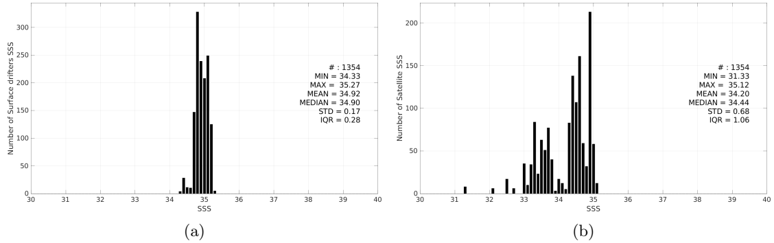
Figure 3: Histograms of SSS from Surface drifters (a) and Aquarius SSS L3 OR v5 - Monthly (NASA-GSFC) (b) considering all match-up pairs per bins of 0.1 over the Arctic Ocean Pi-MEP region and for the full satellite product period.
