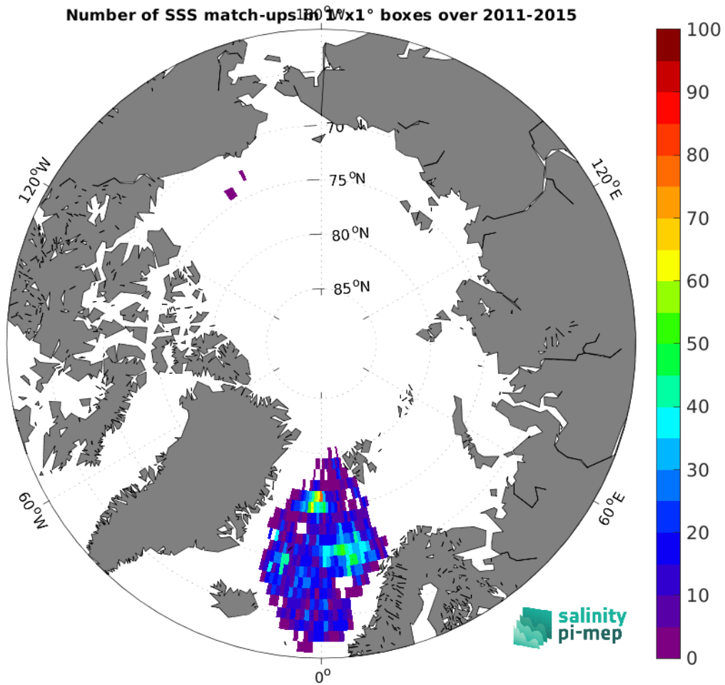
Figure 5: Number of SSS match-ups between Argo SSS and the Aquarius SSS L3 OR v5 - Monthly (NASA-GSFC) SSS product for the Arctic Ocean Pi-MEP region over 1^\circ \times 1^\circ boxes and for the full satellite product period.
