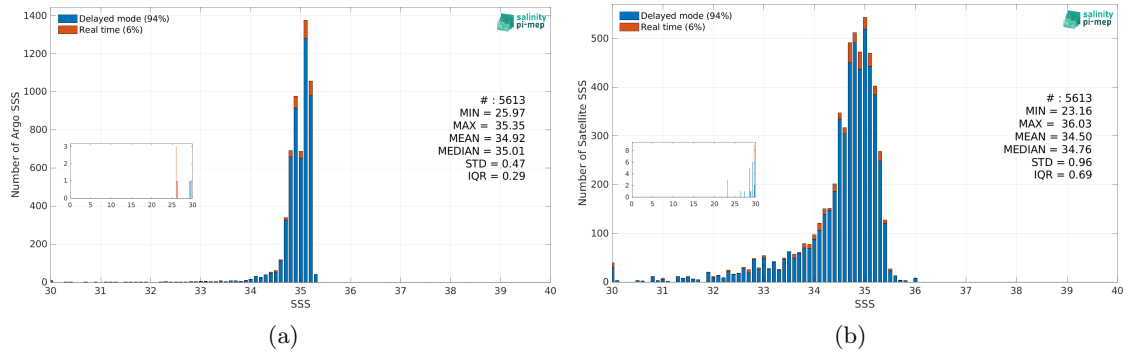
Figure 3: Histograms of SSS from Argo (a) and Aquarius SSS L3 OR v5 - Monthly (NASA-GSFC) (b) considering all match-up pairs per bins of 0.1 over the Arctic Ocean Pi-MEP region and for the full satellite product period.
